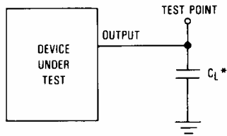
Figure 3. Test Circuit
