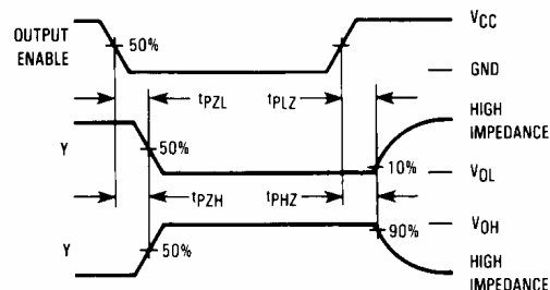
Figure 2. Switching Waveforms
