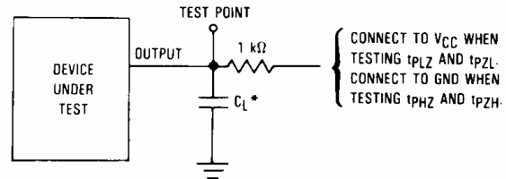
Figure 4. Test Circuit
