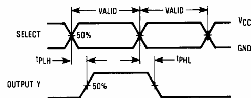
Figure 2. Switching Waveforms
