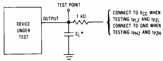
Figure 5. Test Circuit
