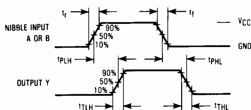
Figure 1. Switching Waveforms
