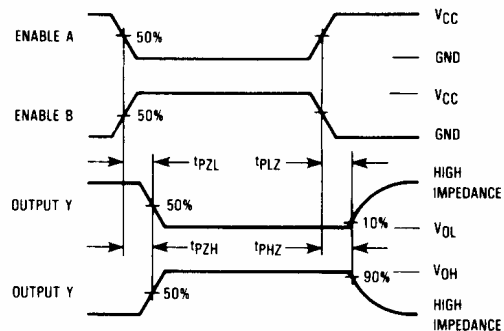
Figure 2. Switching Waveforms
