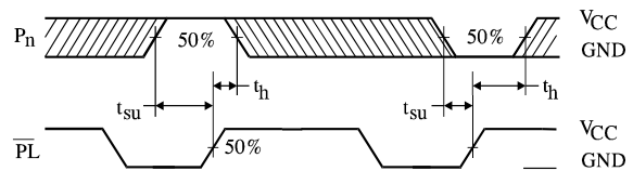
Figure 4. Switching Waveforms
