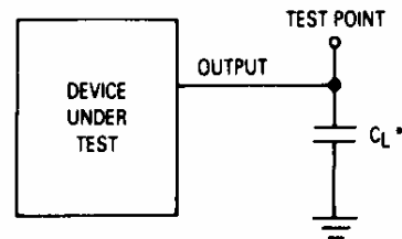
Figure 6. Test Circuit
