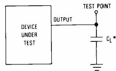
Figure 2. Test Circuit
