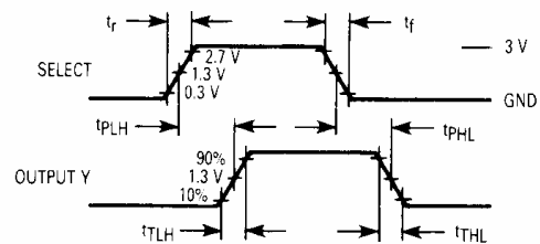
Figure 2. Switching Waveforms
