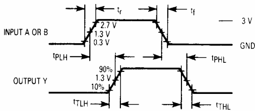
Figure 1. Switching Waveforms
