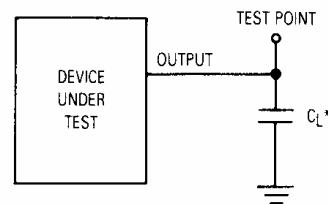
Figure 4. Test Circuit
