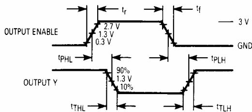
Figure 3. Switching Waveforms
