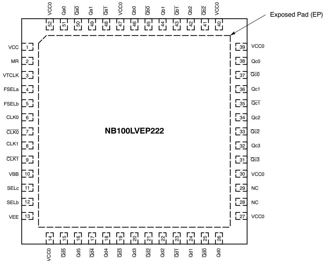
Figure 2. QFN-52 Pinout (Top View)
