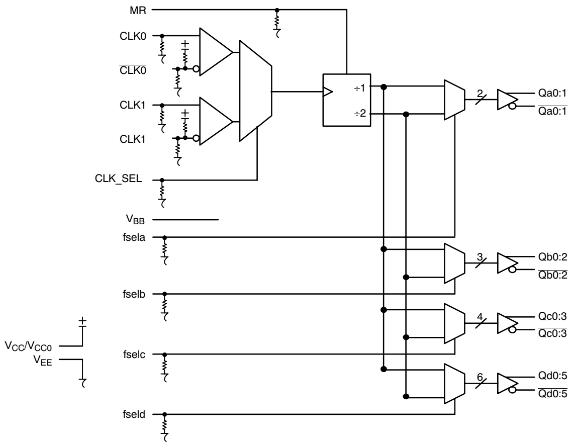
Figure 3. Logic Diagram
