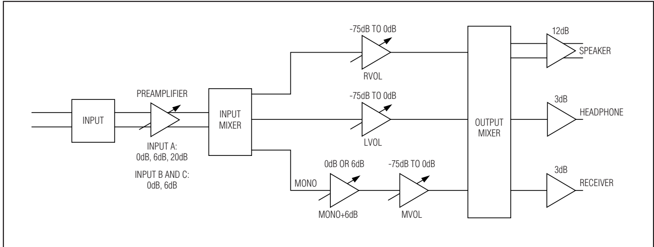
Figure 6. Signal Path
