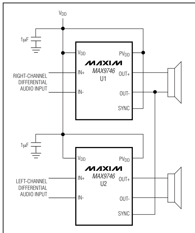
Figure 6. Master-Slave Stereo Configuration
