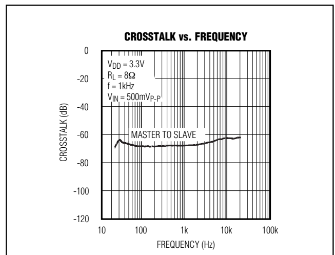
Figure 8. Master-Slave Crosstalk
