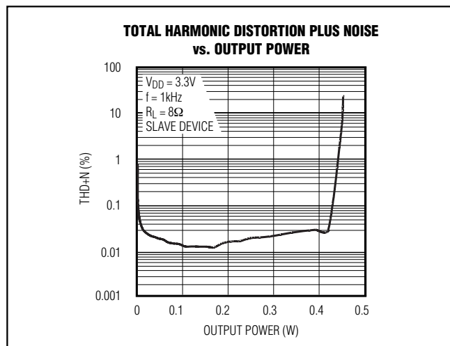
Figure 7. Master-Slave THD+N
