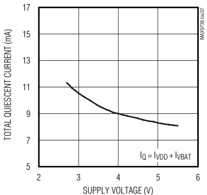
TOTAL QUIESCENT CURRENT vs. SUPPLY VOLTAGE
