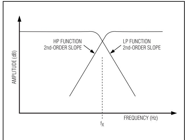
Figure 6. Crossover Frequency
