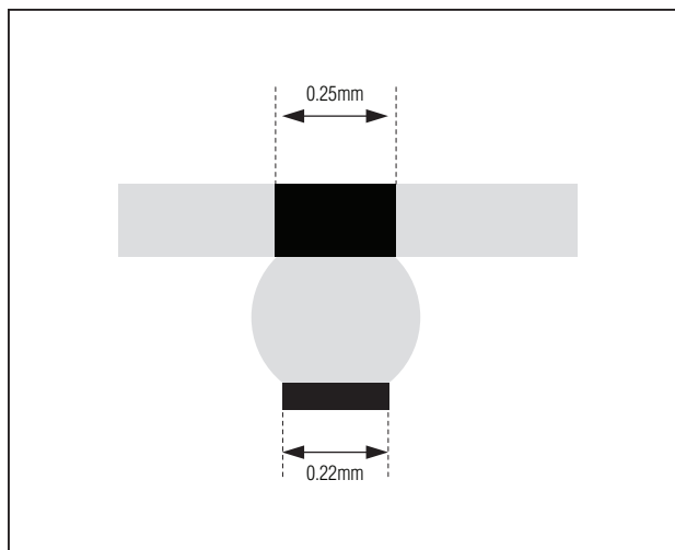
Figure 15. Recommended PCB Footprint
