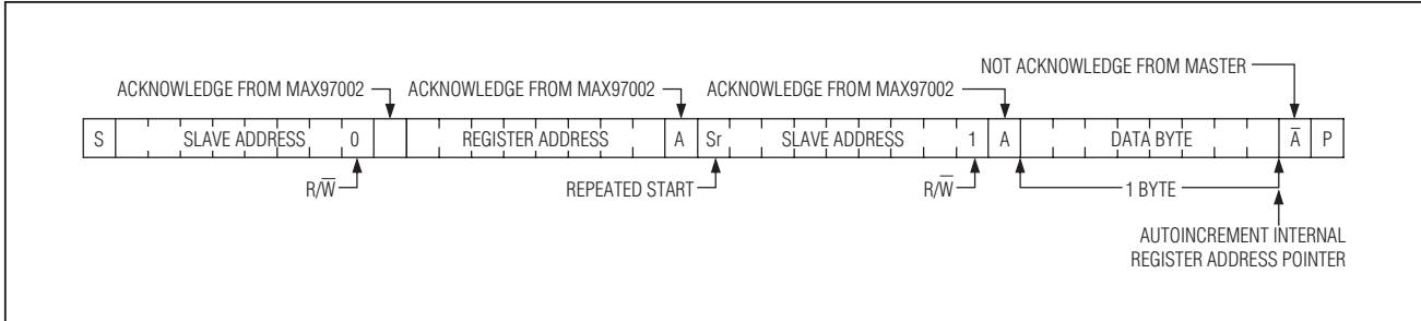
Figure 12. Reading One Byte of Data from the MAX97002
