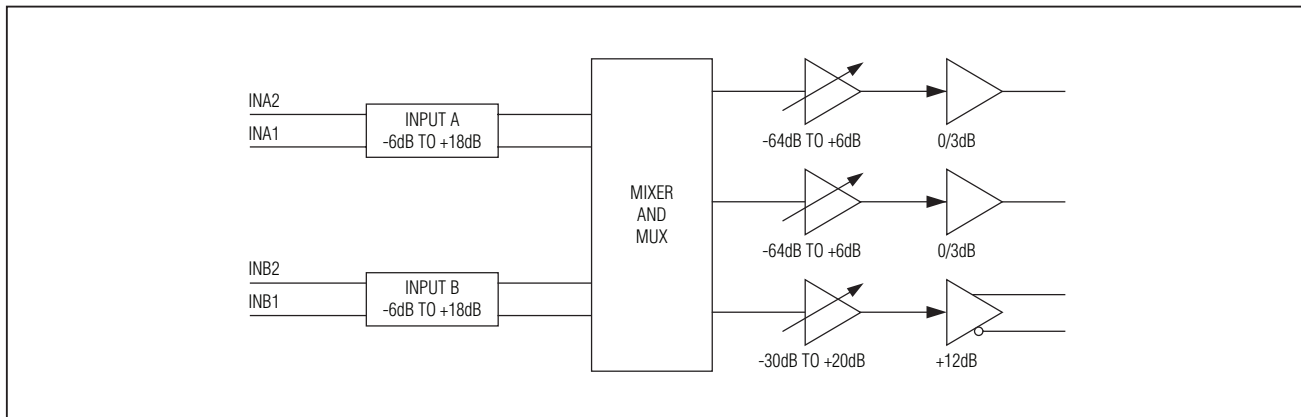
Figure 2. Signal Path
