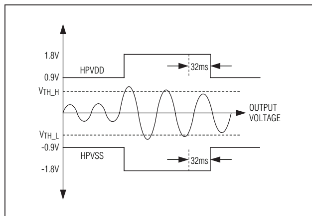
Figure 7. Class H Operation
