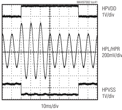
CLASS H OPERATION
