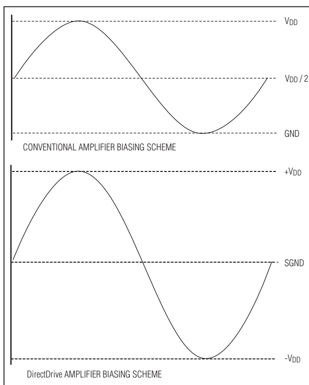
Figure 6. Traditional Amplifier Output vs. MAX97002 DirectDrive Output
