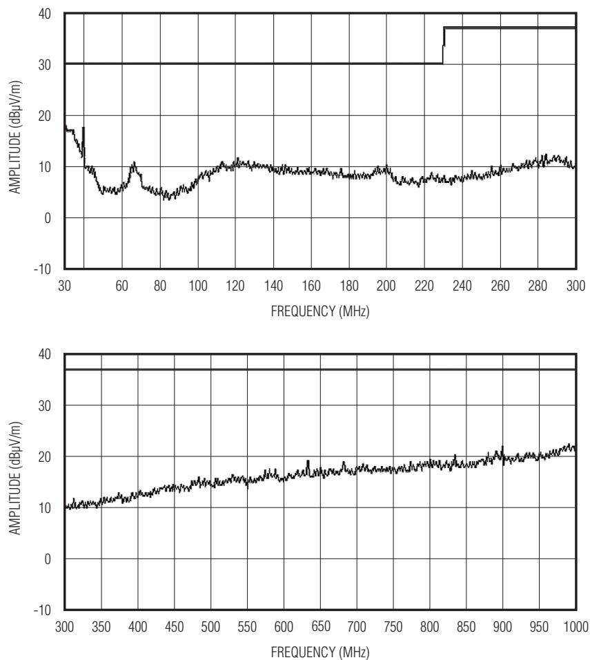
Figure 4. EMI with 15cm of Speaker Cable
