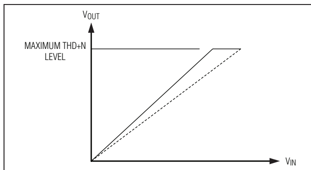
Figure 5. Limiter Gain Curve
