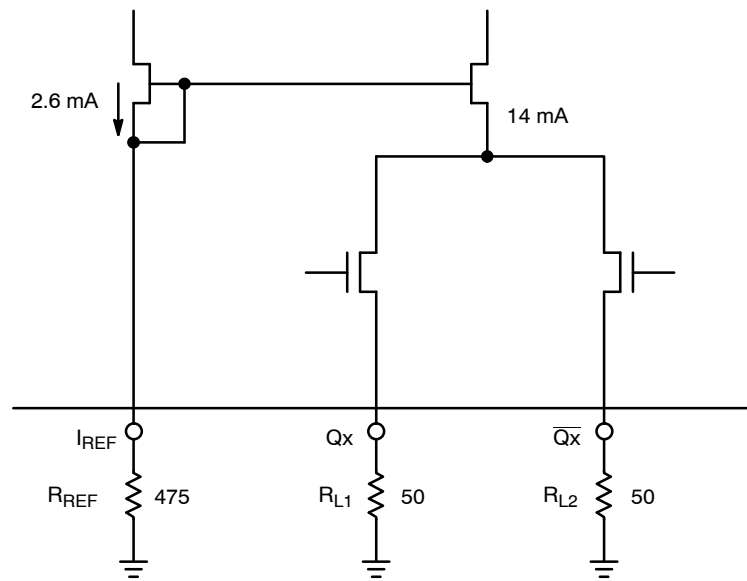
Figure 11. HCSL Simplified Output Structure
