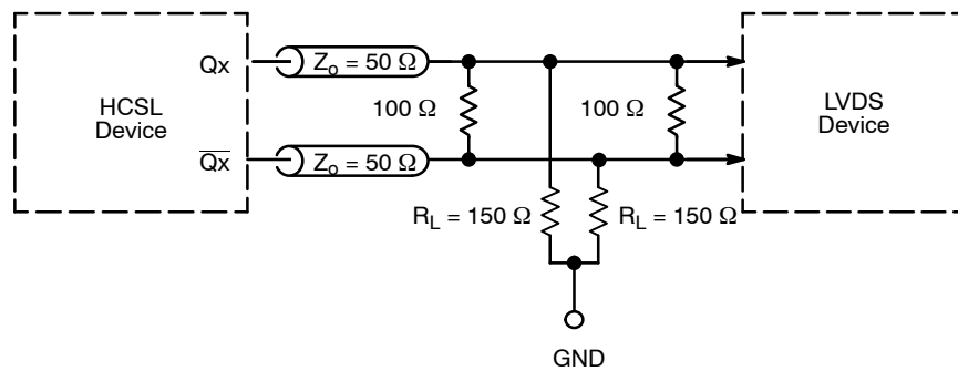
Figure 10. HCSL Interface Termination to LVDS
