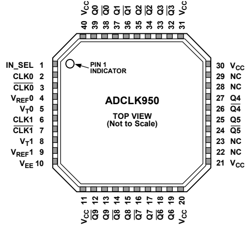
Figure 2. Pin Configuration
