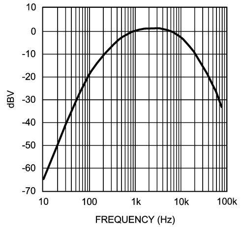
FIGURE 2. A-Weighted Filter
