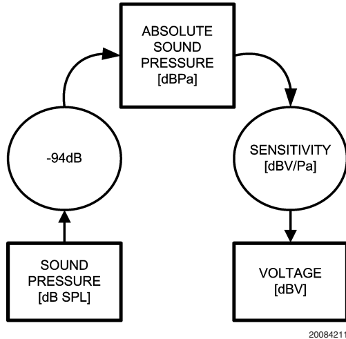
FIGURE 4. dB SPL to dBV Conversion
