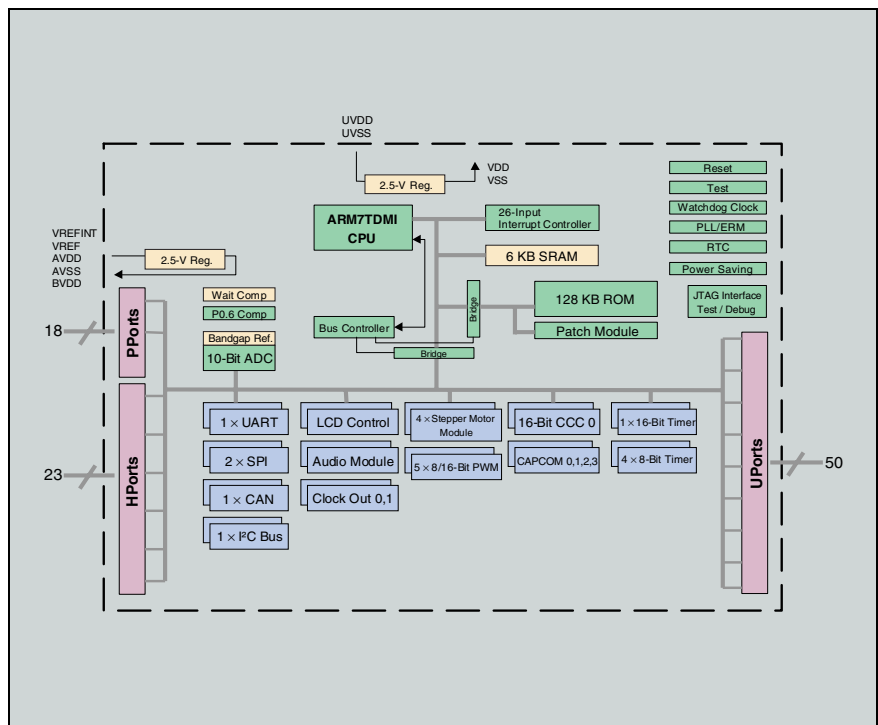
Fig. 2: Block diagram of the CDC 3231G
