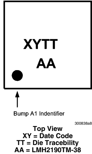
16-Bump micro SMD Marking
