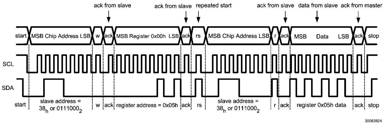
FIGURE 16. Example I 2 C Read Cycle
