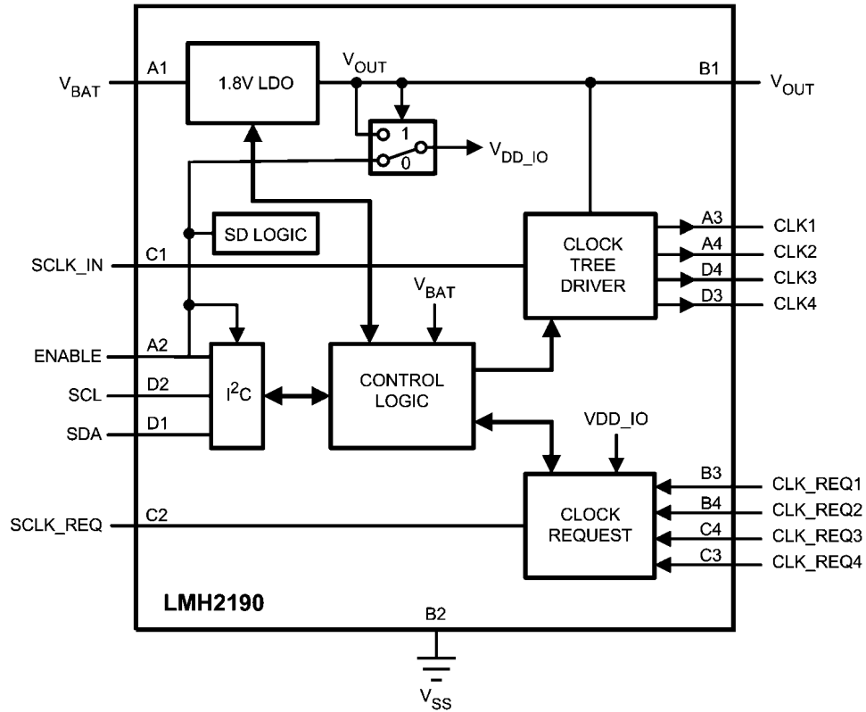
LMH2190
