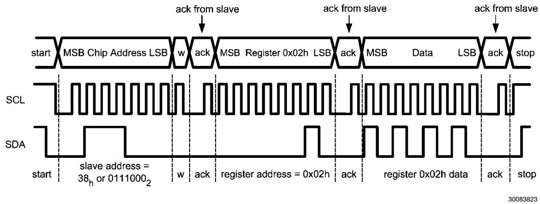
FIGURE 15. Example I 2 C Write Cycle
