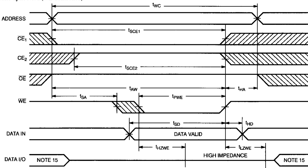
Write Cycle No. 1 ( \overline{WE} Controlled) [8, 13, 14]
