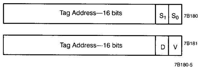
Figure 1. Cache Tag Entry Format
