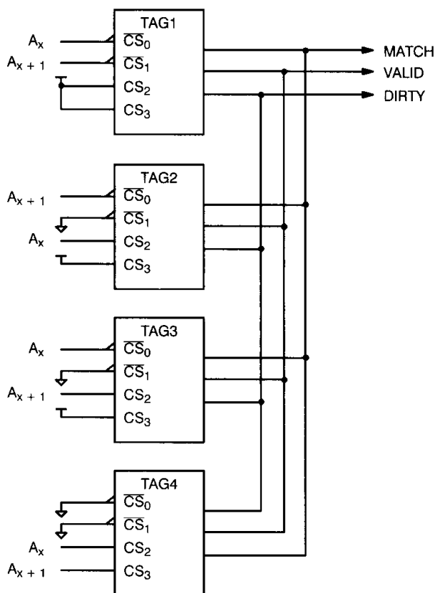
Figure 2. Cascading the CY7B180 and CY7B181
