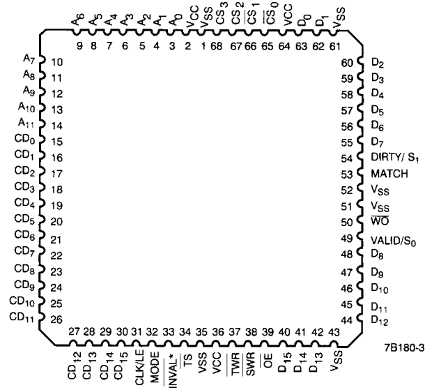
LCC & PLCC Top View
