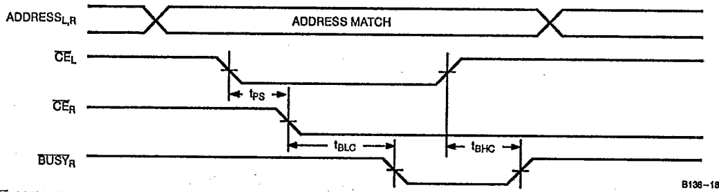
Busy Timing Diagram No. 1 ( \overline{CE} Arbitration) [30]
