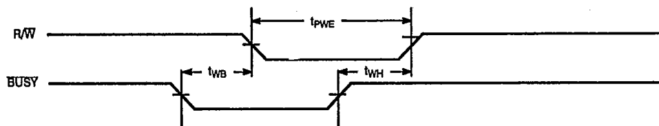
Write Timing with Busy Input ( M/\overline{S}=\text{LOW} )
