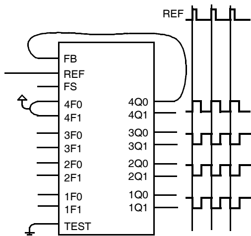
Figure 5. Inverted Output Connections
