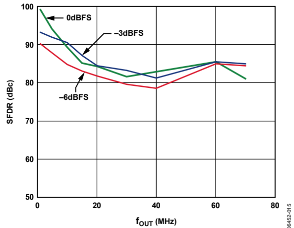
Figure 16. AD9779A In-Band SFDR vs. f_{OUT} , Digital Full-Scale
