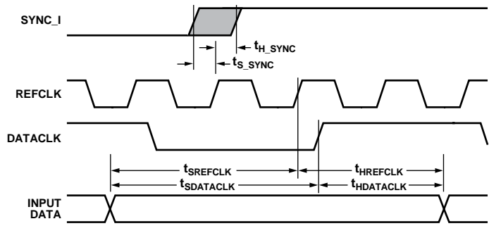
Figure 96. Timing Specifications, PLL Enabled or Disabled, Interpolation = 4x
