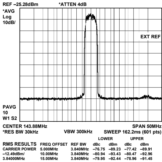
Figure 34. AD9779A WCDMA Signal, 4x Interpolation, f_{DATA} = 122.88 MSPS, f_{DAC}/4 Modulation
