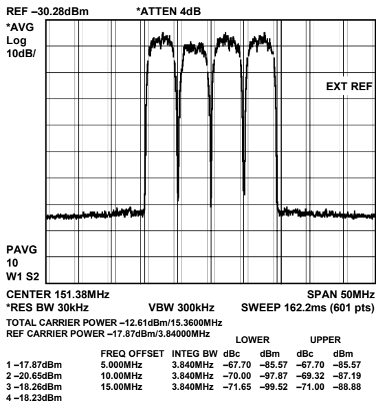
Figure 35. AD9779A Multicarrier WCDMA Signal, 4x Interpolation, f_{DAC} = 122.88 MSPS, f_{DAC}/4 Modulation
