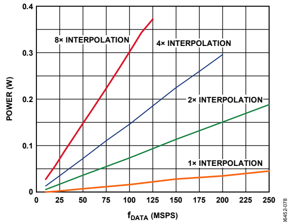
Figure 84. Power Dissipation, Digital 1.8 V Supply, I Data Only, Real Mode, Does Not Include Zero Stuffing
