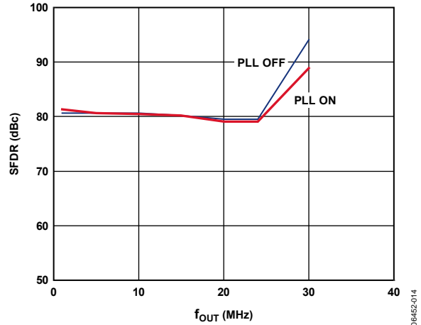
Figure 15. AD9779A In-Band SFDR, 4x Interpolation, f_{DATA} = 100 MSPS, PLL On/Off
