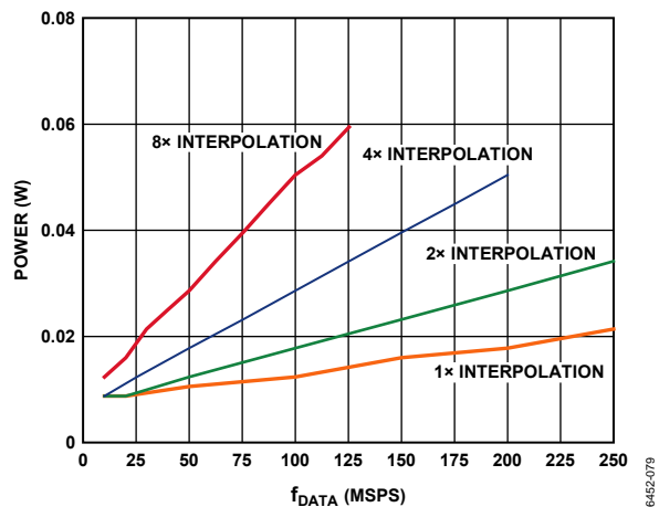
Figure 85. Power Dissipation, Clock 1.8 V Supply, I Data Only, Real Mode, Includes Modulation Modes, Does Not Include Zero Stuffing
