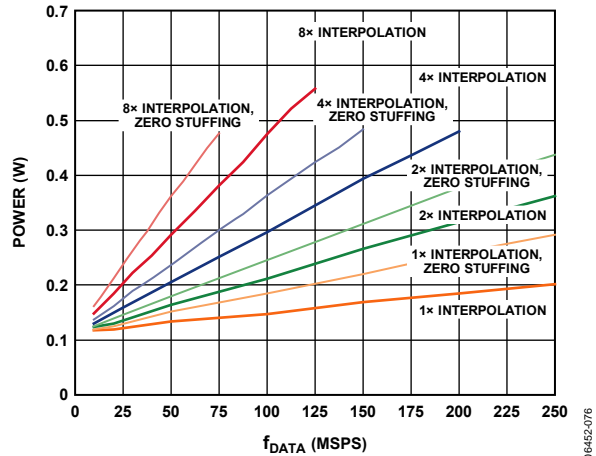
Figure 83. Total Power Dissipation, I Data Only, Real Mode
