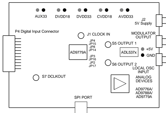
Figure 103. AD9776A/AD9778A/AD9779A Evaluation Board Showing All Connections
