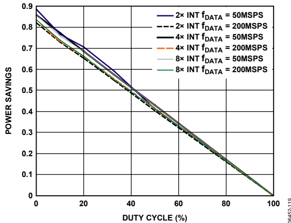
Figure 92. Power Savings Based on Duty Cycle of TXENABLE
