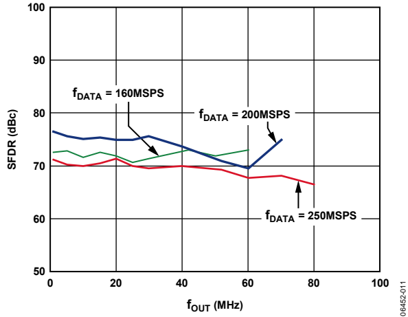
Figure 12. AD9779A Out-of-Band SFDR vs. f_{OUT} , 2x Interpolation
