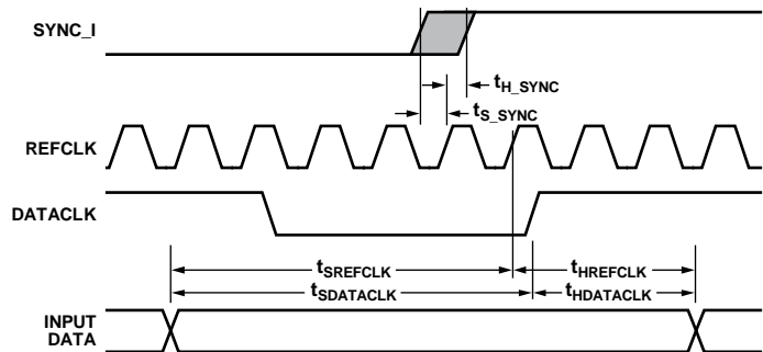
Figure 97. Timing Specifications, PLL Enabled or Disabled, Interpolation = 8x
