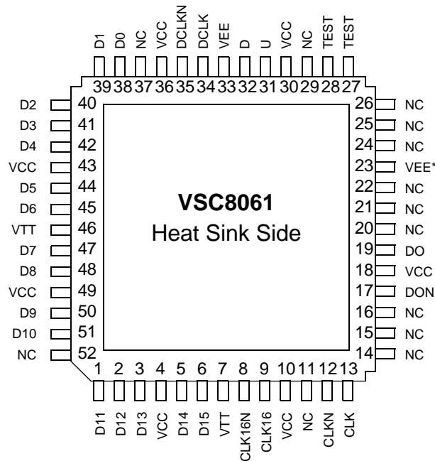
Figure 9: VSC8061/8062 F (52-Pin LDCC) Pin Diagrams
