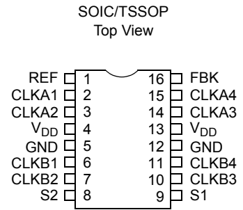
Pin Configuration
