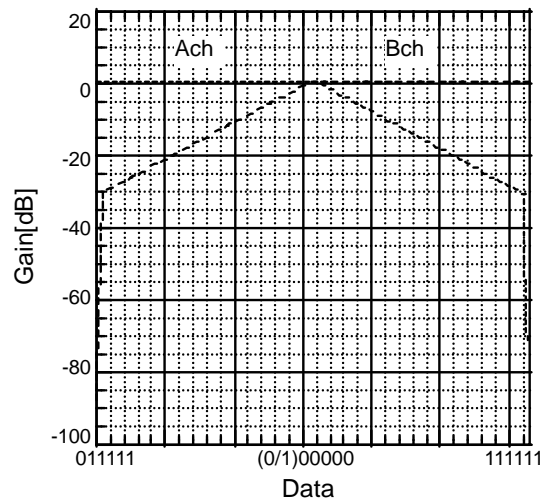
Balance Control V_{in}=1\text{Vrms}/1\text{kHz}
