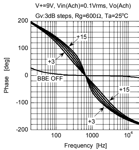
Phase vs Frequency (BBE)
