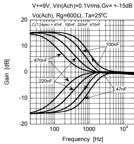
Gain vs Frequency (TONE)
