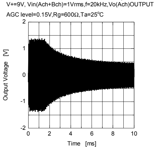
AGC Attack Time (C:9pin=1 μF)
