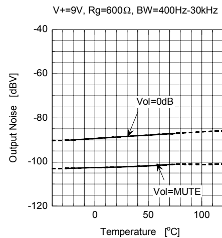
Output Noise vs Temperature
