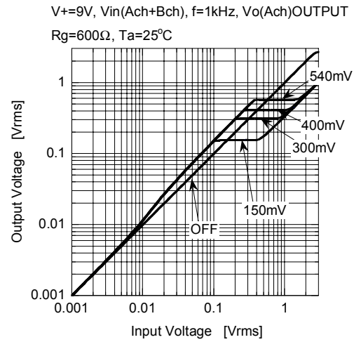
AGC Control
