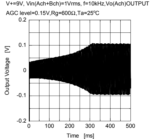
AGC Recovery Time (C:9pin=1 μF)
