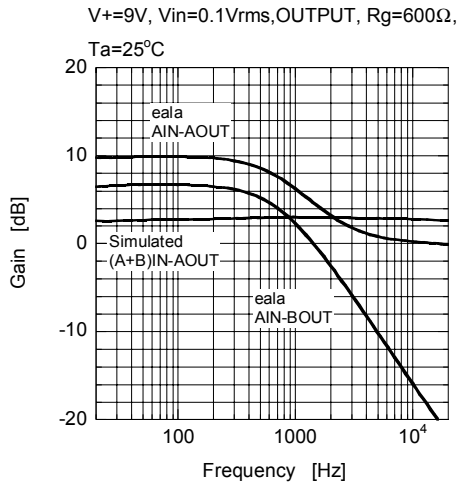
Gain vs Frequency (eala&Simulated)
