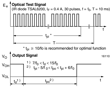
Figure 1. Output Function
