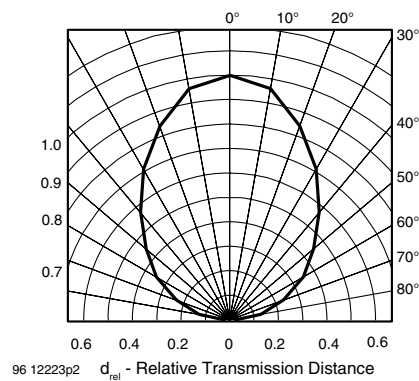
Figure 12. Directivity
