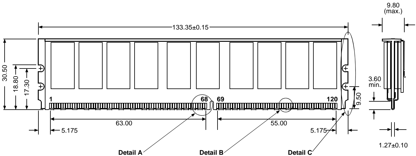
Front View
