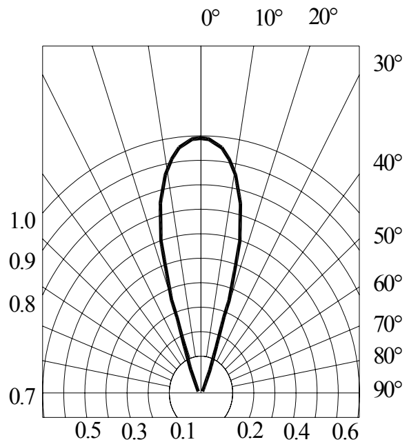
RADIATION DIAGRAM
