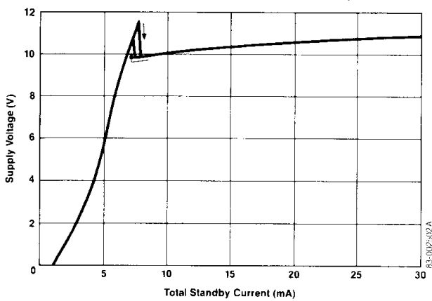
Total Standby Current vs. Supply Voltage
