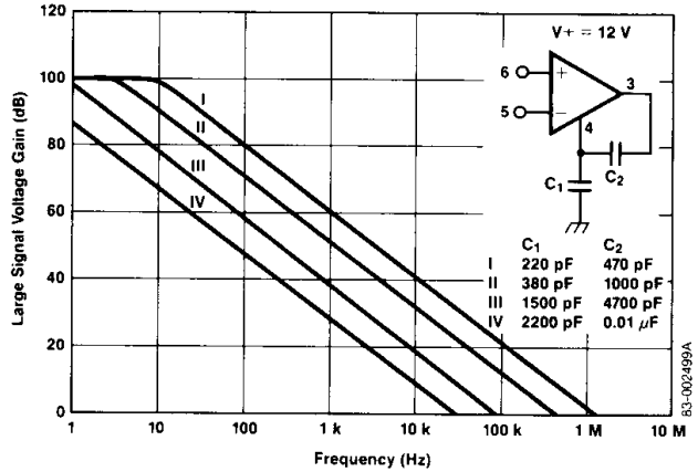
Error Amplifier II, A_{V2} vs. Frequency
