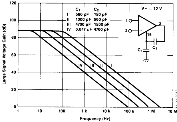
Error Amplifier I, A_{V1} vs. Frequency
