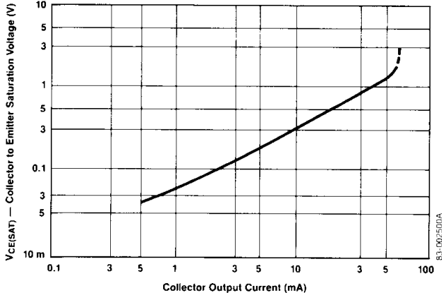
Correct Saturation Voltage vs. Collector Current
