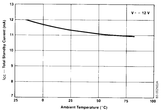
Total Standby Current vs. Ambient Temperature
