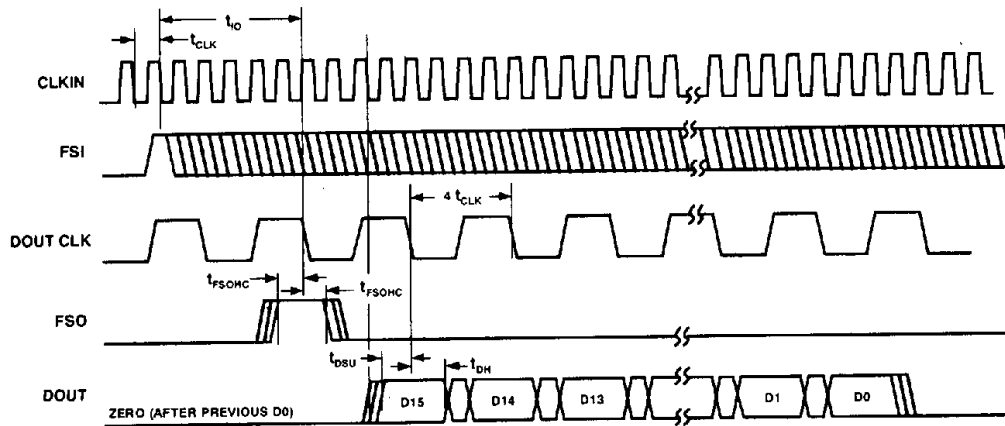
Figure 14a. Mode A Timing
