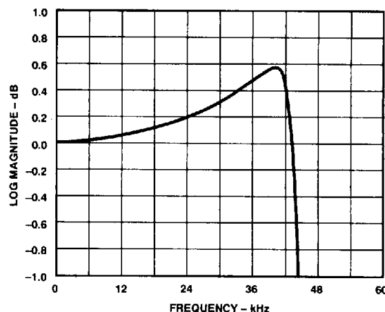
Figure 6. FIR Filter, Compensation Function
