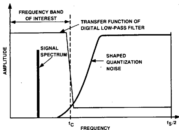
Figure 2. Noise Shaping
