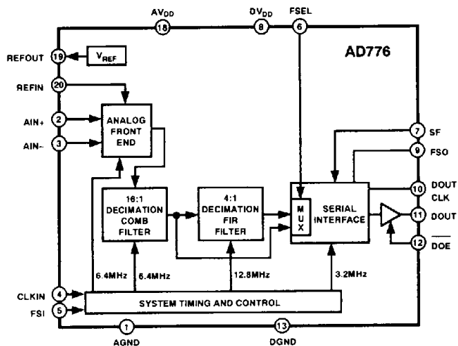
Figure 3. Block Diagram
