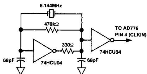
Figure 12. Basic Clock Circuit
