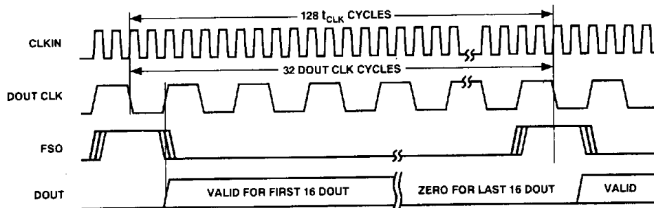
Figure 14b. Mode A Timing
