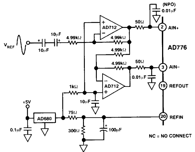
Figure 9. Single-Ended Input to Differential Circuit
