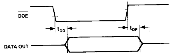
Figure 18. Data Output Timing
