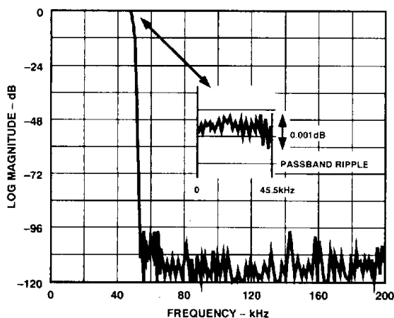
Figure 5. FIR Filter, Low-Pass Response
