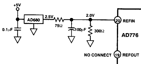
Figure 11. External Voltage Reference Circuit
