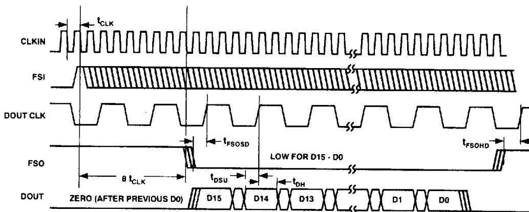
Figure 15a. Mode B Timing
