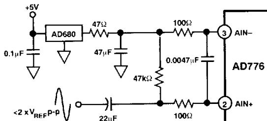
Figure 8. Single-Ended Input Circuit for Improved PSRR
