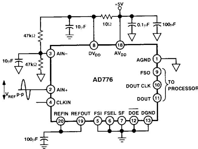
Figure 7. Simple Single-Ended Input Circuit
