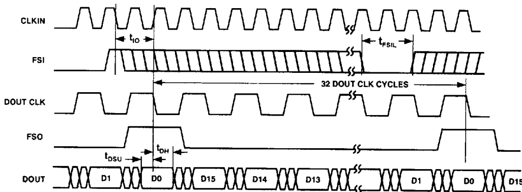
Figure 16. Mode C Timing
