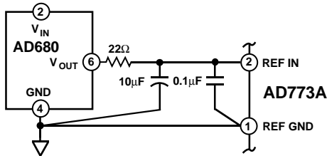
Figure 11. Recommended AD773A to AD680 Connection
