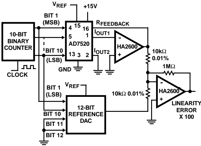
FIGURE 2. NONLINEARITY
