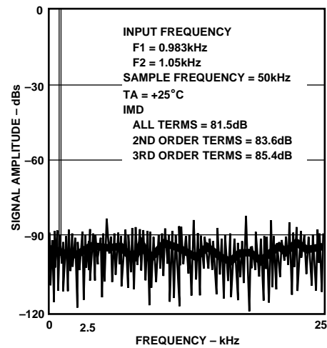
Figure 12. IMD Plot
