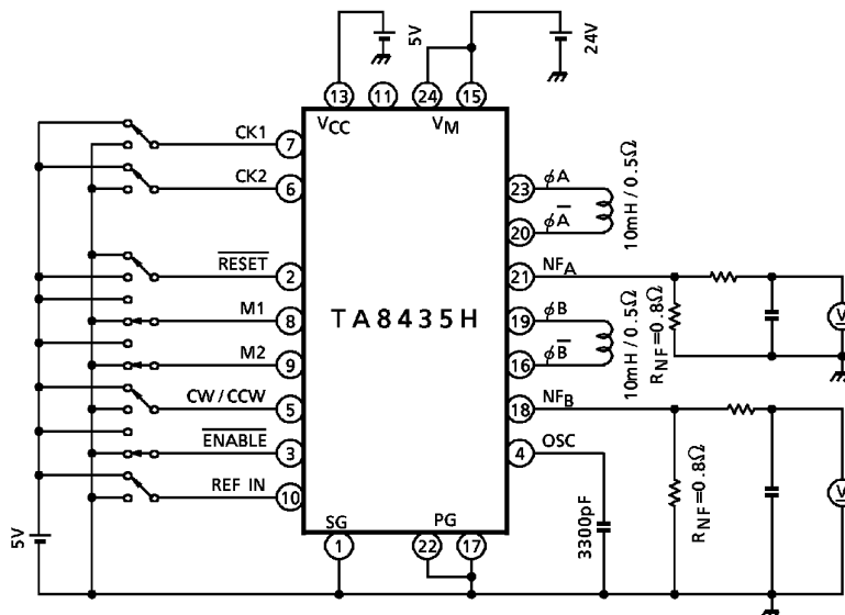
TEST CIRCUIT 4 V_{CE(SAT)} UPPER SIDE, LOWER SIDE
