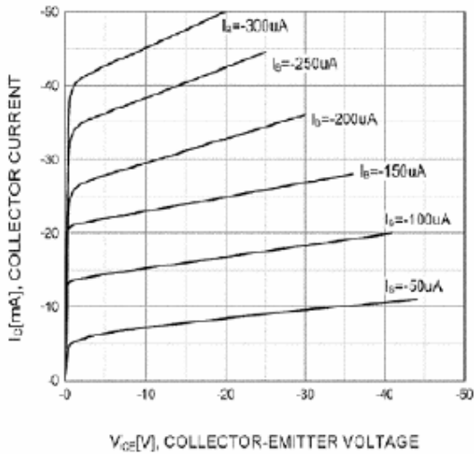
Static Characteristic
