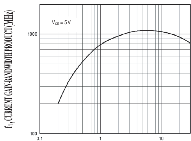
FIG4. Current Gain Bandwidth Product
