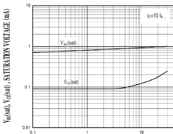
FIG3. Base-Emitter Saturation Voltage Collector-Emitter Saturation Voltage
