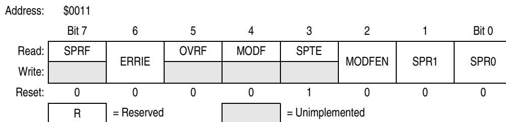
Figure 17-13. SPI Status and Control Register (SPSCR)
