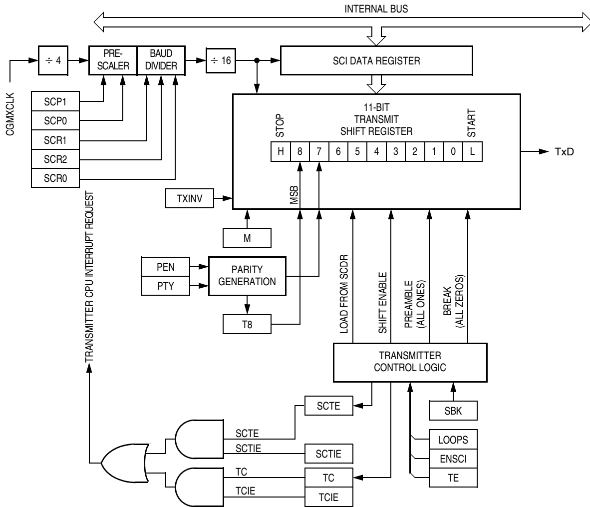
Figure 16-4. SCI Transmitter
