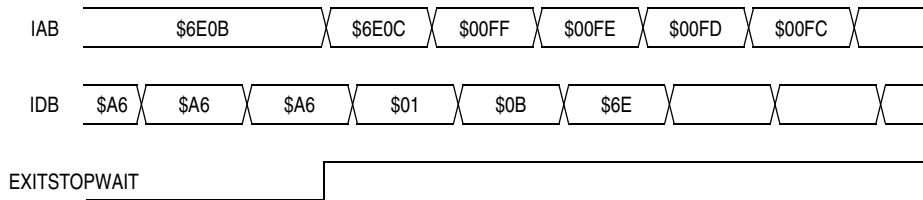
Figure 7-12. Wait Mode Entry Timing
