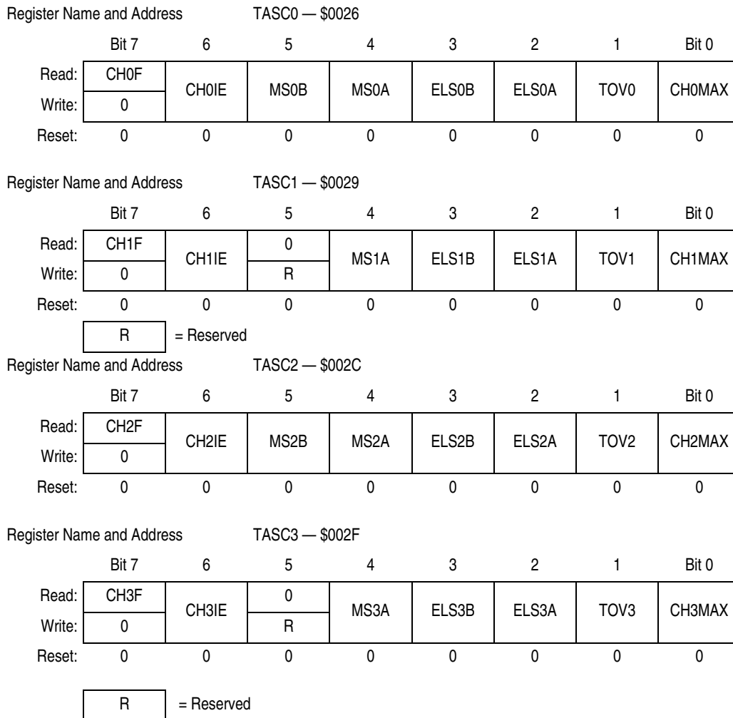
Figure 18-7. TIMA Channel Status and Control Registers (TASC0–TASC5)
