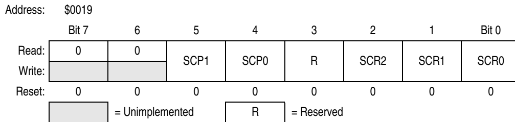
Figure 16-18. SCI Baud Rate Register (SCBR)
