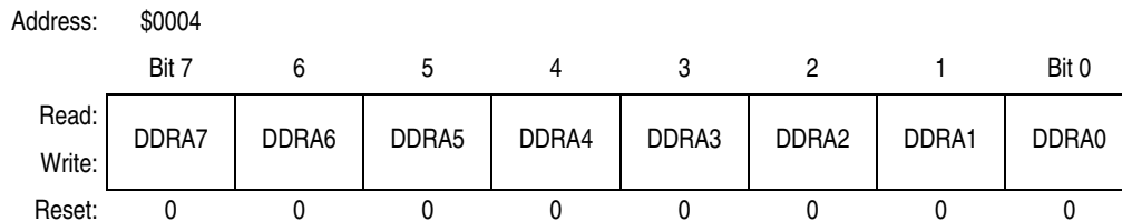
Figure 23-3. Data Direction Register A (DDRA)
