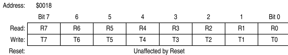
Figure 16-17. SCI Data Register (SCDR)
