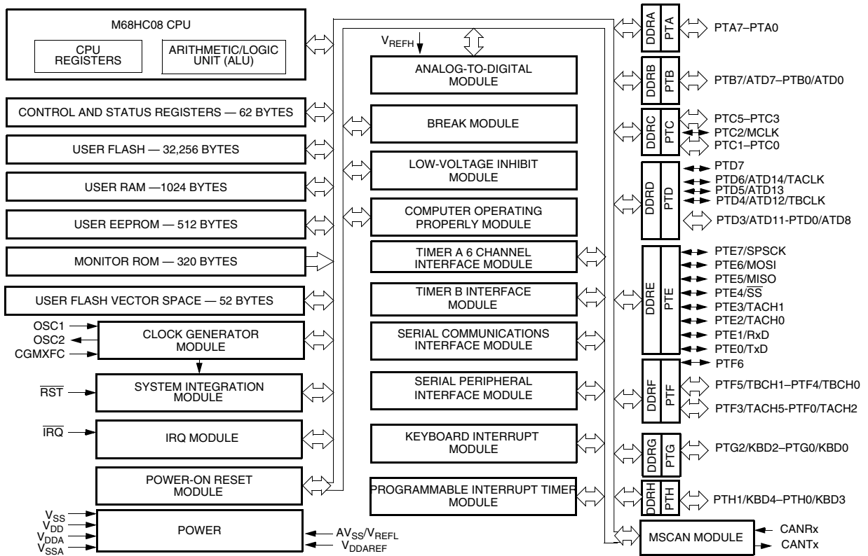
Figure 1-1. MCU Block Diagram for the MC68HC908AZ32A
