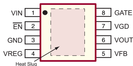
8-Lead SOIC w/ Heat Slug (SG) (top view)
