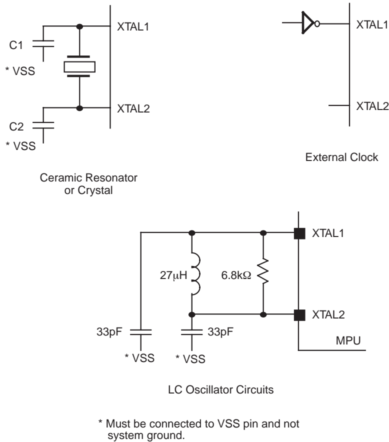
Figure 20. Oscillator Configuration
