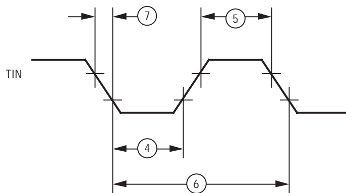
Figure 5. Counter Timer
