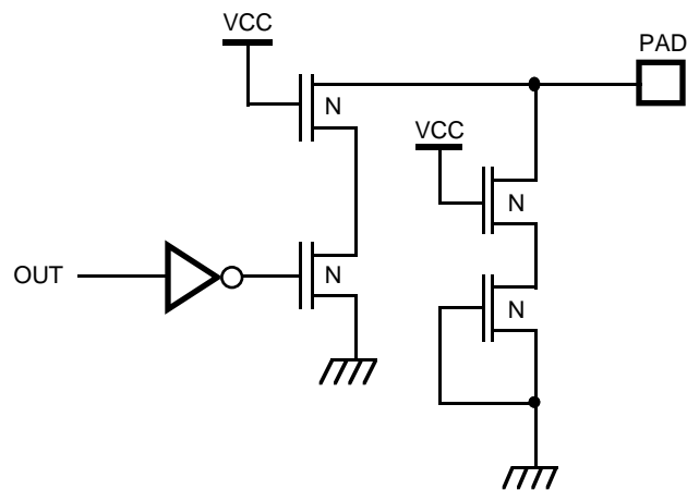
Figure 28. Output Only, 12-Volt Open-Drain (Pad Type 7)
