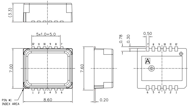
Figure 3. Housing dimensions
