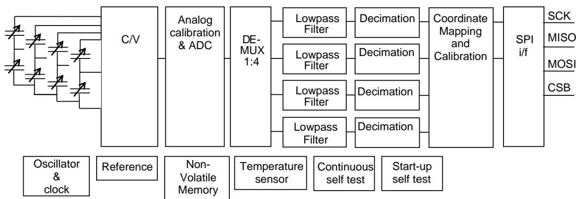
Figure 1. SCA2100-D01 Block diagram
