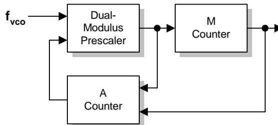
Figure 3: Feedback Divider
