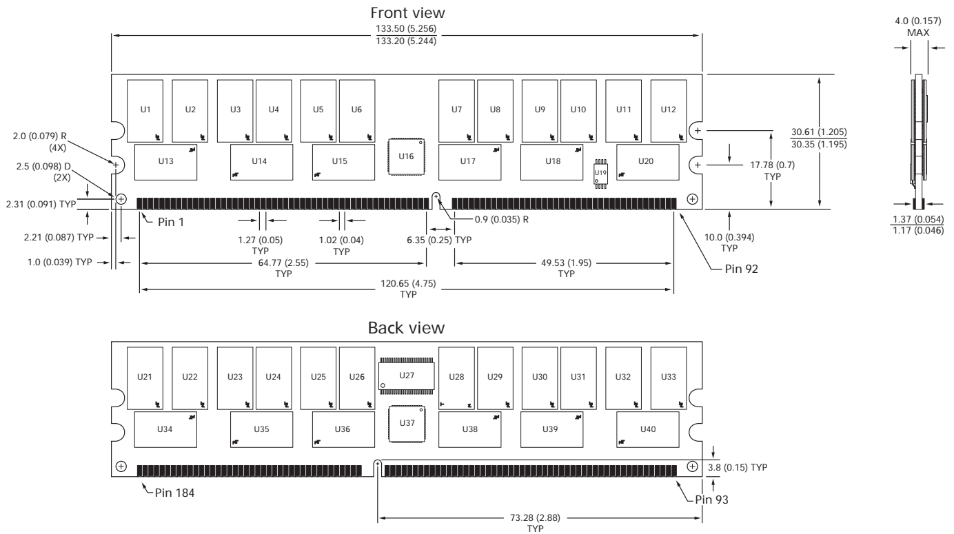
Figure 8: 184-Pin RDIMM – Standard-Height Layout (1GB)
