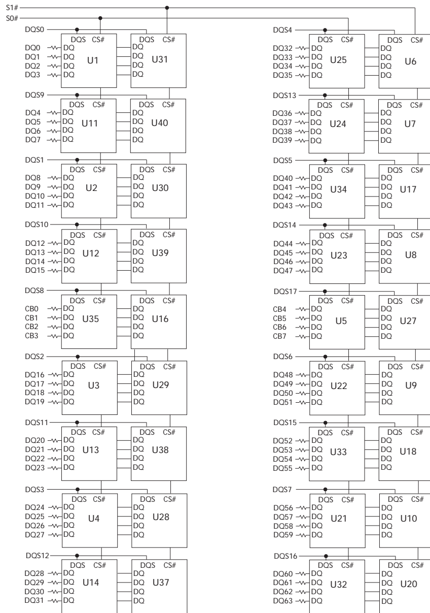
Figure 6: Functional Block Diagram – Standard-Height Layout (2GB)
