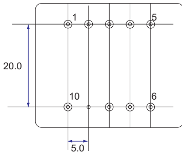
Pin view (underneath)
