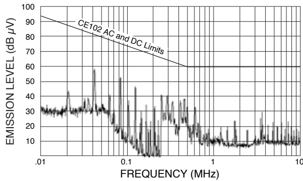
CE102: Three paralleled and synchronized MFL28 converters with an FMCE-0828.
