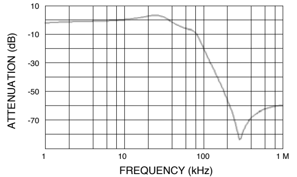
FMCE-0828 Attenuation
