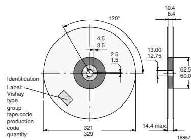
Figure 10. Reel Dimensions - GS18
