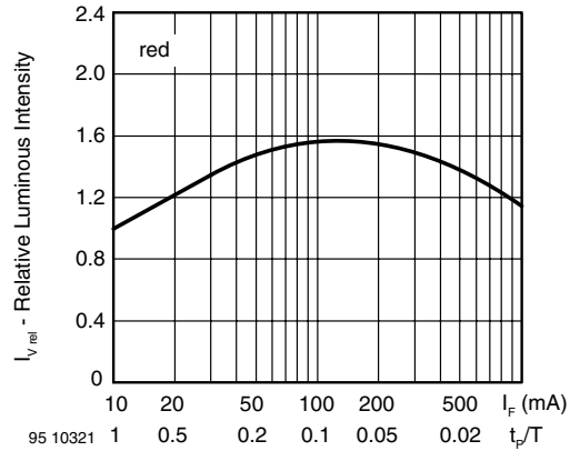
Figure 5. Rel. Lumin. Intensity vs. Forw. Current/Duty Cycle
