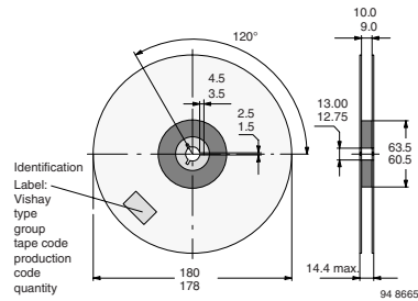
Figure 9. Reel Dimensions - GS08
