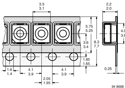
Figure 8. Tape Dimensions in mm for PLCC-2
