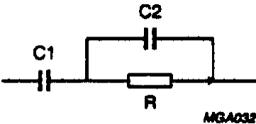
Fig.6 Loop filter
