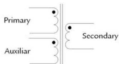
FLYBACK
