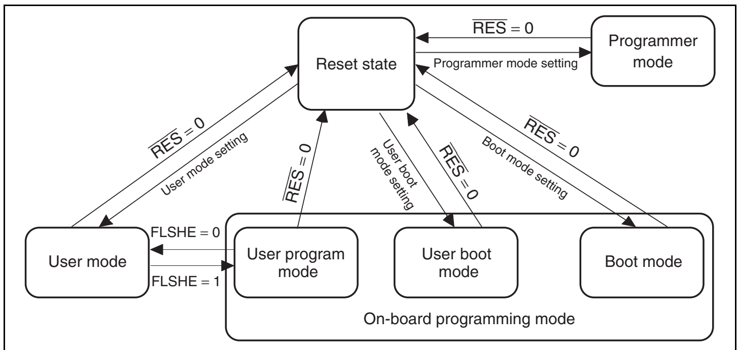
Figure 19.2 Mode Transition for Flash Memory
