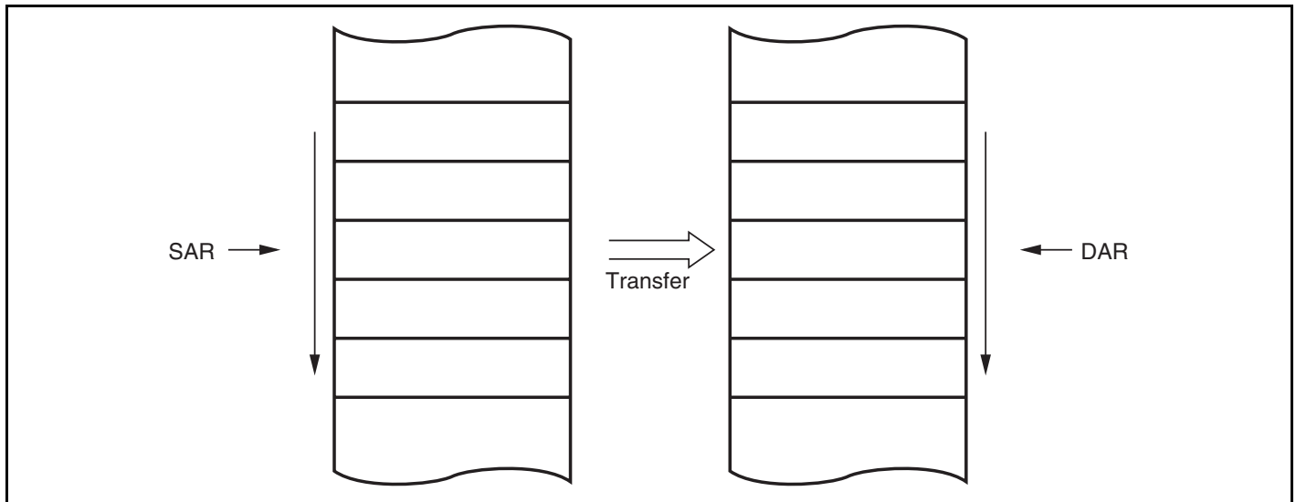
Figure 7.5 Memory Mapping in Normal Mode
