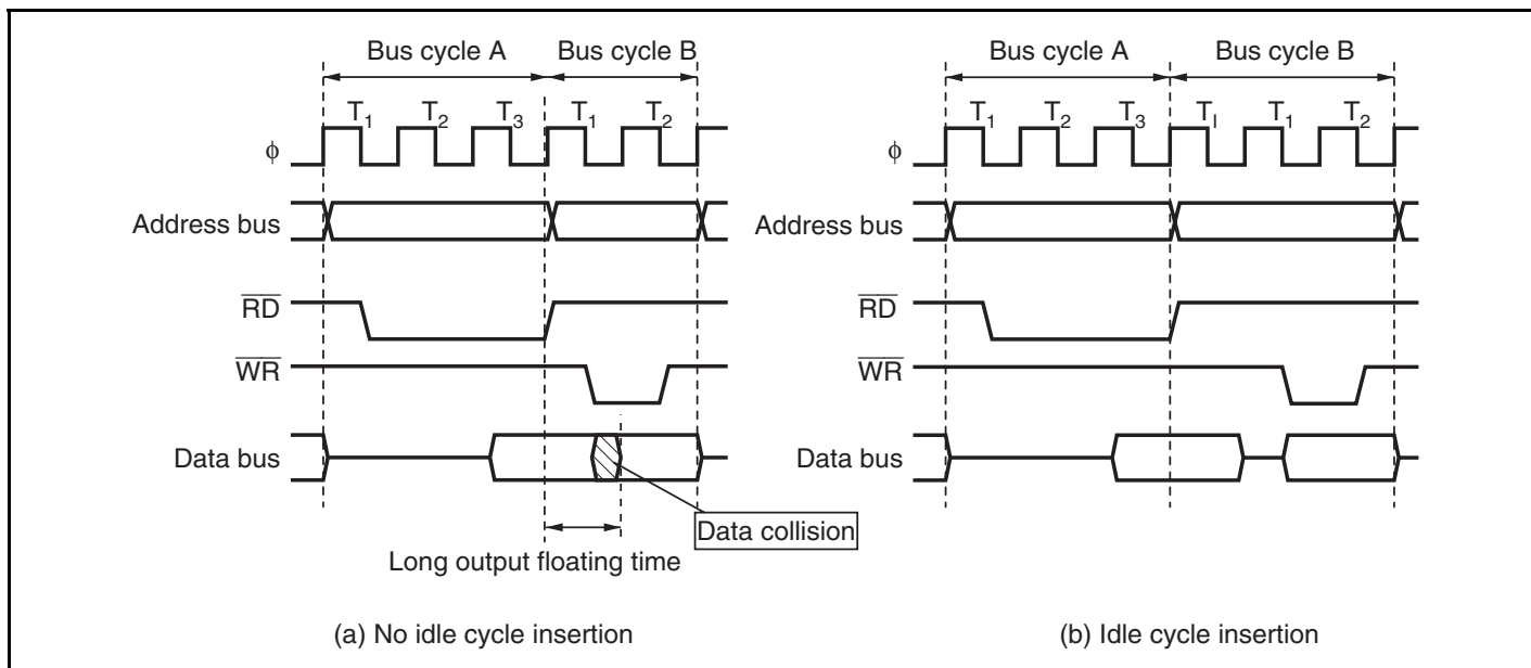
Figure 6.10 Examples of Idle Cycle Operation
