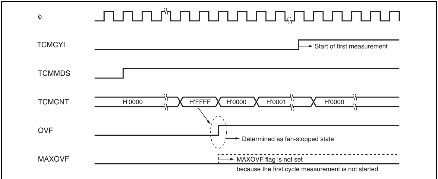
Figure 12.9 Example of Timing in Fan-Stopped State (1)
