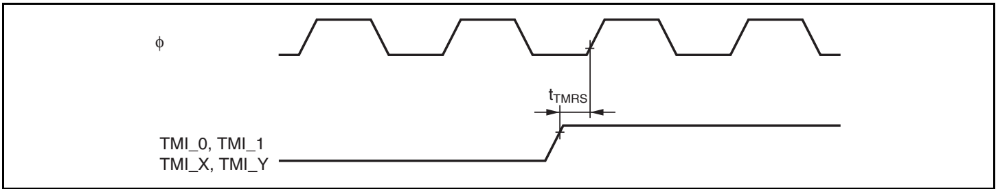
Figure 24.21 8-Bit Timer Reset Input Timing
