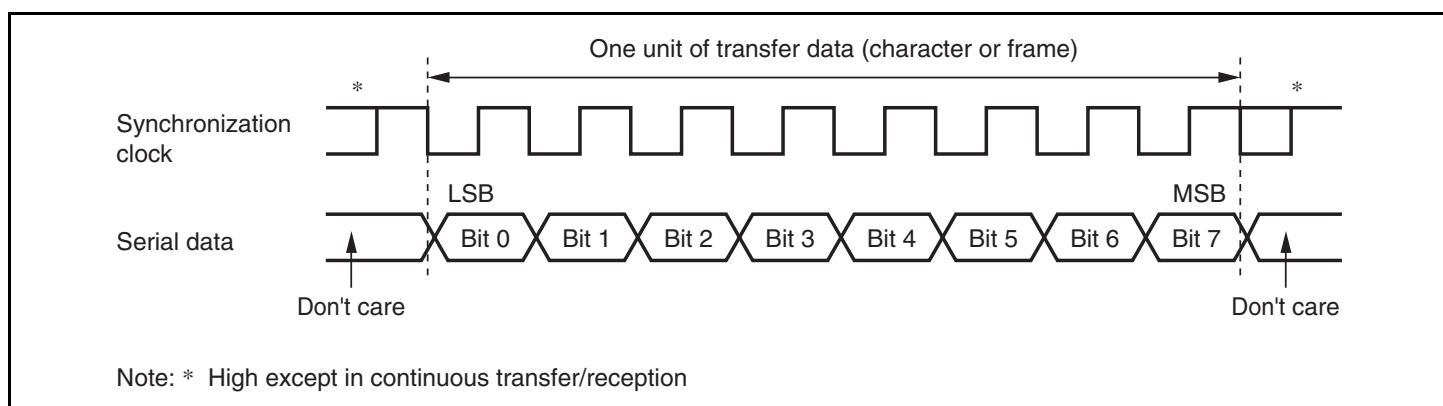
Figure 15.14 Data Format in Clocked Synchronous Communication (LSB-First)
