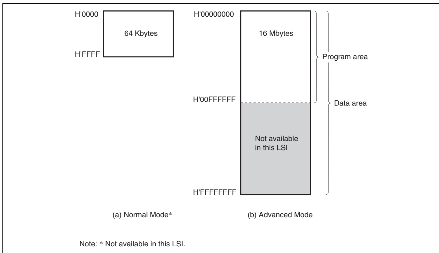
Figure 2.5 Memory Map
