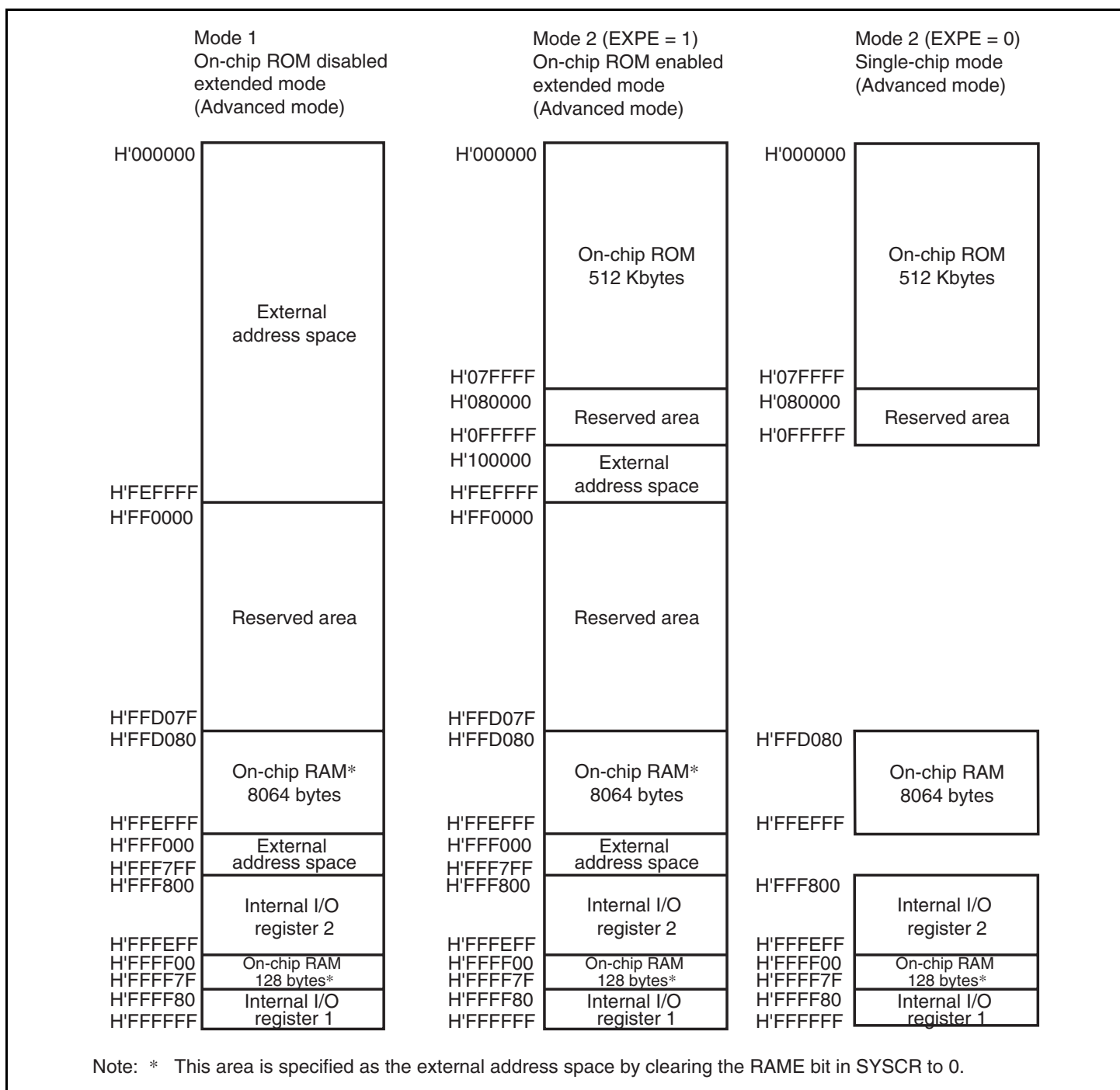
Figure 3.1 Address Map (1)
