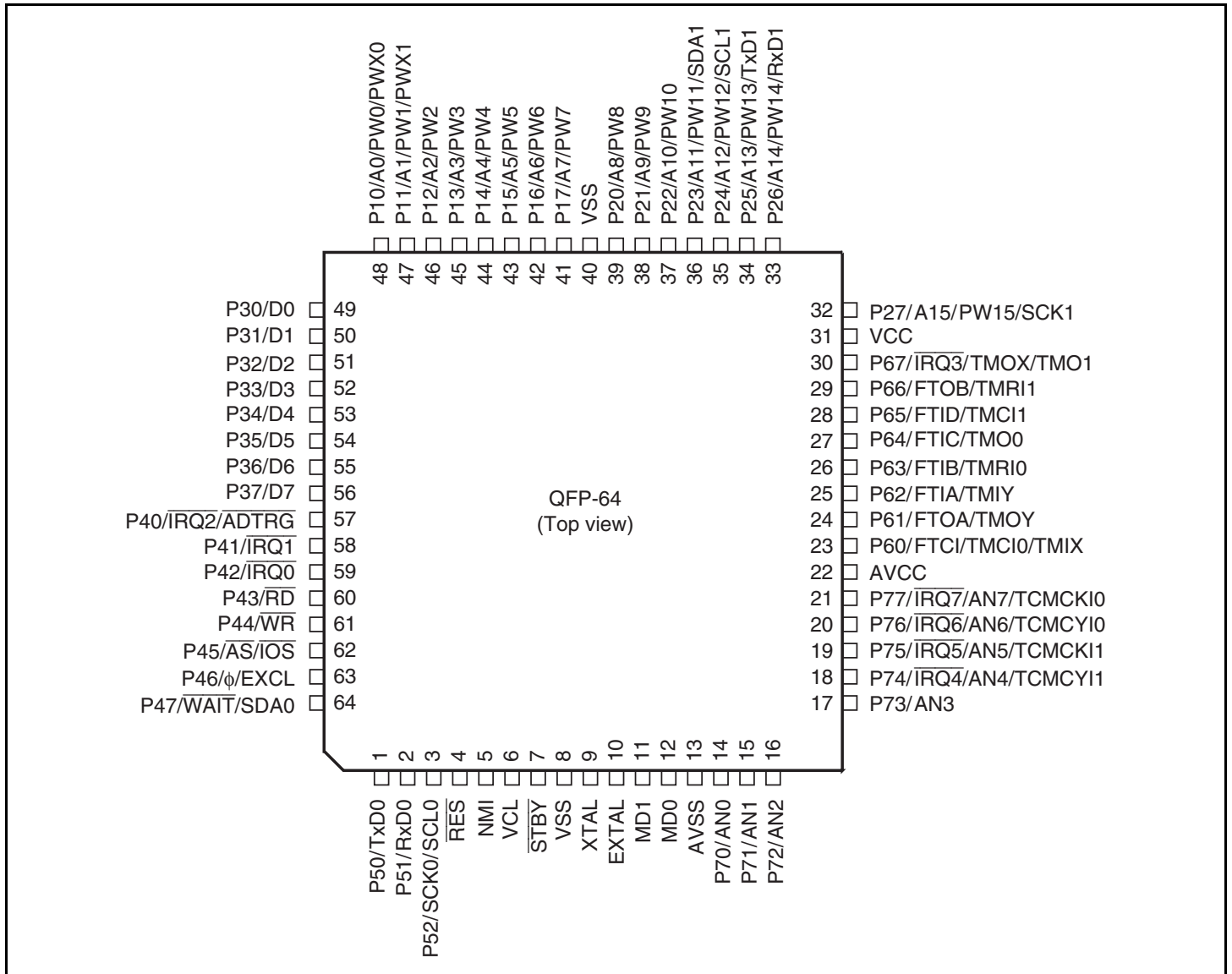
Figure 1.3 Pin Assignments (QFP-64)
