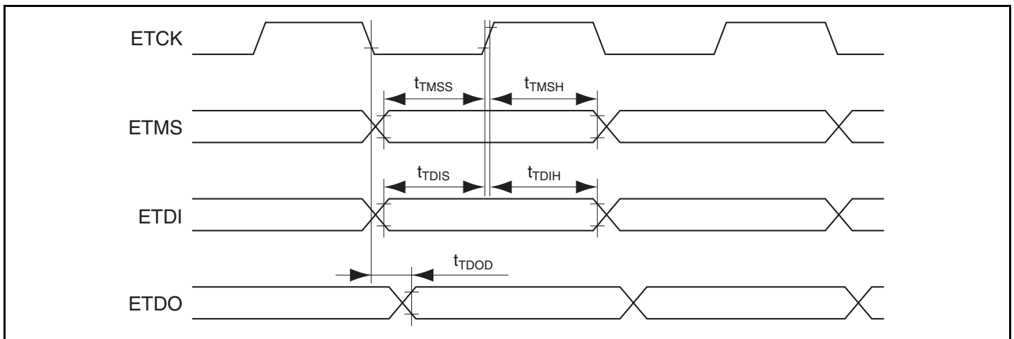
Figure 24.29 H-UDI Input/Output Timing
