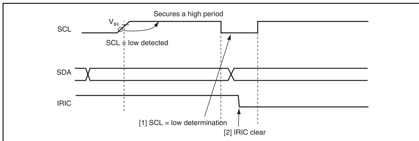
Figure 16.32 IRIC Flag Clearing Timing When WAIT = 1
