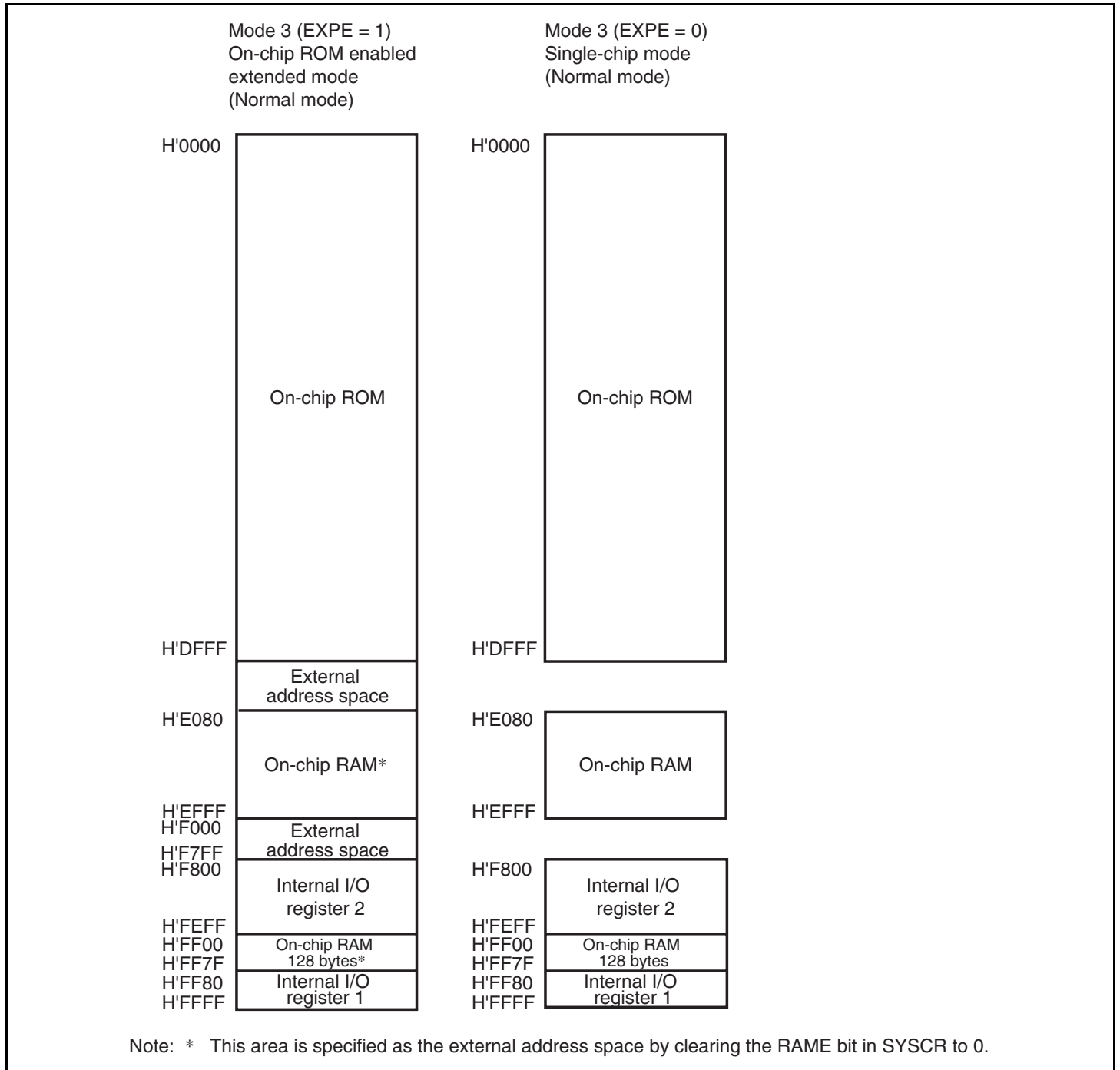
Figure 3.2 Address Map (2)
