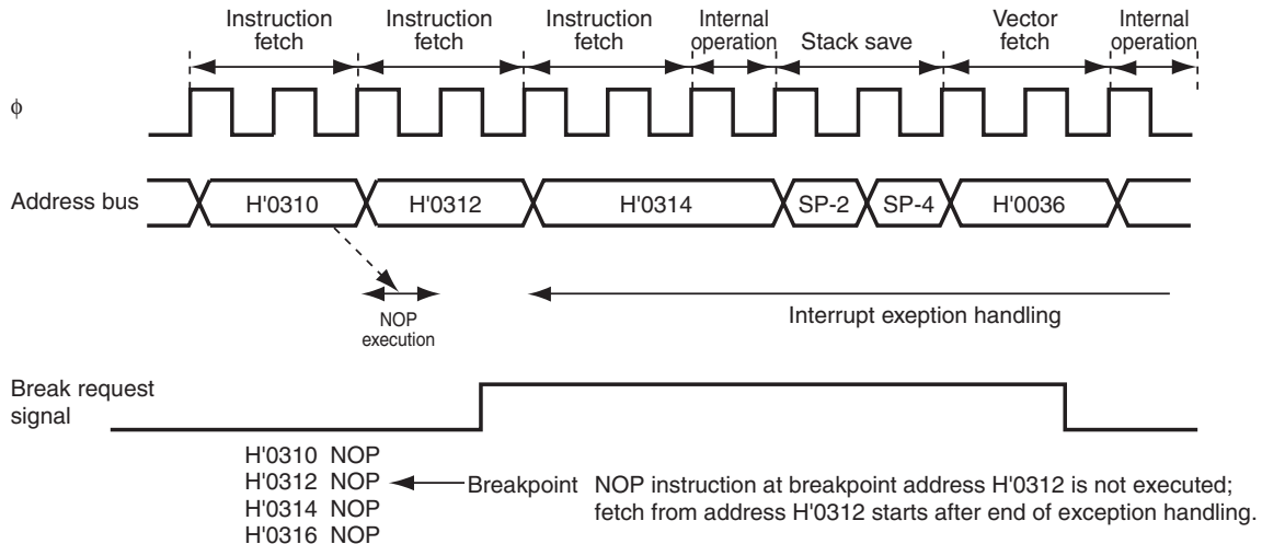
Figure 5.10 Examples of Address Break Timing
