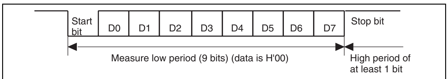
Figure 19.7 Automatic-Bit-Rate Adjustment Operation of SCI
