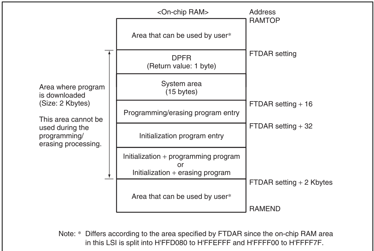
Figure 19.10 RAM Map when Programming/Erasing is Executed
