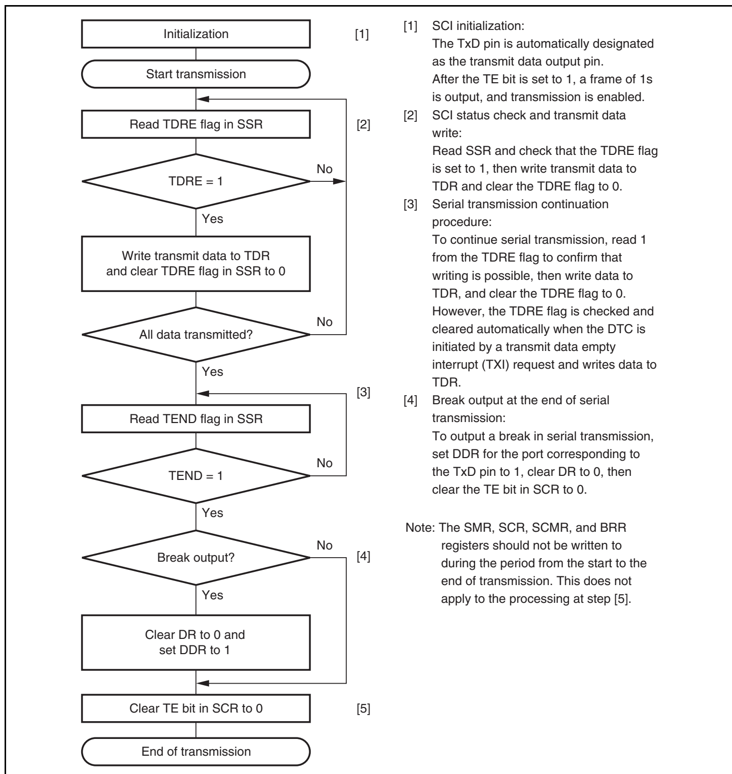
Figure 15.7 Sample Serial Transmission Flowchart
