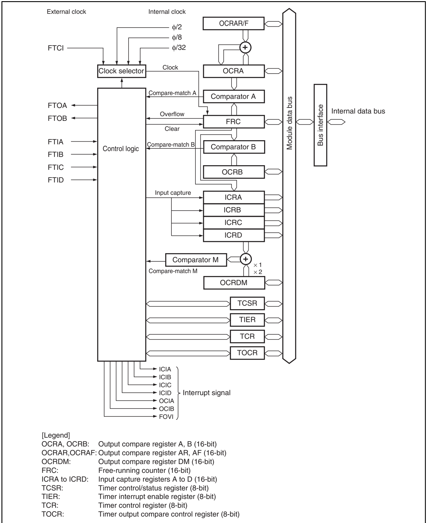
Figure 11.1 Block Diagram of 16-Bit Free-Running Timer
