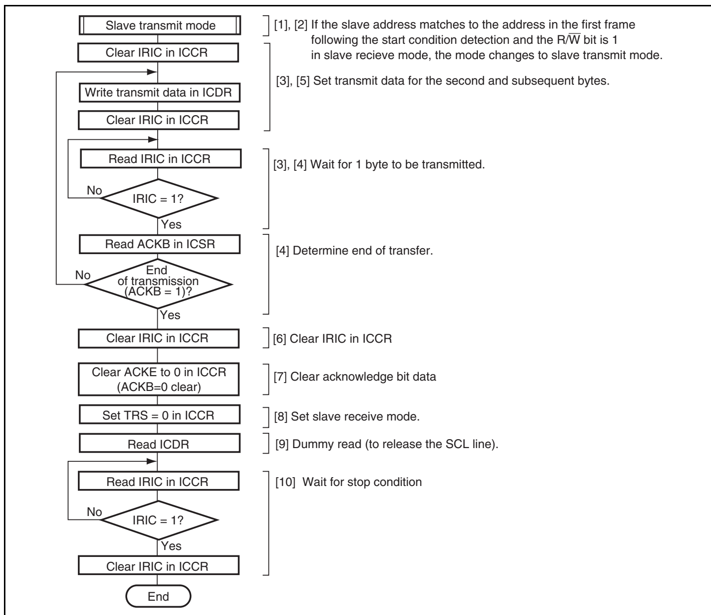
Figure 16.23 Sample Flowchart for Slave Transmit Mode
