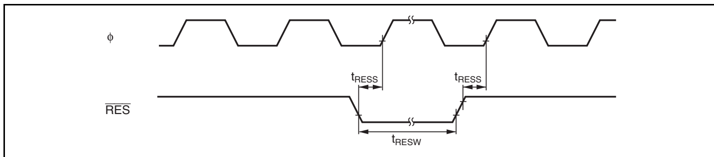
Figure 24.7 Reset Input Timing
