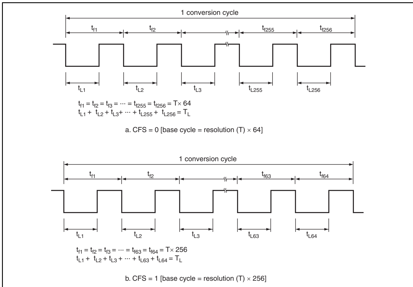
Figure 10.4 Output Waveform (OS = 0, DADR corresponds to T_L )
