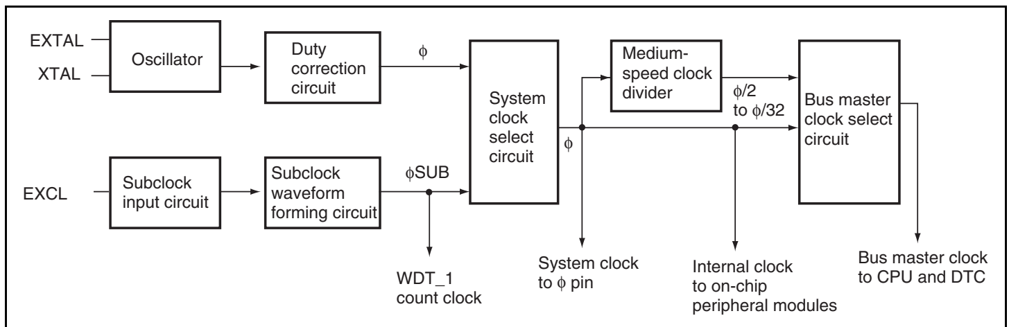
Figure 21.1 Block Diagram of Clock Pulse Generator
