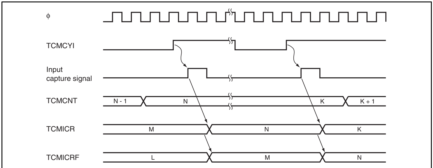
Figure 12.5 Buffer Operation of Input Capture
