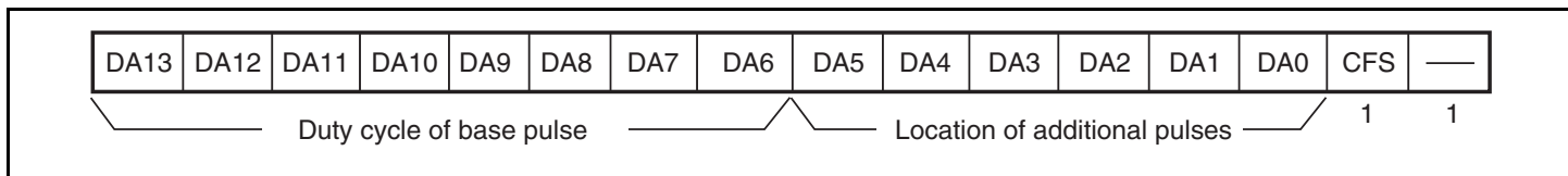
Figure 10.6 D/A Data Register Configuration when CFS = 1
