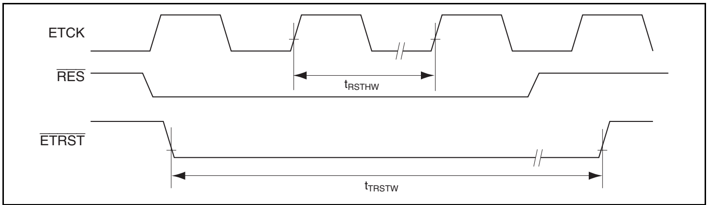
Figure 24.28 Reset Hold Timing
