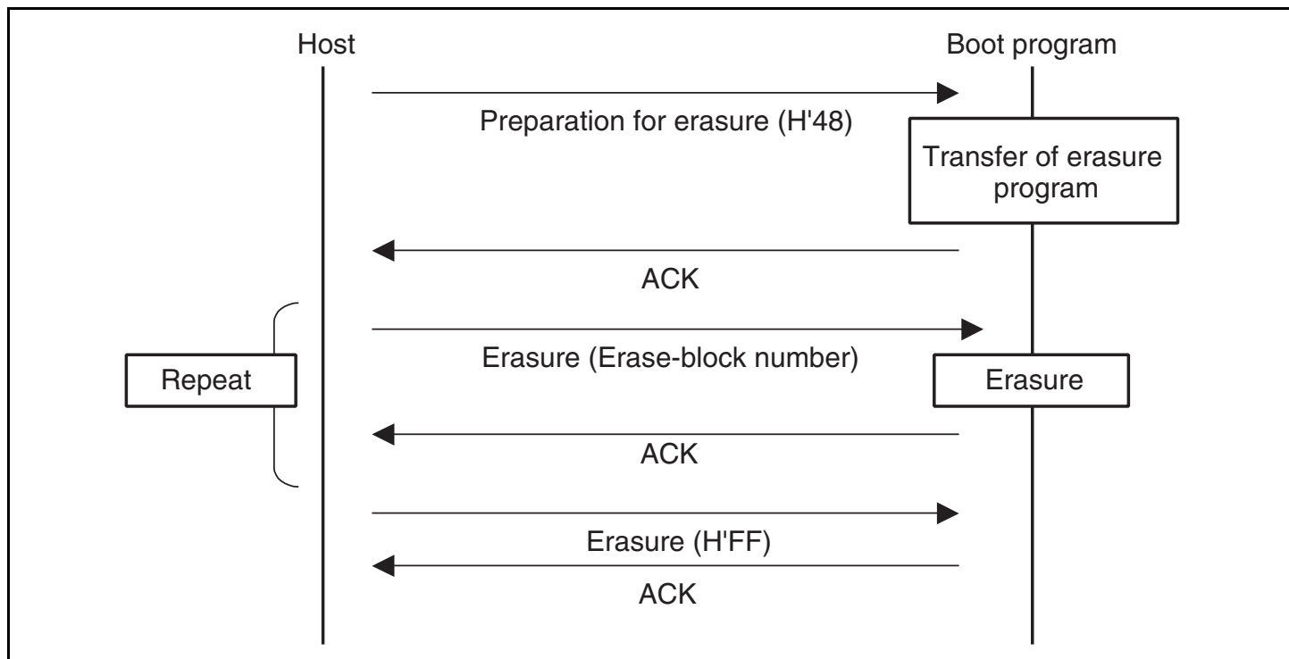
Figure 19.24 Erasure Sequence
