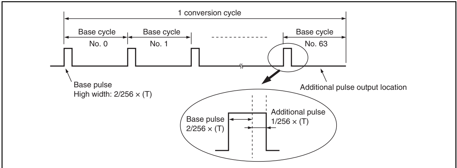
Figure 10.7 Output Waveform when DADR = H'0207 (OS = 1)
