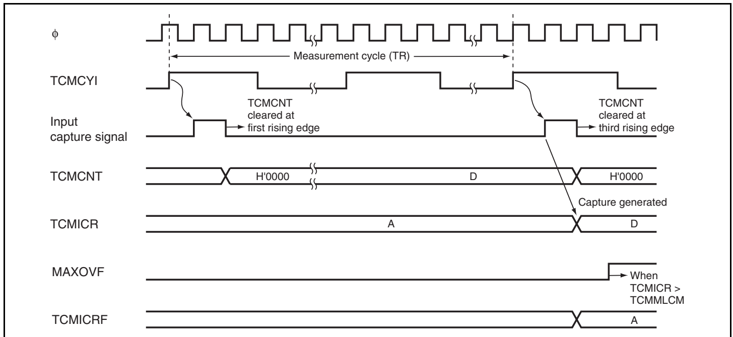
Figure 12.8 Example of Timing in Speed Measurement
