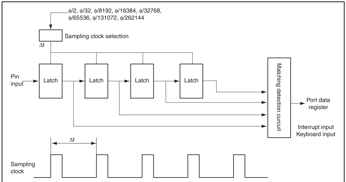
Figure 8.1 Noise Cancel Circuit
