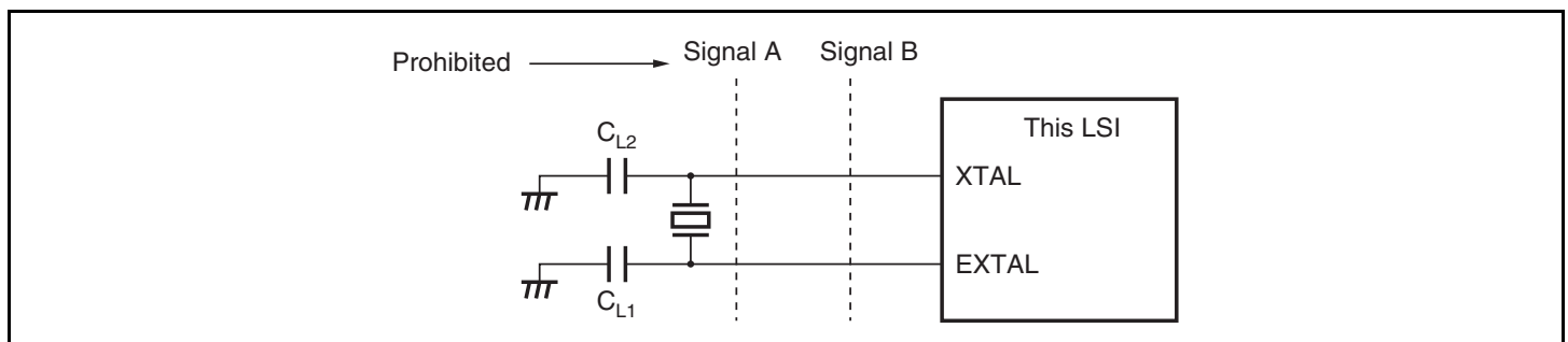
Figure 21.9 Note on Board Design of Oscillator Section
