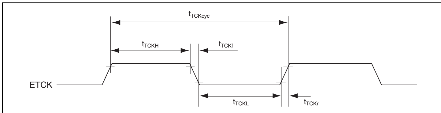
Figure 24.27 ETCK Timing
