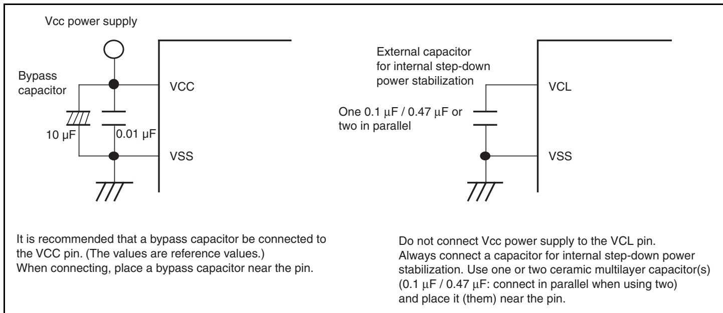
Figure 24.30 Connection of VCL Capacitor
