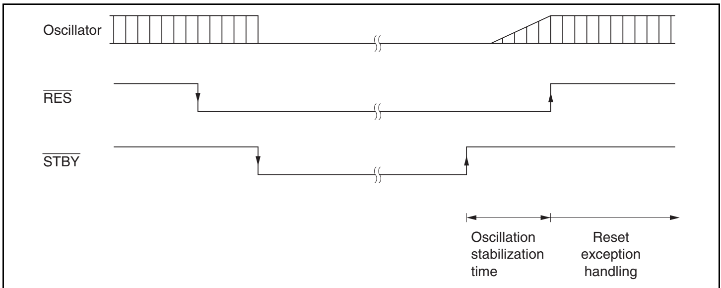
Figure 22.4 Hardware Standby Mode Timing
