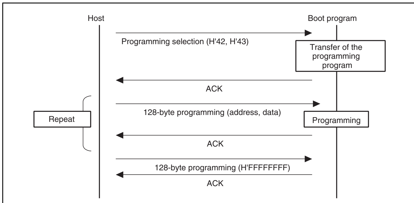
Figure 19.23 Programming Sequence
