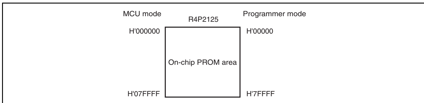
Figure 20.2 Memory Map in Programmer Mode
