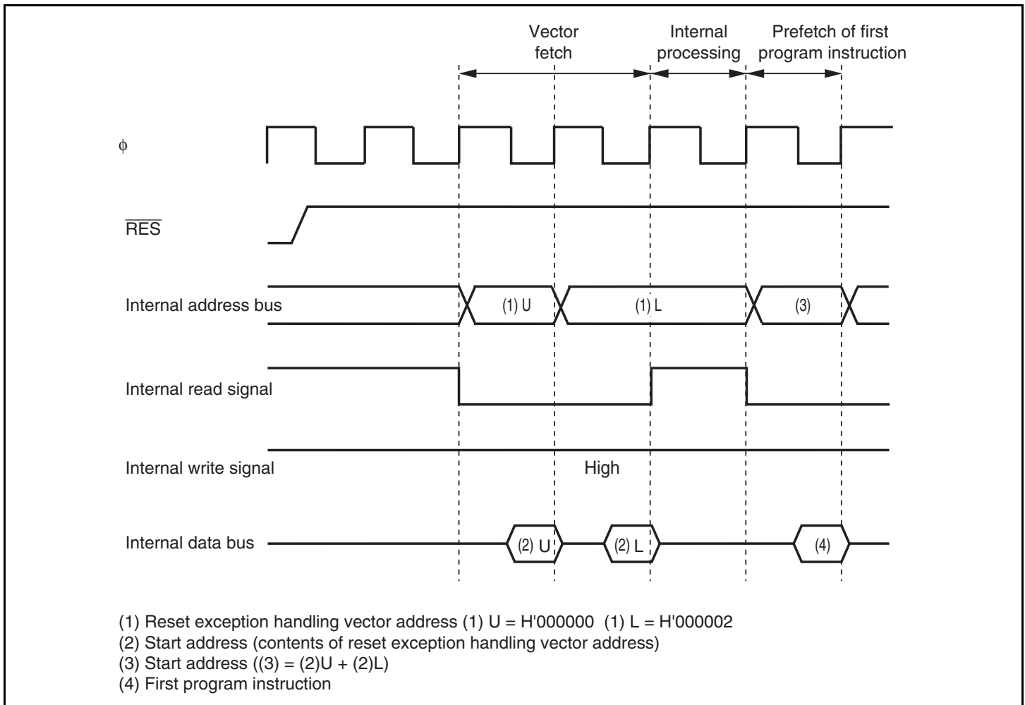
Figure 4.1 Reset Sequence (Mode 2)
