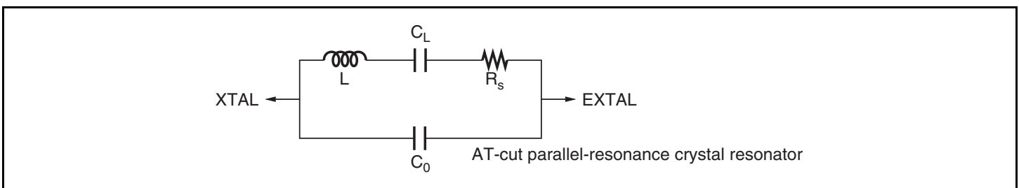
Figure 21.3 Equivalent Circuit of Crystal Resonator
