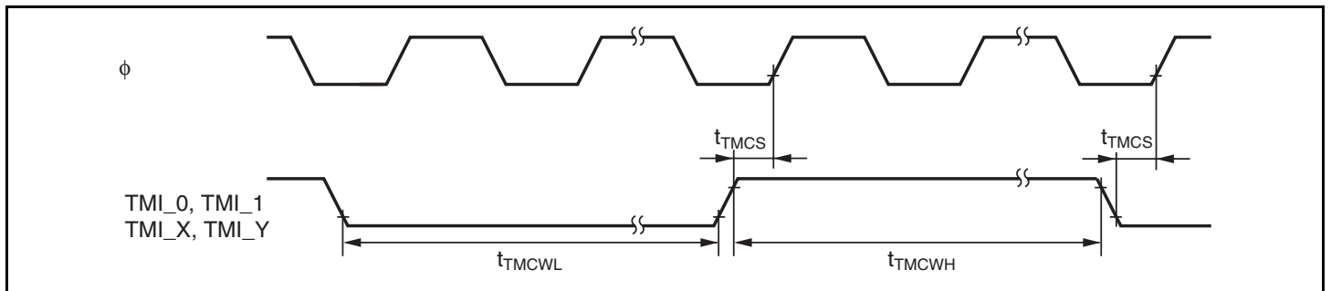
Figure 24.20 8-Bit Timer Clock Input Timing
