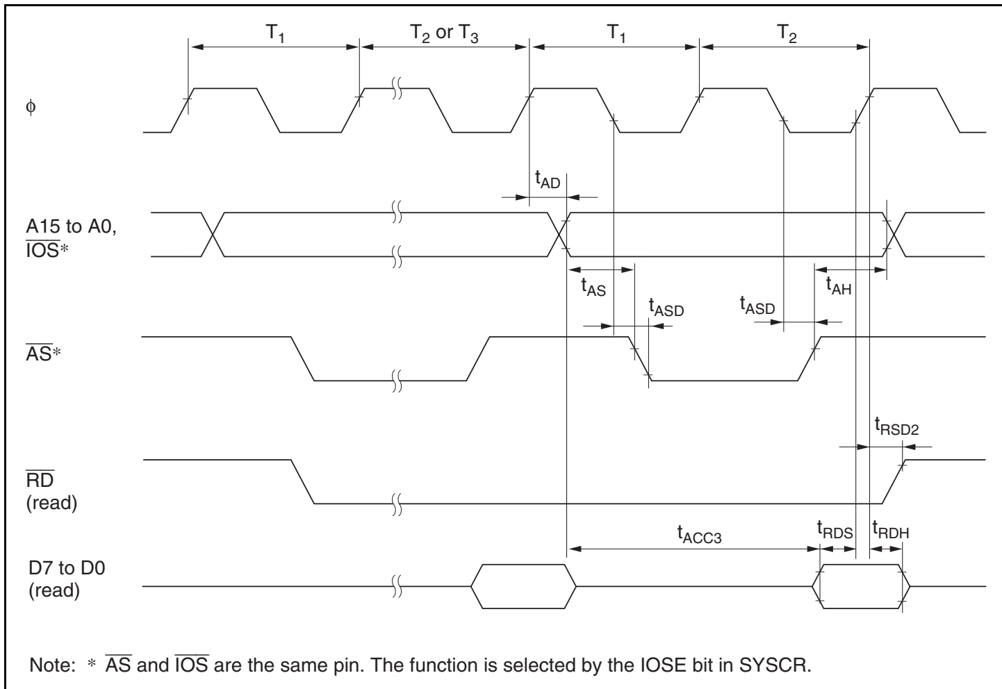
Figure 24.12 Burst ROM Access Timing (Two-State Access)
