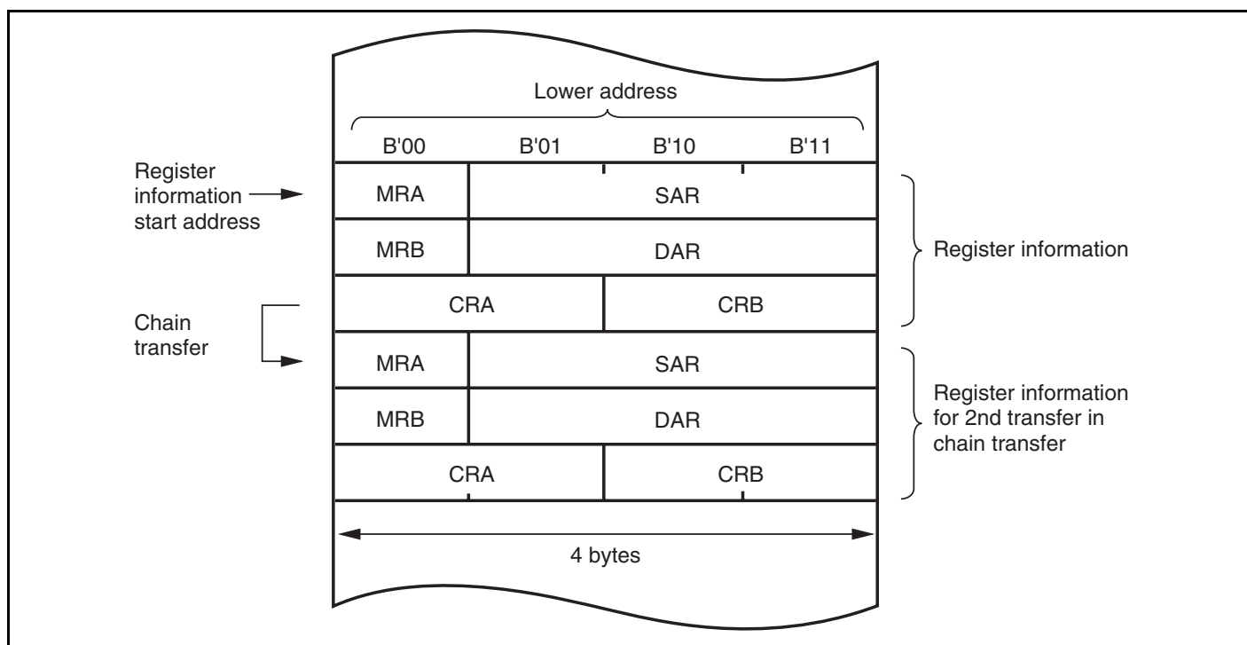
Figure 7.3 DTC Register Information Location in Address Space
