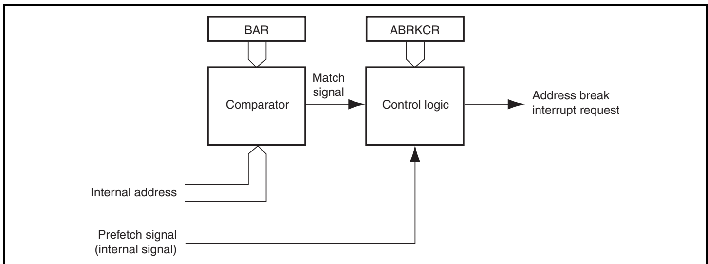
Figure 5.9 Block Diagram of Address Break Function
