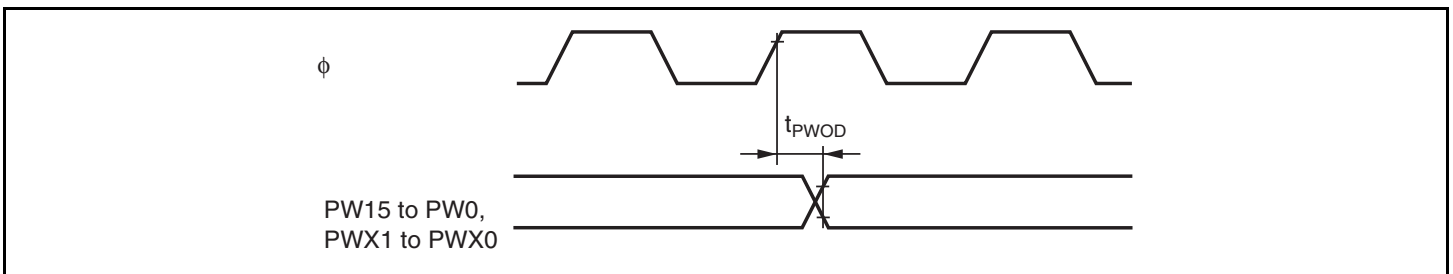
Figure 24.22 PWM, PWMX Output Timing
