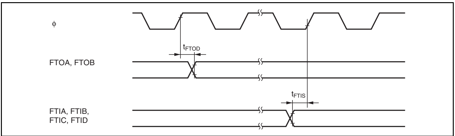
Figure 24.15 FRT Input/Output Timing
