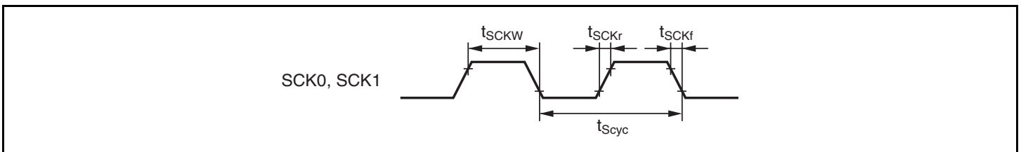
Figure 24.23 SCK Clock Input Timing
