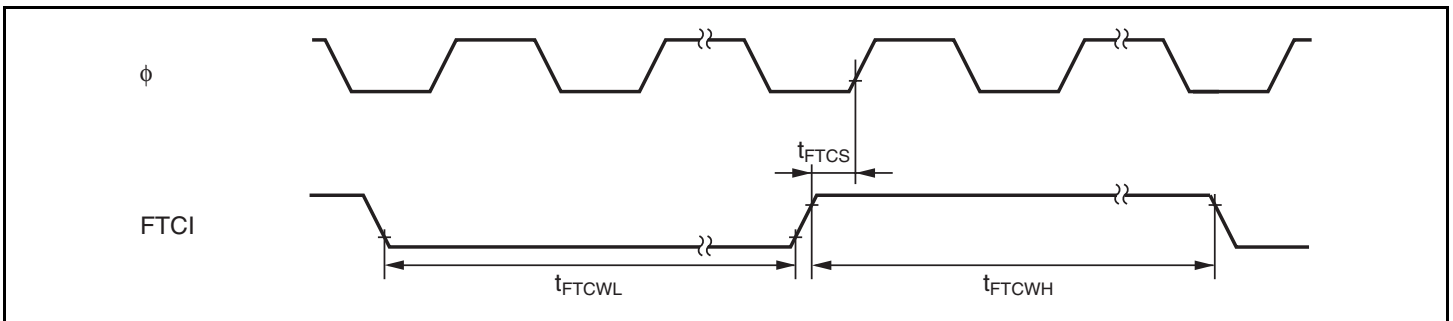
Figure 24.16 FRT Clock Input Timing
