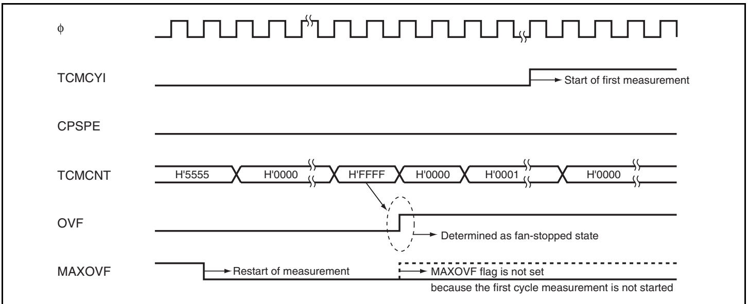
Figure 12.10 Example of Timing in Fan-Stopped State (2)
