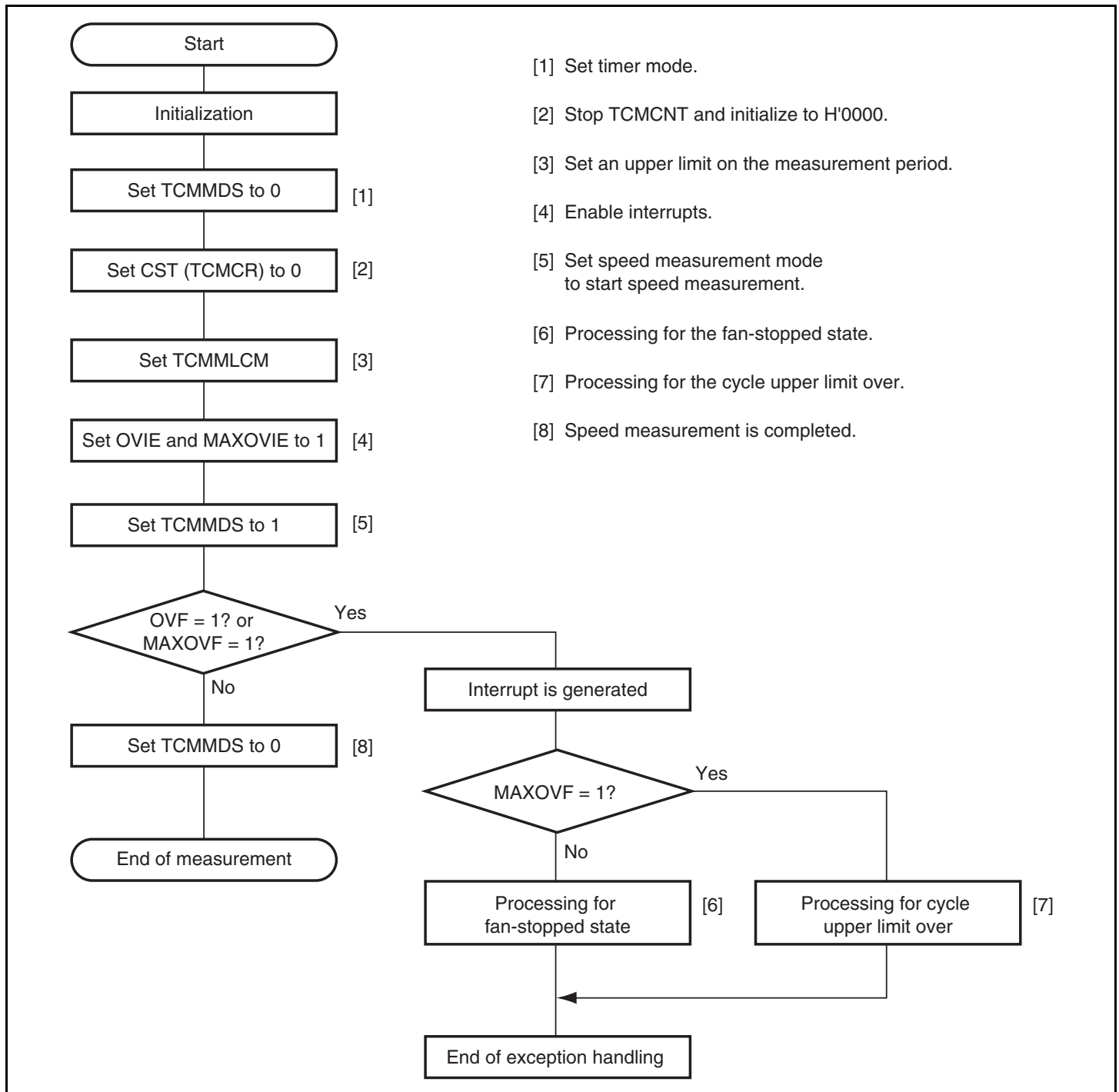
Figure 12.11 Example of Speed Measurement Mode Settings
