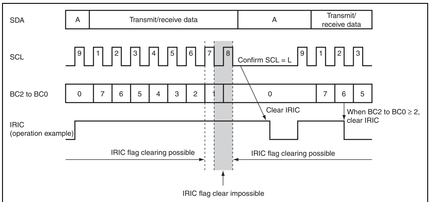
Figure 16.36 IRIC Flag Clear Timing in Wait Operation
