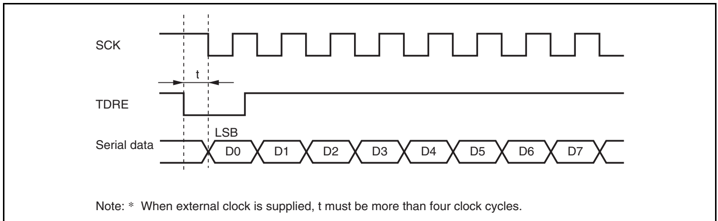
Figure 15.21 Example of Transmission using DTC in Clocked Synchronous Mode
