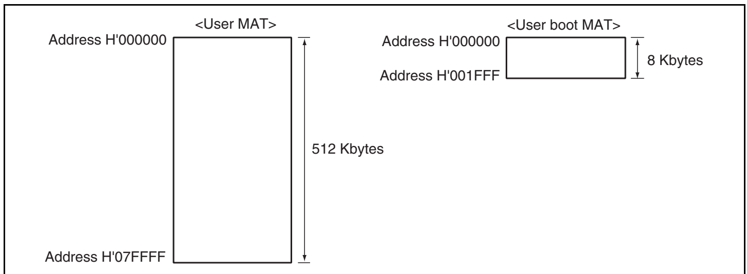
Figure 19.3 Flash Memory Configuration
