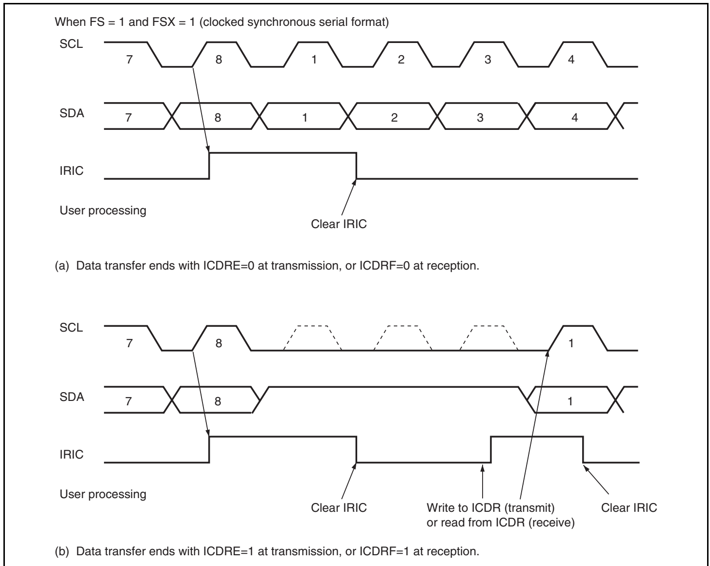
Figure 16.27 IRIC Setting Timing and SCL Control (3)
