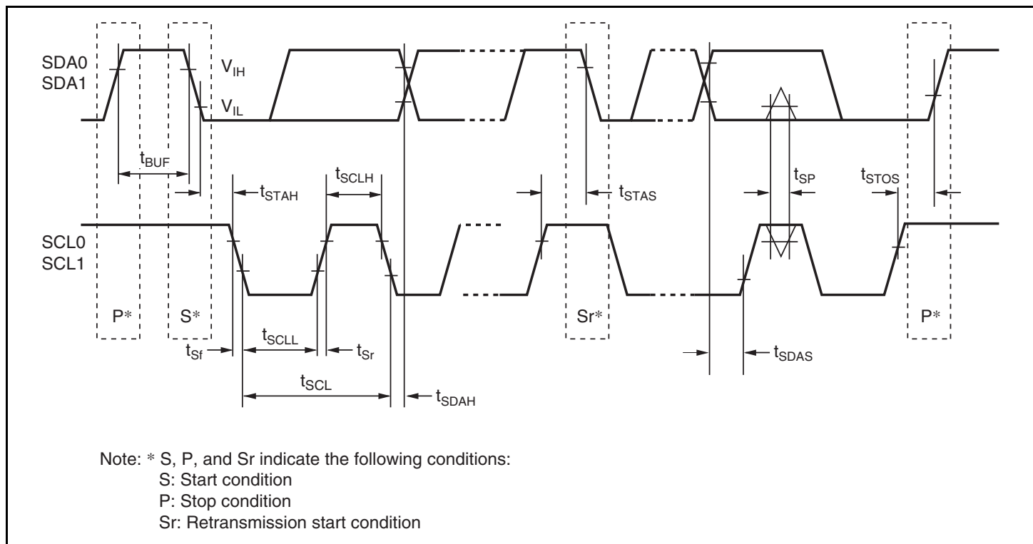
Figure 24.26 I 2 C Bus Interface Input/Output Timing
