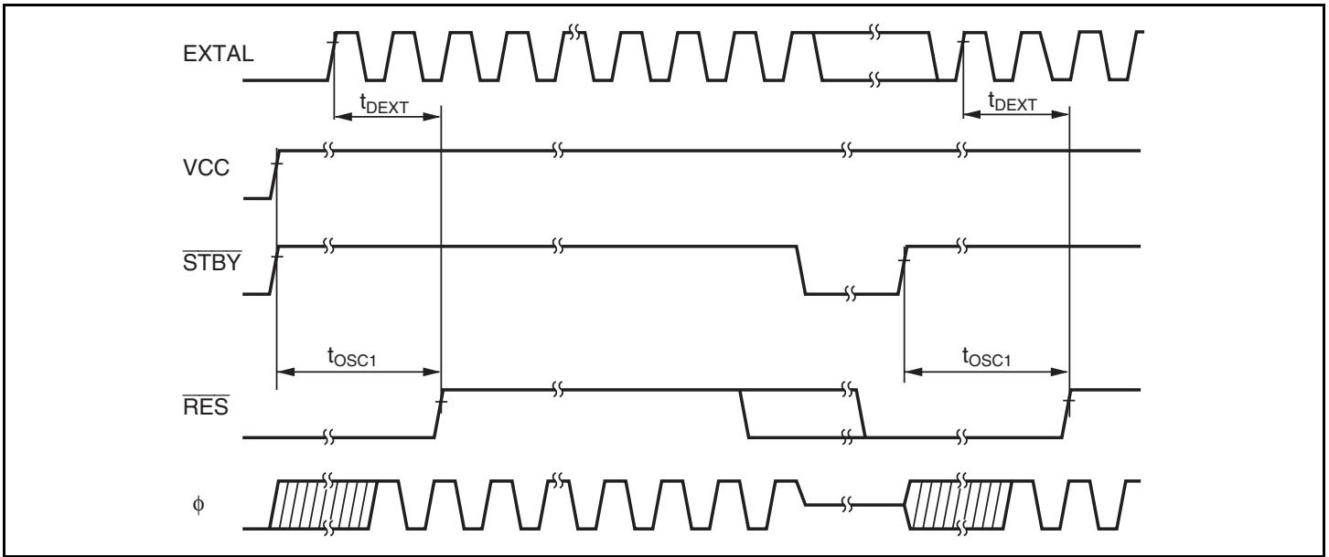
Figure 24.5 Oscillation Stabilization Timing
