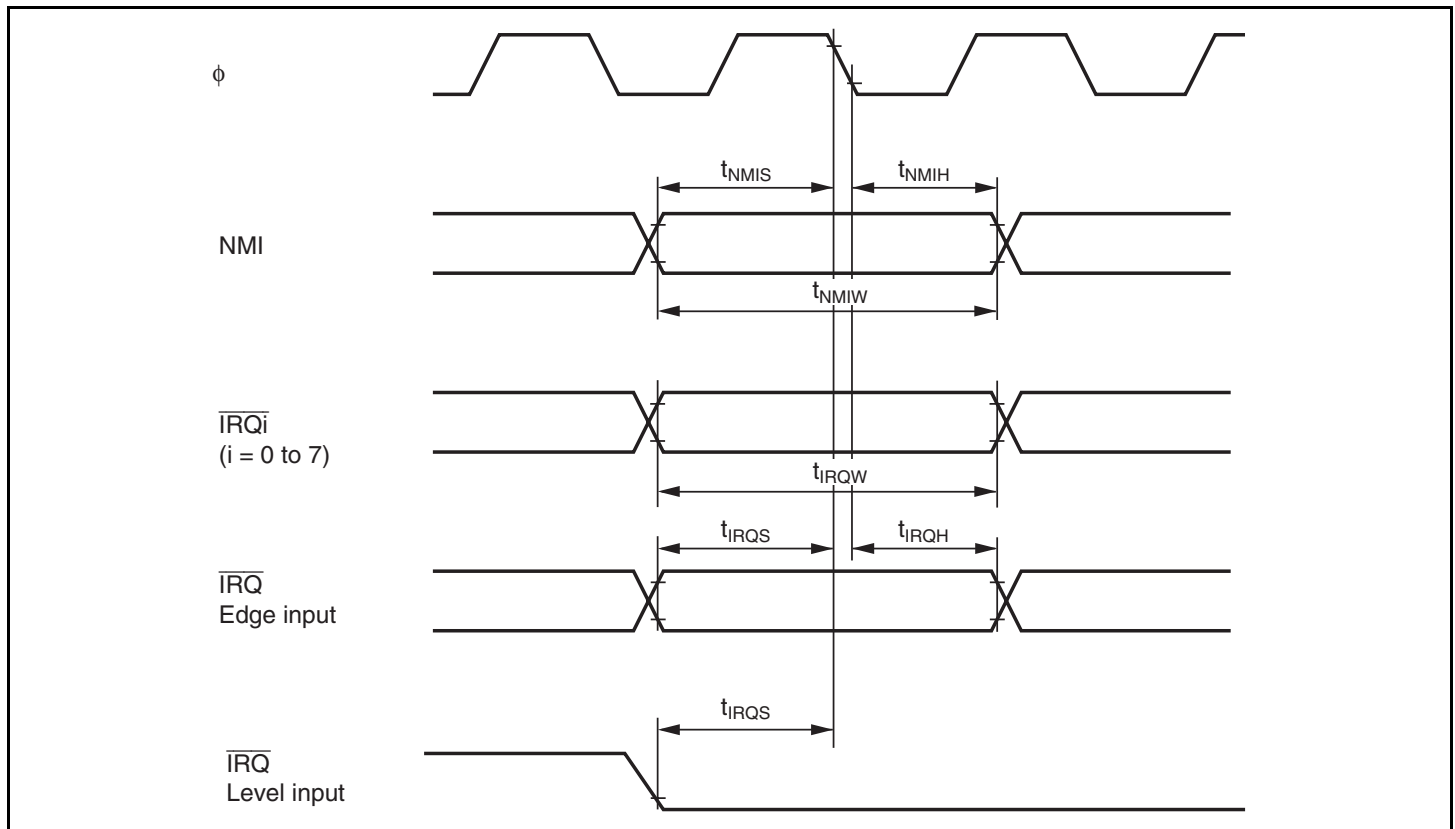
Figure 24.8 Interrupt Input Timing
