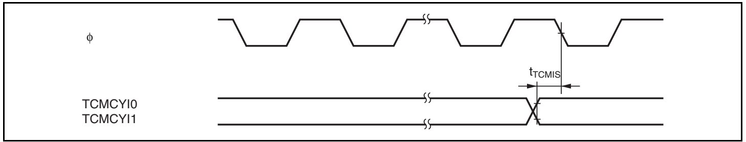
Figure 24.17 TCM Input/Output Timing
