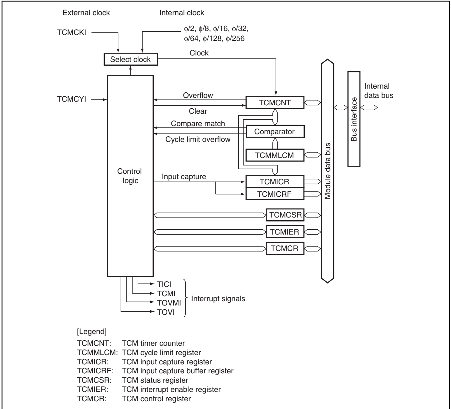
Figure 12.1 Block Diagram of the TCM
