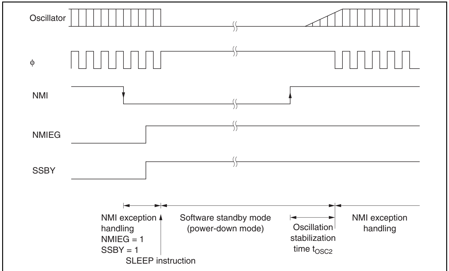
Figure 22.3 Software Standby Mode Application Example
