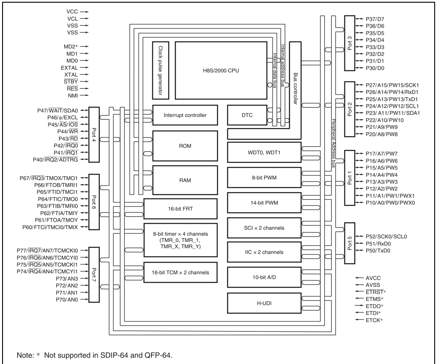
Figure 1.1 Block Diagram
