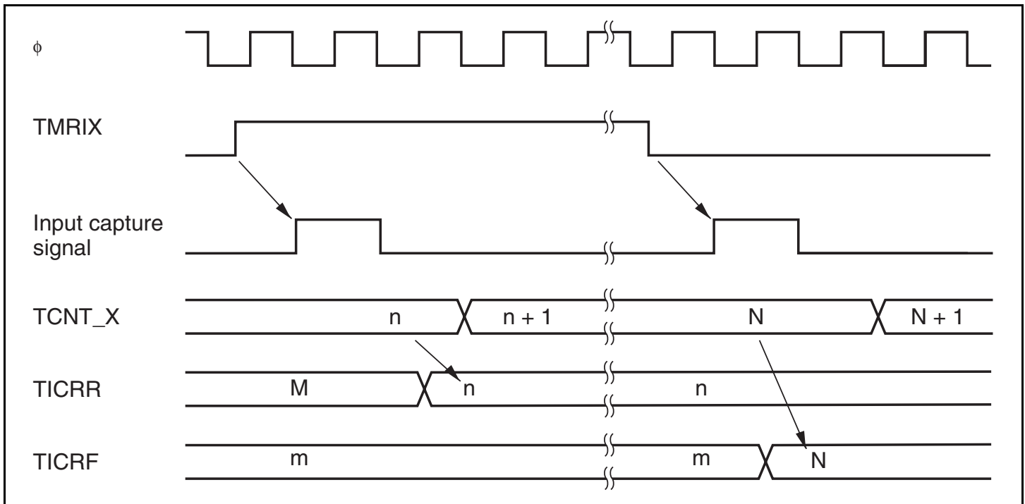
Figure 13.11 Timing of Input Capture Operation
