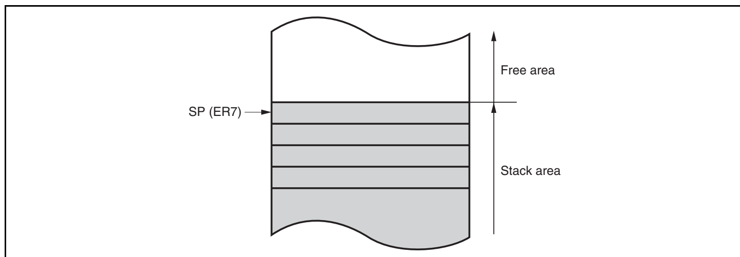
Figure 2.8 Stack
