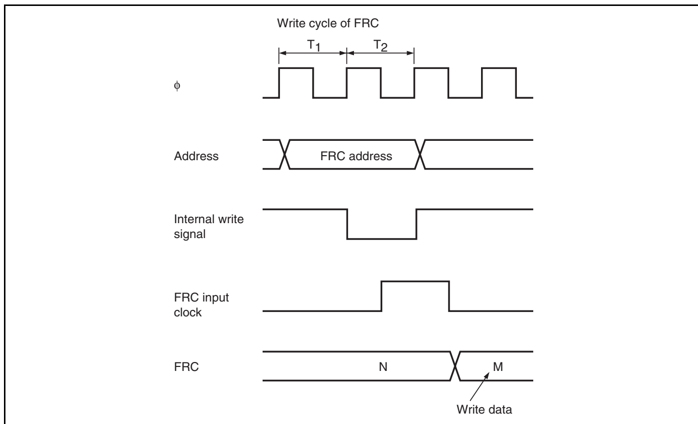
Figure 11.18 Conflict between FRC Write and Increment
