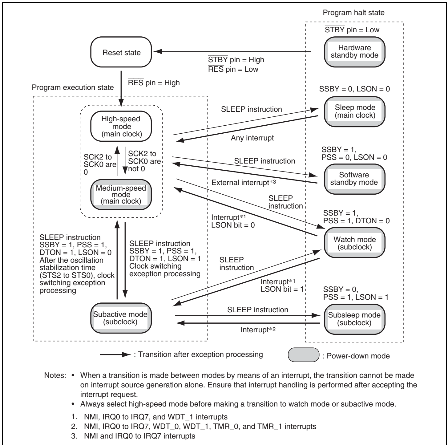
Figure 22.1 Mode Transition Diagram
