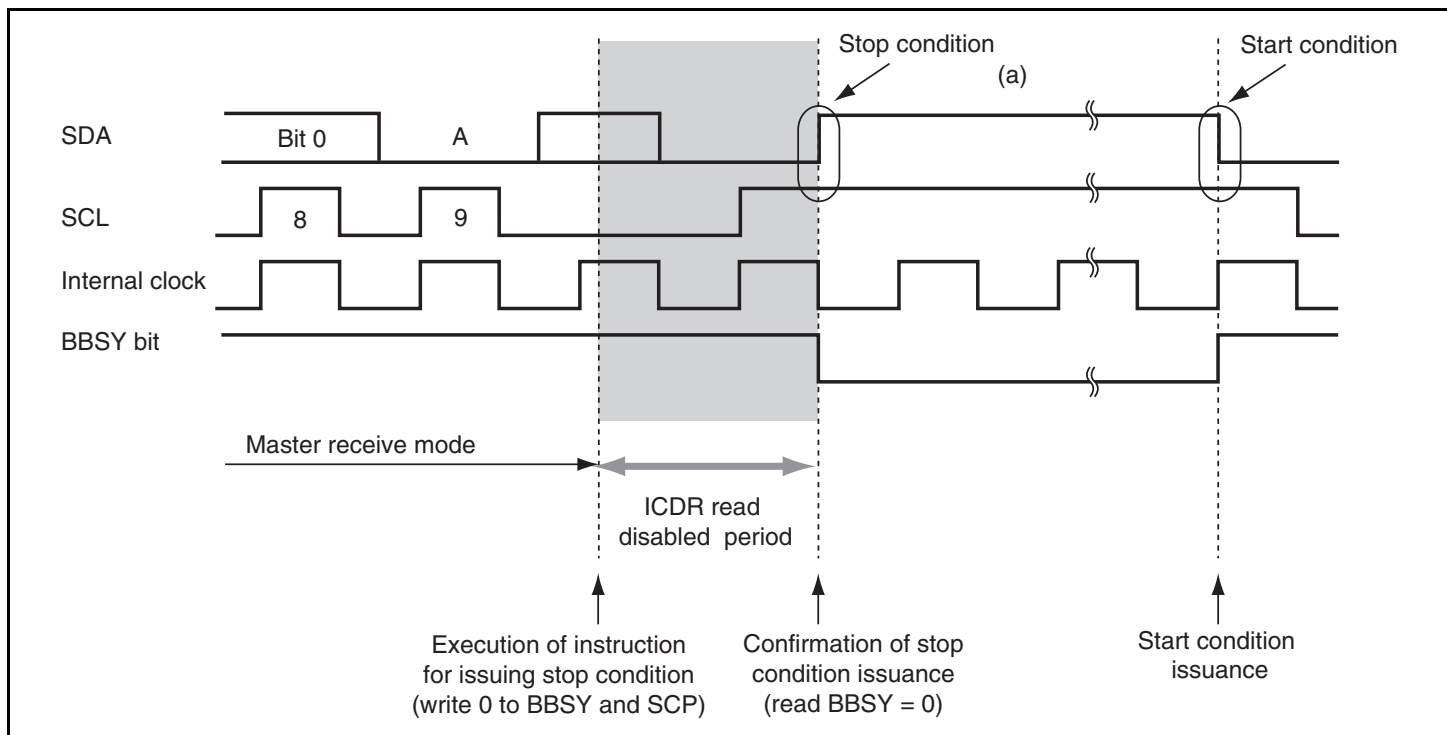
Figure 16.29 Notes on Reading Master Receive Data
