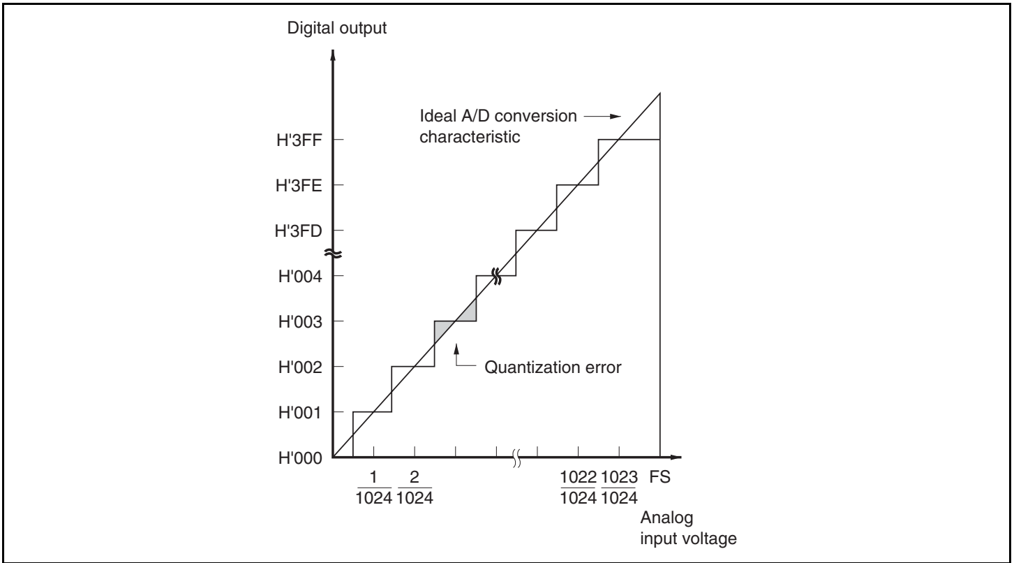
Figure 17.4 A/D Conversion Accuracy Definitions
