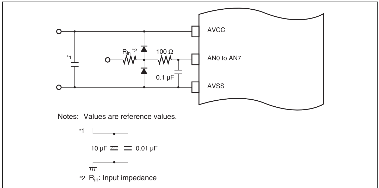
Figure 17.7 Example of Analog Input Protection Circuit
