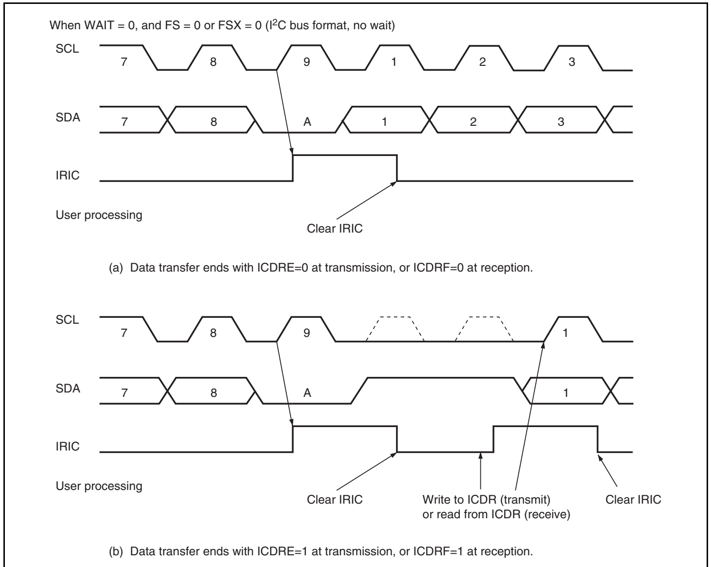
Figure 16.25 IRIC Setting Timing and SCL Control (1)
