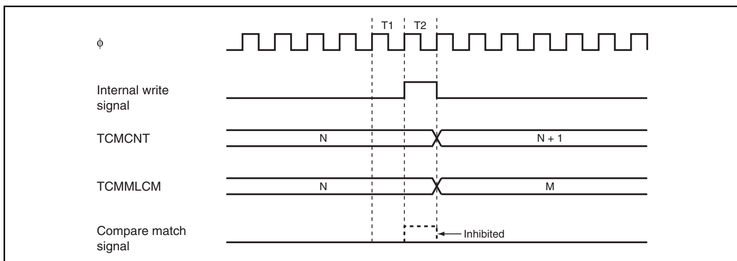
Figure 12.13 Conflict between TCMMLCM Write and Compare Match
