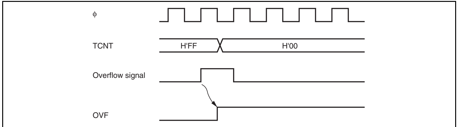
Figure 13.10 Timing of OVF Flag Setting
