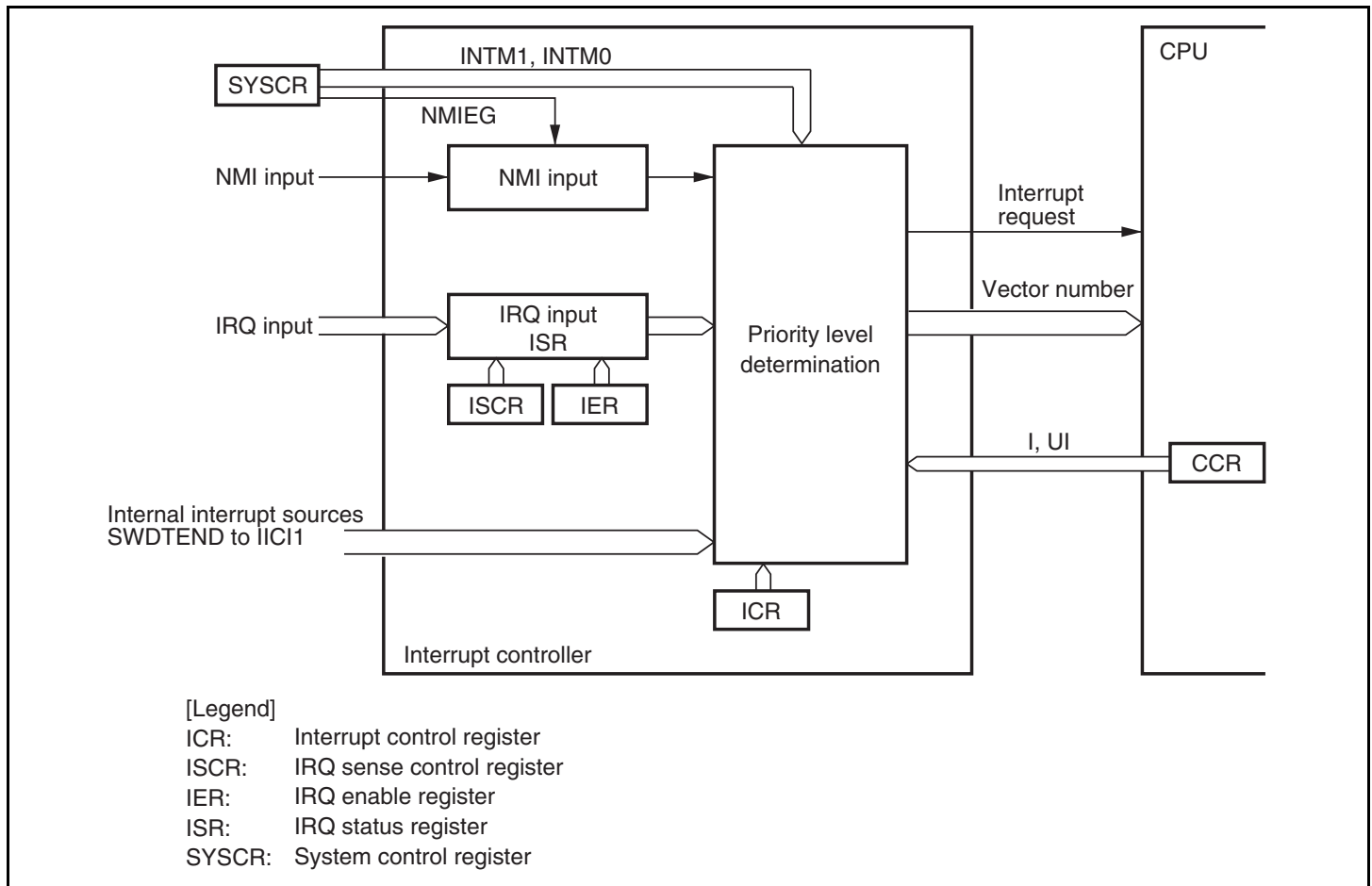
Figure 5.1 Block Diagram of Interrupt Controller
