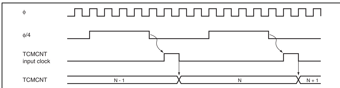
Figure 12.2 Example of Free Running Counter Operation
