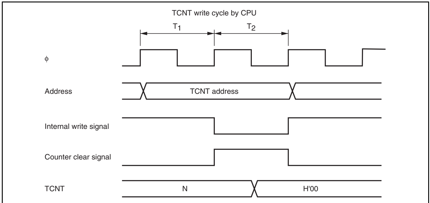
Figure 13.13 Conflict between TCNT Write and Clear
