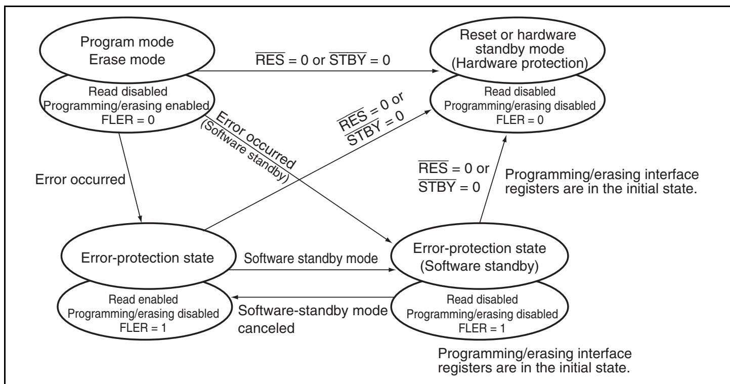
Figure 19.16 Transitions to Error-Protection State
