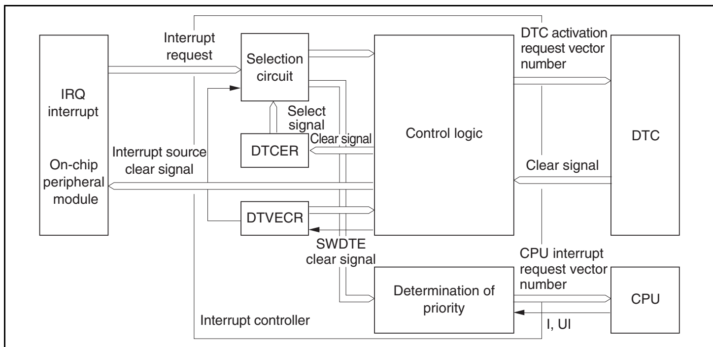
Figure 5.8 Interrupt Control for DTC
