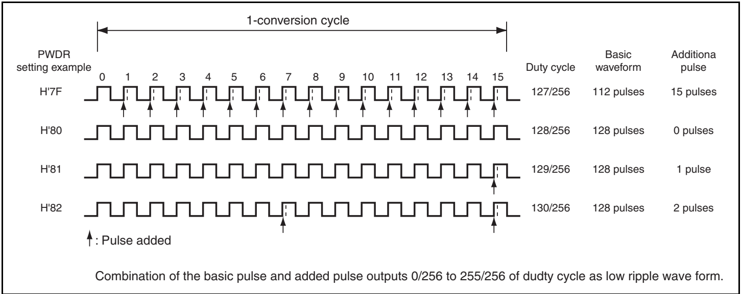
Figure 9.3 Example of PWM Setting
