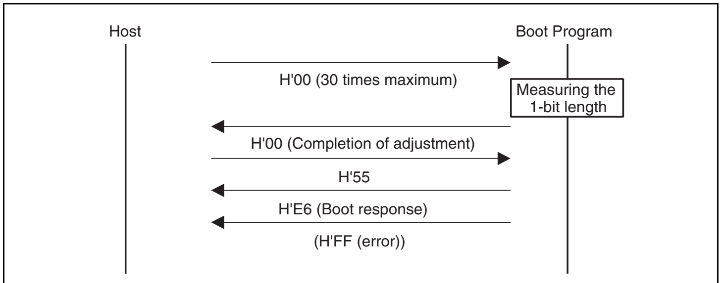
Figure 19.20 Bit-Rate-Adjustment Sequence
