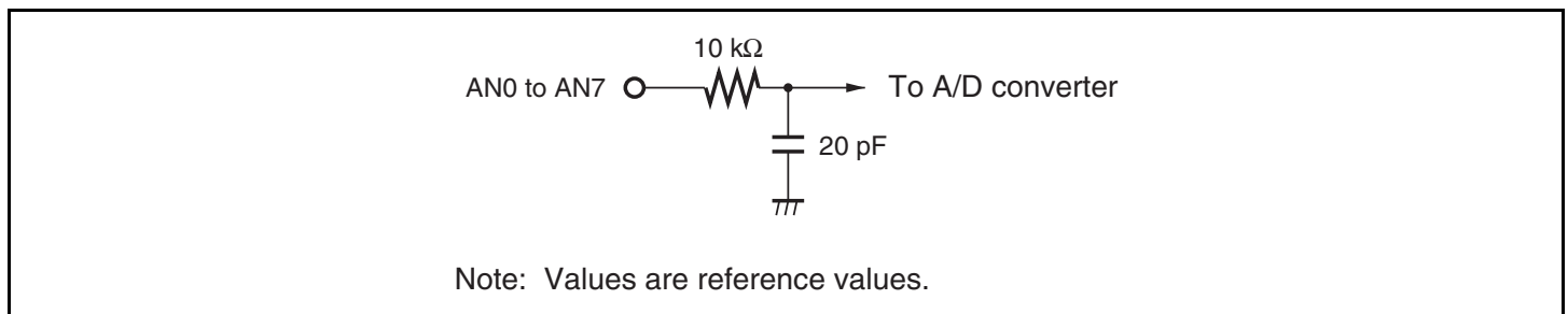
Figure 17.8 Analog Input Pin Equivalent Circuit
