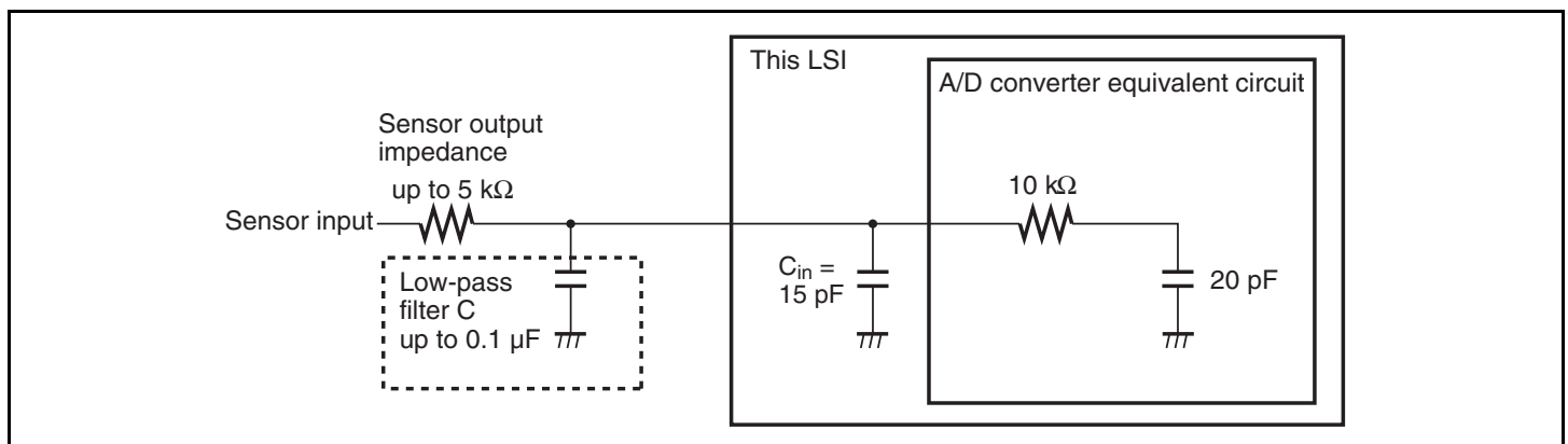
Figure 17.6 Example of Analog Input Circuit
