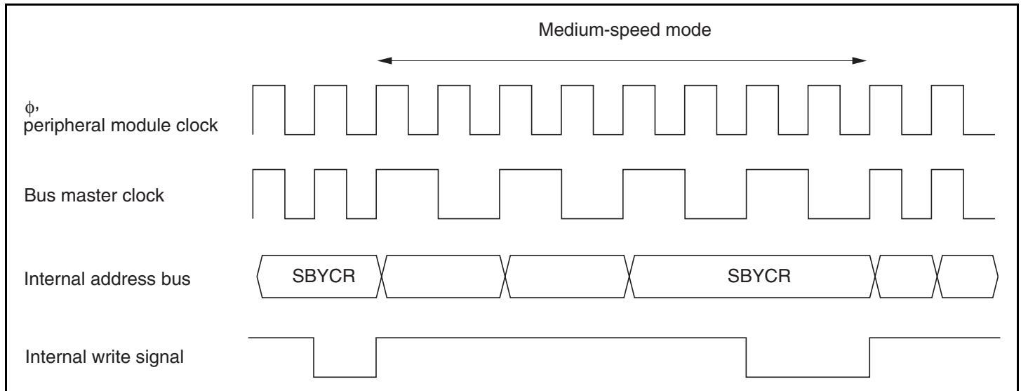
Figure 22.2 Medium-Speed Mode Timing
