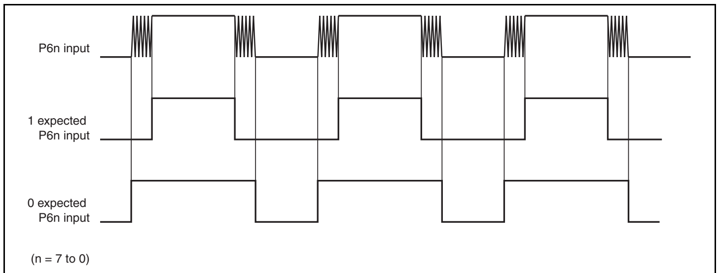
Figure 8.2 Conceptual Diagram of Noise Cancel Operation
