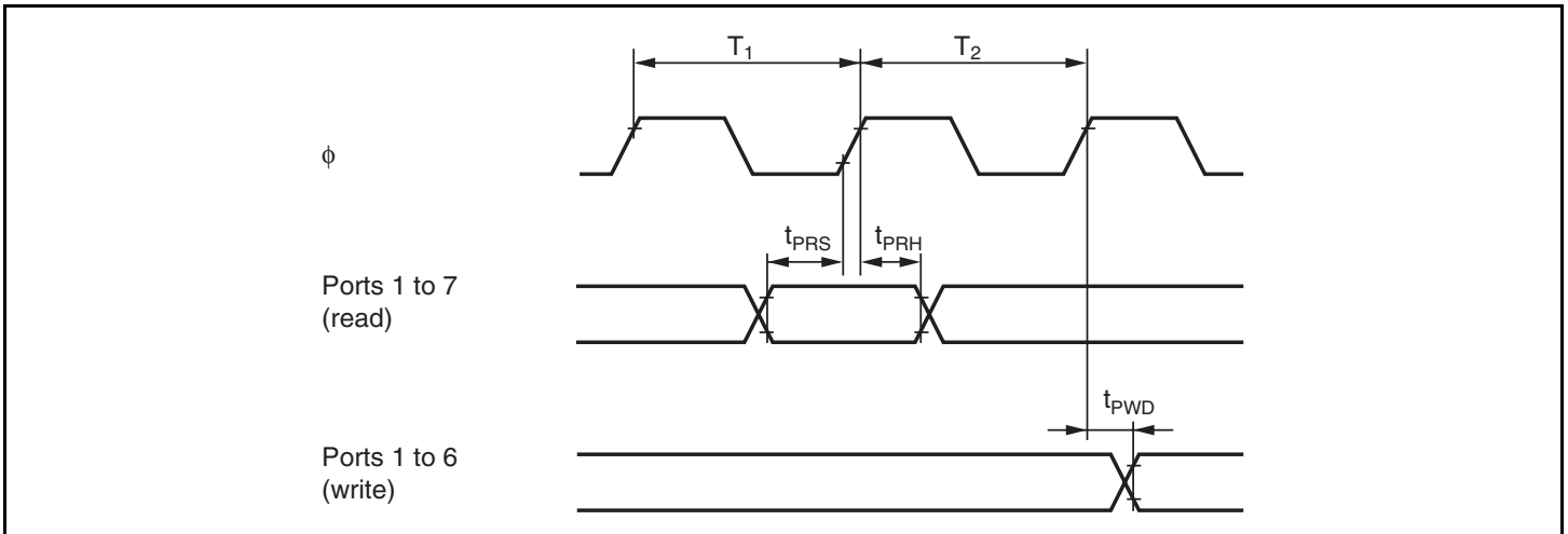
Figure 24.14 I/O Port Input/Output Timing
