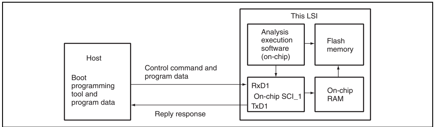
Figure 19.6 System Configuration in Boot Mode
