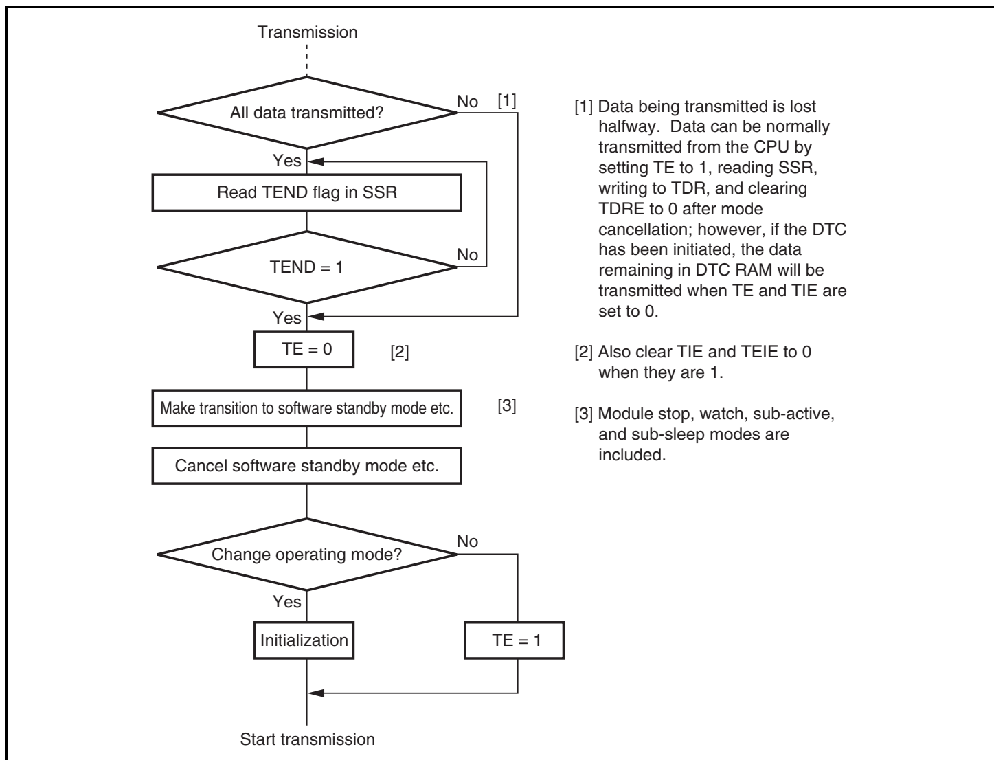
Figure 15.22 Sample Flowchart for Mode Transition during Transmission
