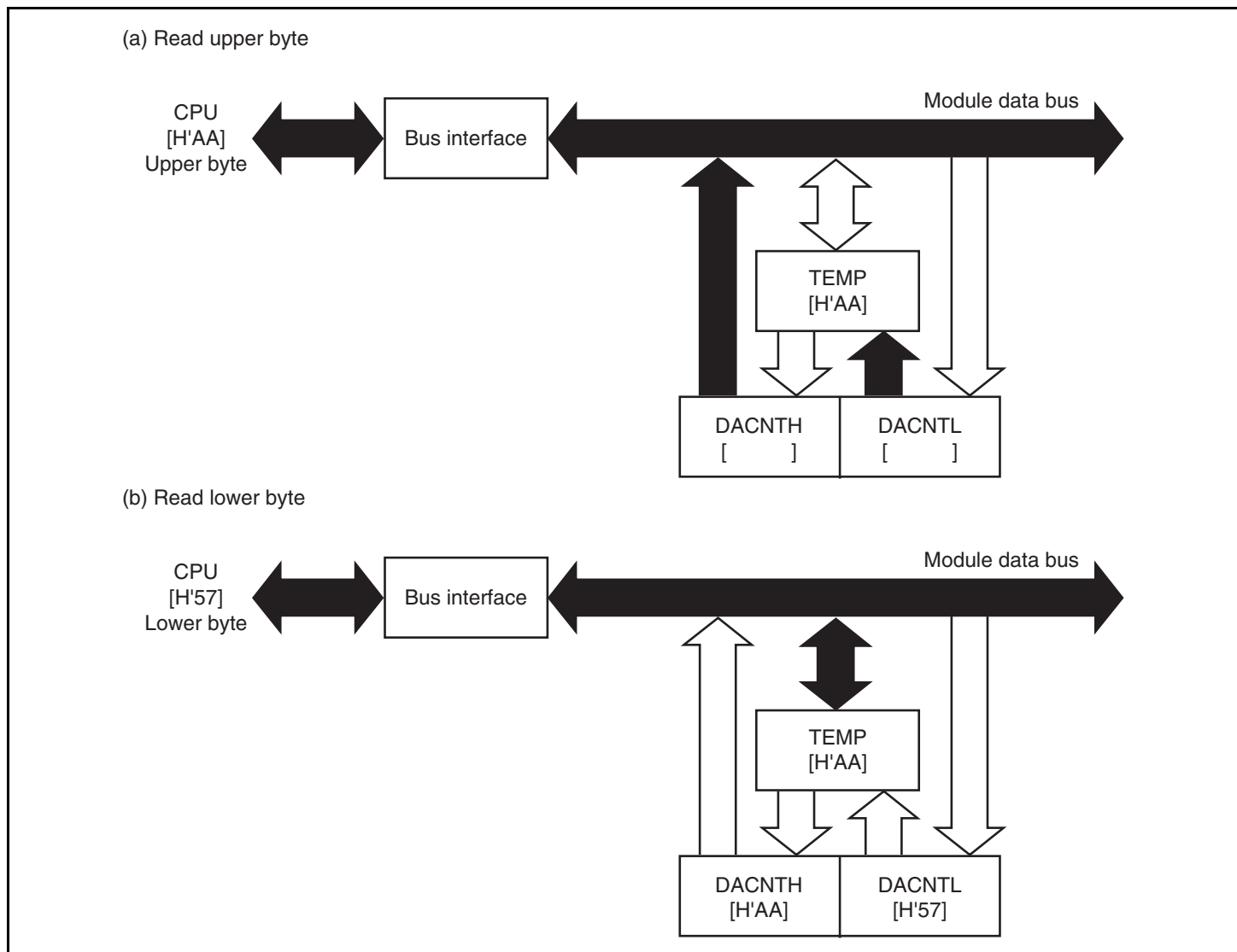
Figure 10.2 (2) DACNT Access Operation (2) [DACNT → CPU(H'AA57) Reading]
