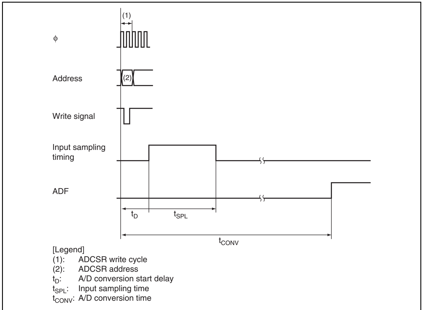
Figure 17.2 A/D Conversion Timing
