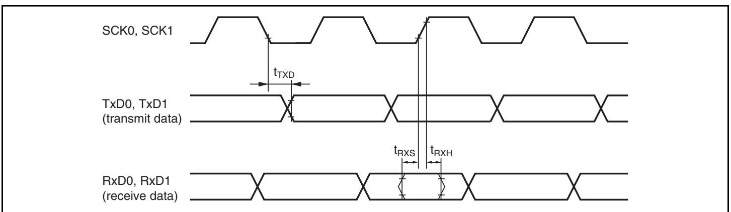
Figure 24.24 SCI Input/Output Timing (Clock Synchronous Mode)
