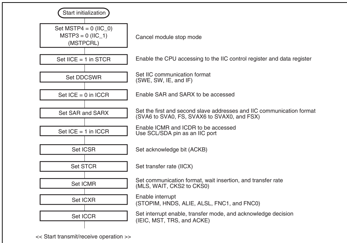
Figure 16.6 Sample Flowchart for IIC Initialization
