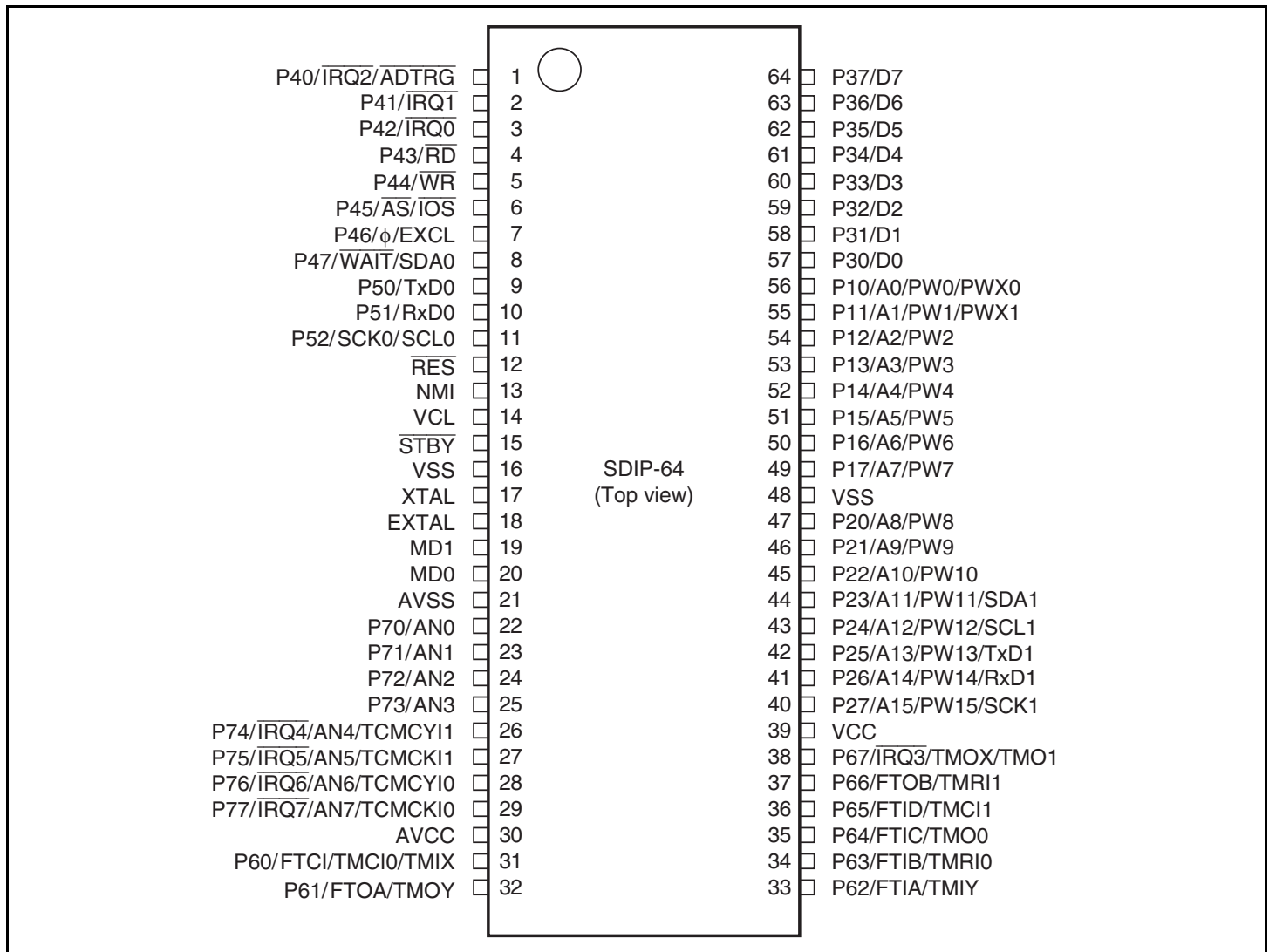
Figure 1.2 Pin Assignments (SDIP-64)
