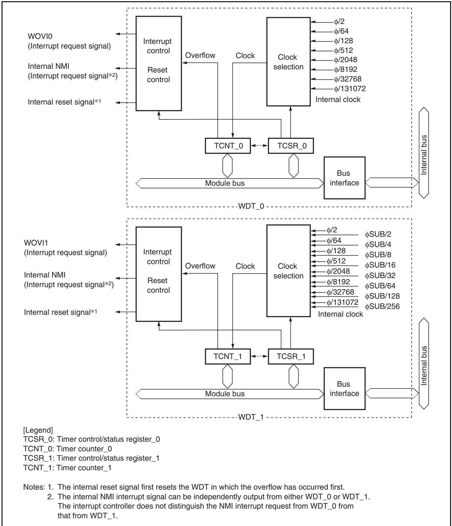
Figure 14.1 Block Diagram of WDT
