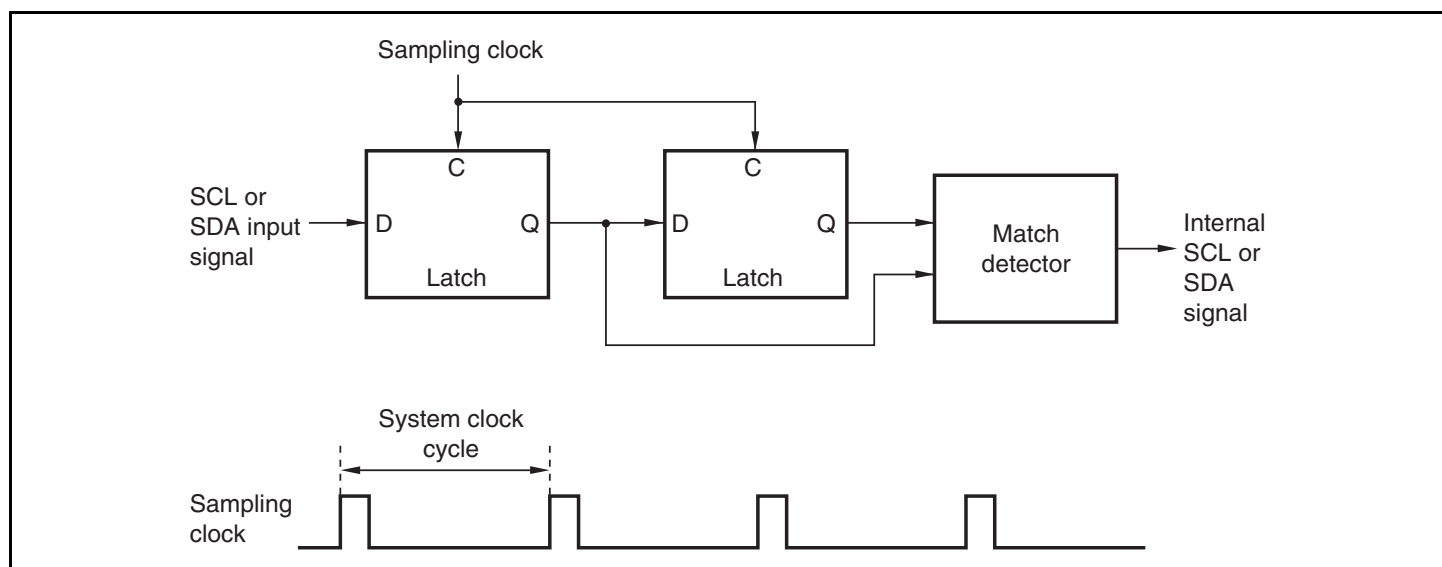
Figure 16.28 Block Diagram of Noise Canceller
