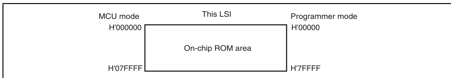
Figure 19.18 Memory Map in Programmer Mode
