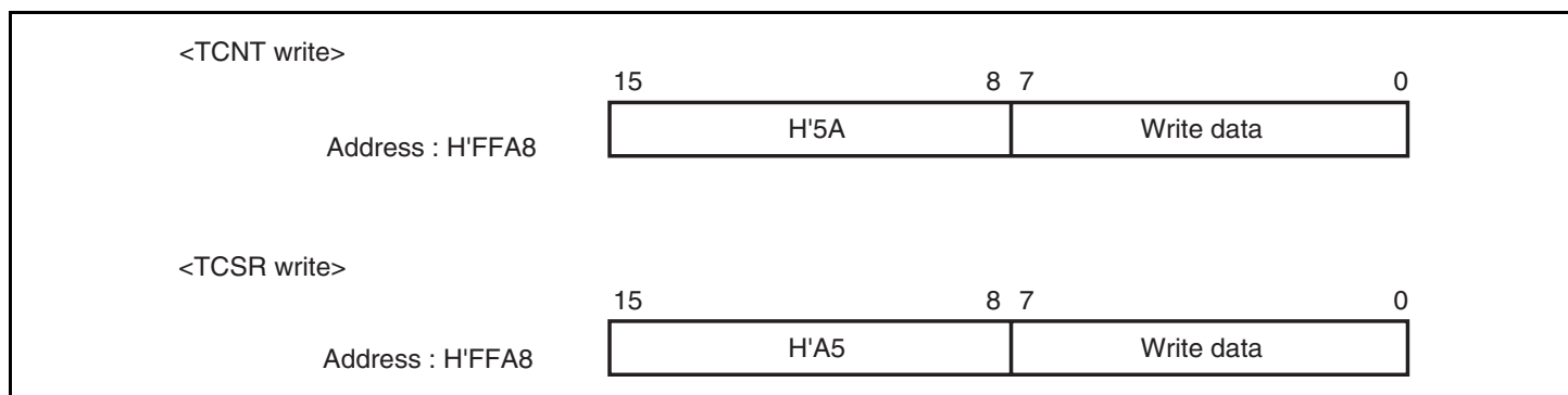
Figure 14.5 Writing to TCNT and TCSR (WDT_0)
