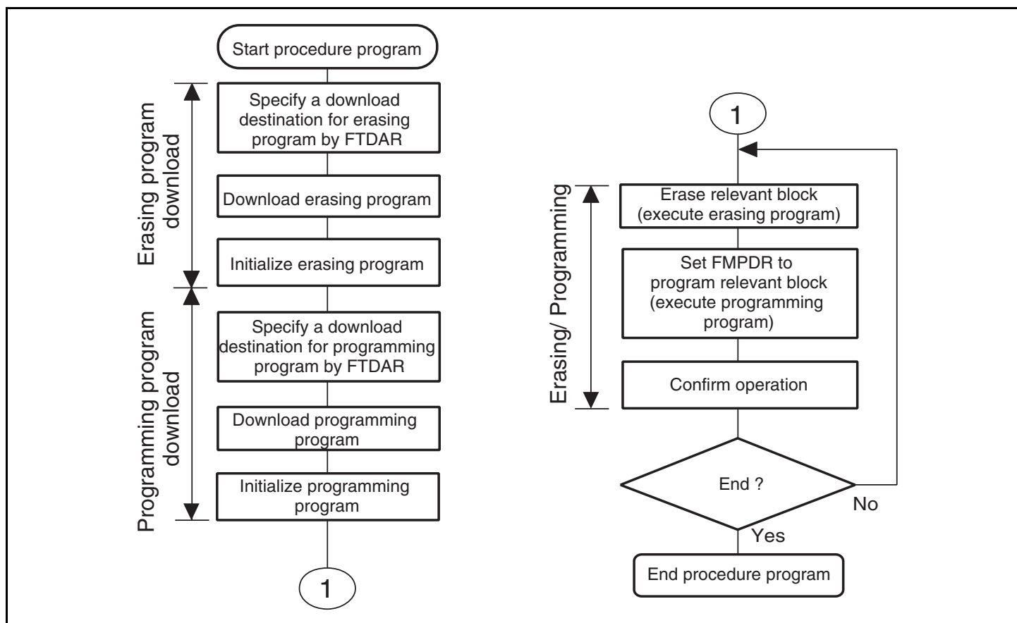
Figure 19.13 Repeating Procedure of Erasing and Programming
