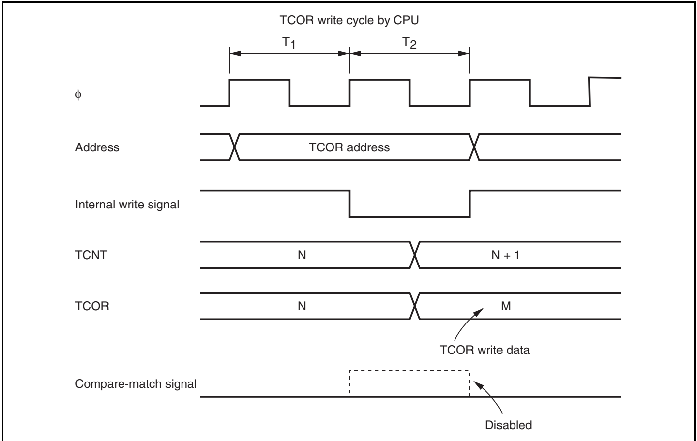
Figure 13.15 Conflict between TCOR Write and Compare-Match
