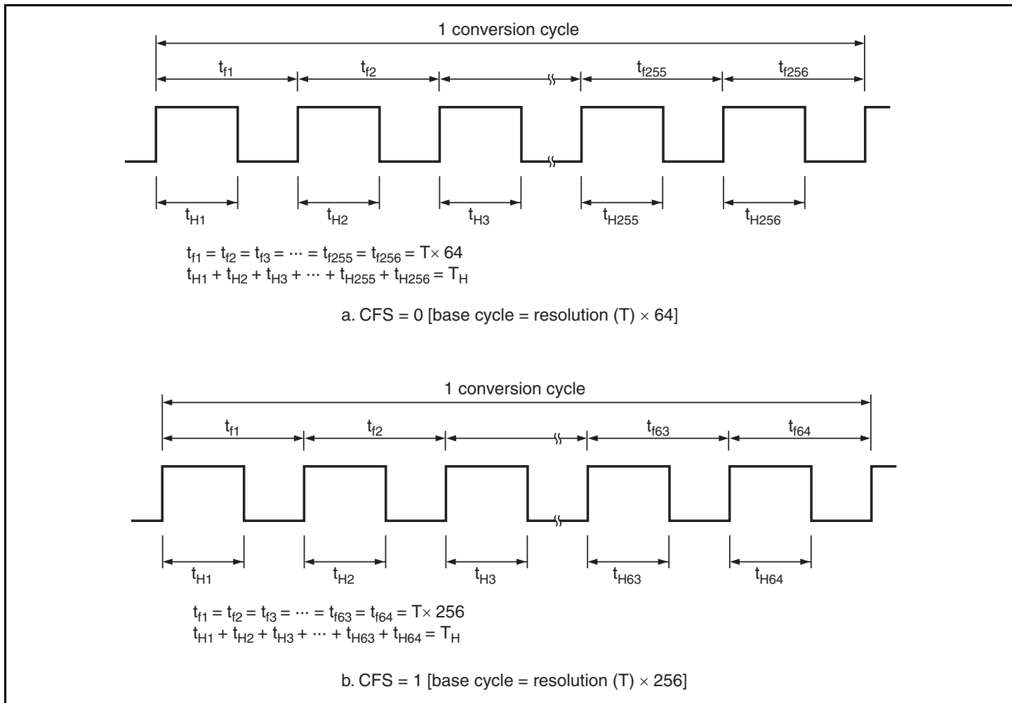
Figure 10.5 Output Waveform (OS = 1, DADR corresponds to T H )
