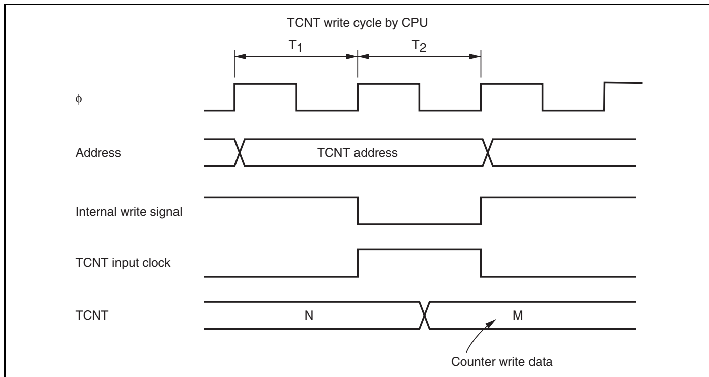
Figure 13.14 Conflict between TCNT Write and Count-Up
