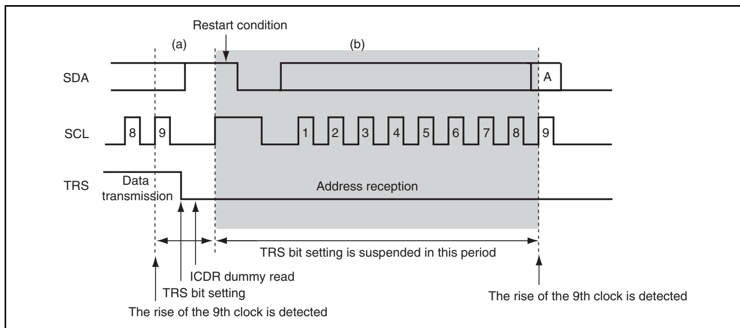
Figure 16.34 TRS Bit Set Timing in Slave Mode
