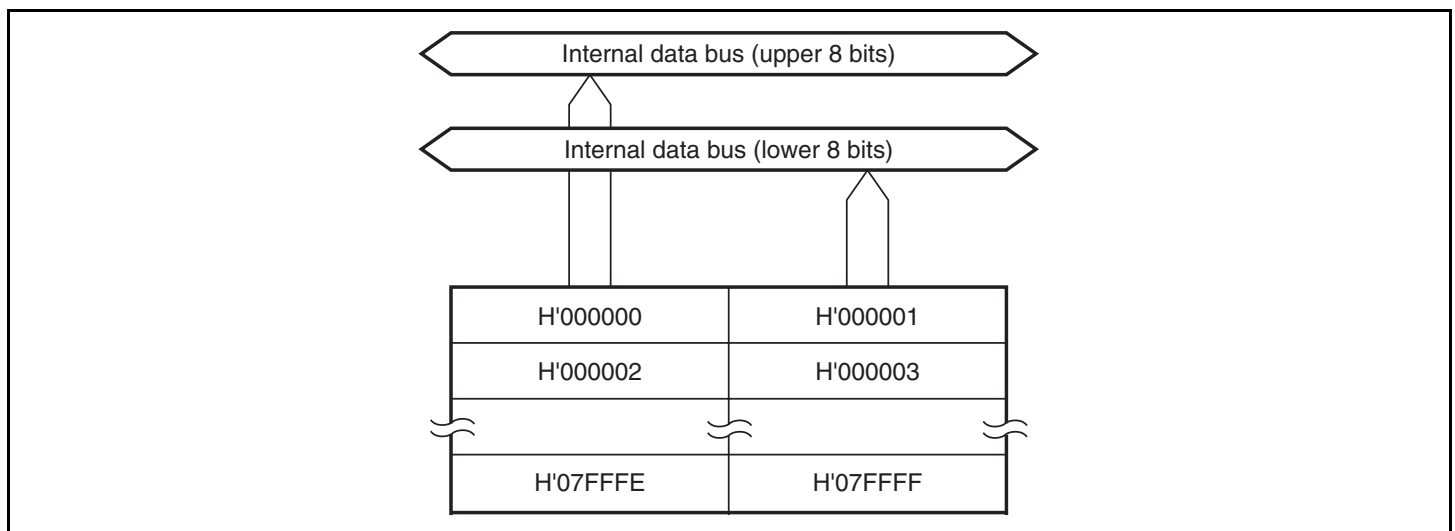
Figure 20.1 PROM Block Diagram (R4P2125)
