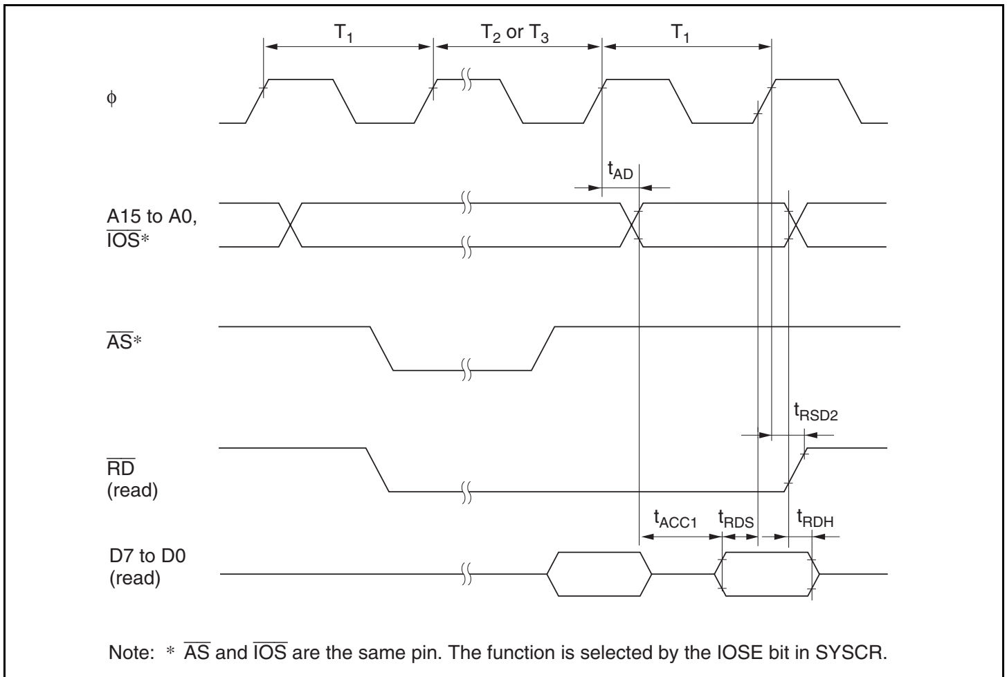
Figure 24.13 Burst ROM Access Timing (One-State Access)
