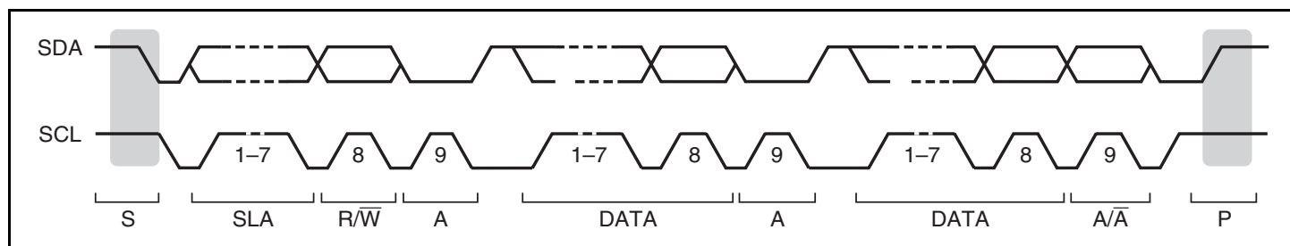
Figure 16.5 I 2 C Bus Timing
