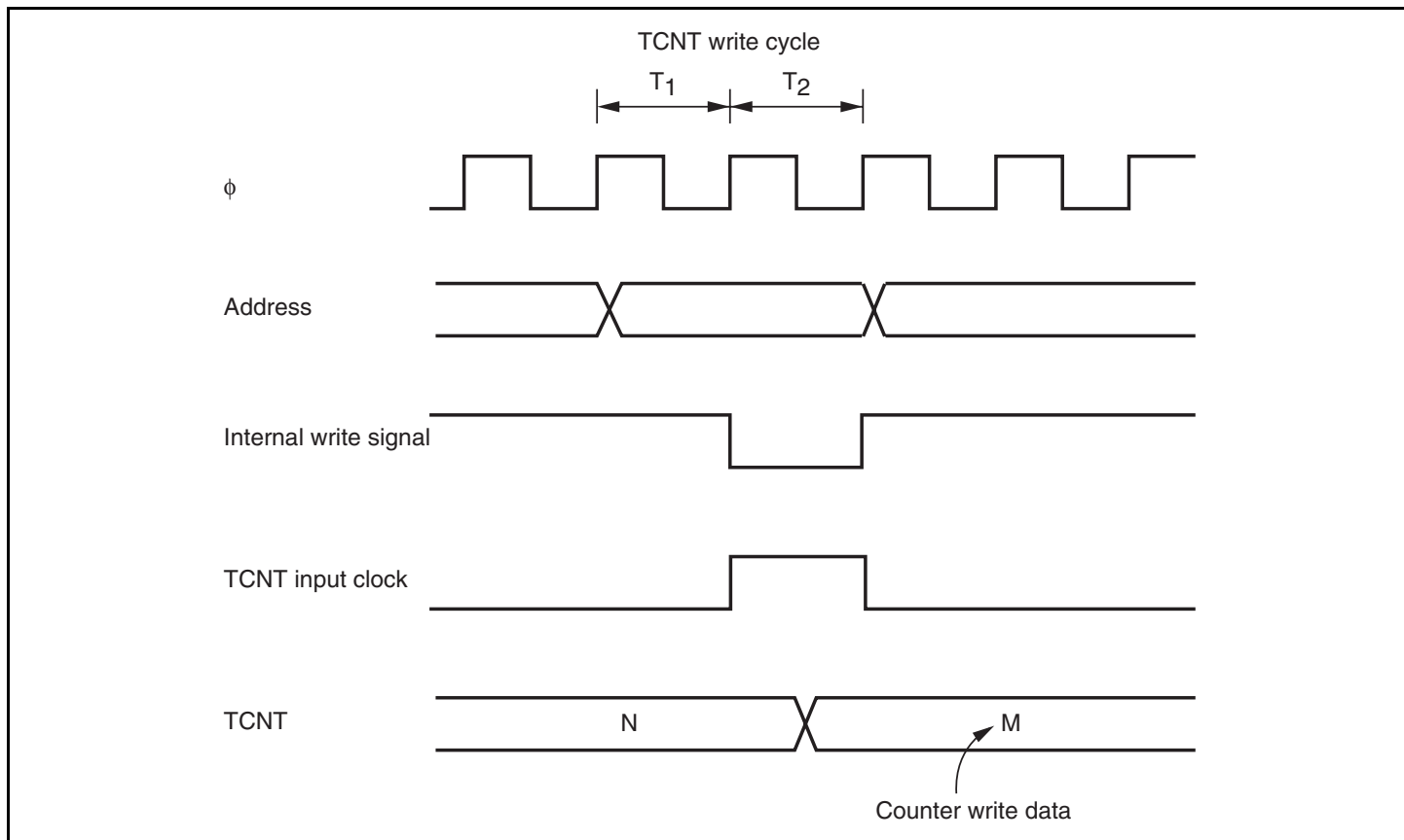
Figure 14.6 Conflict between TCNT Write and Increment
