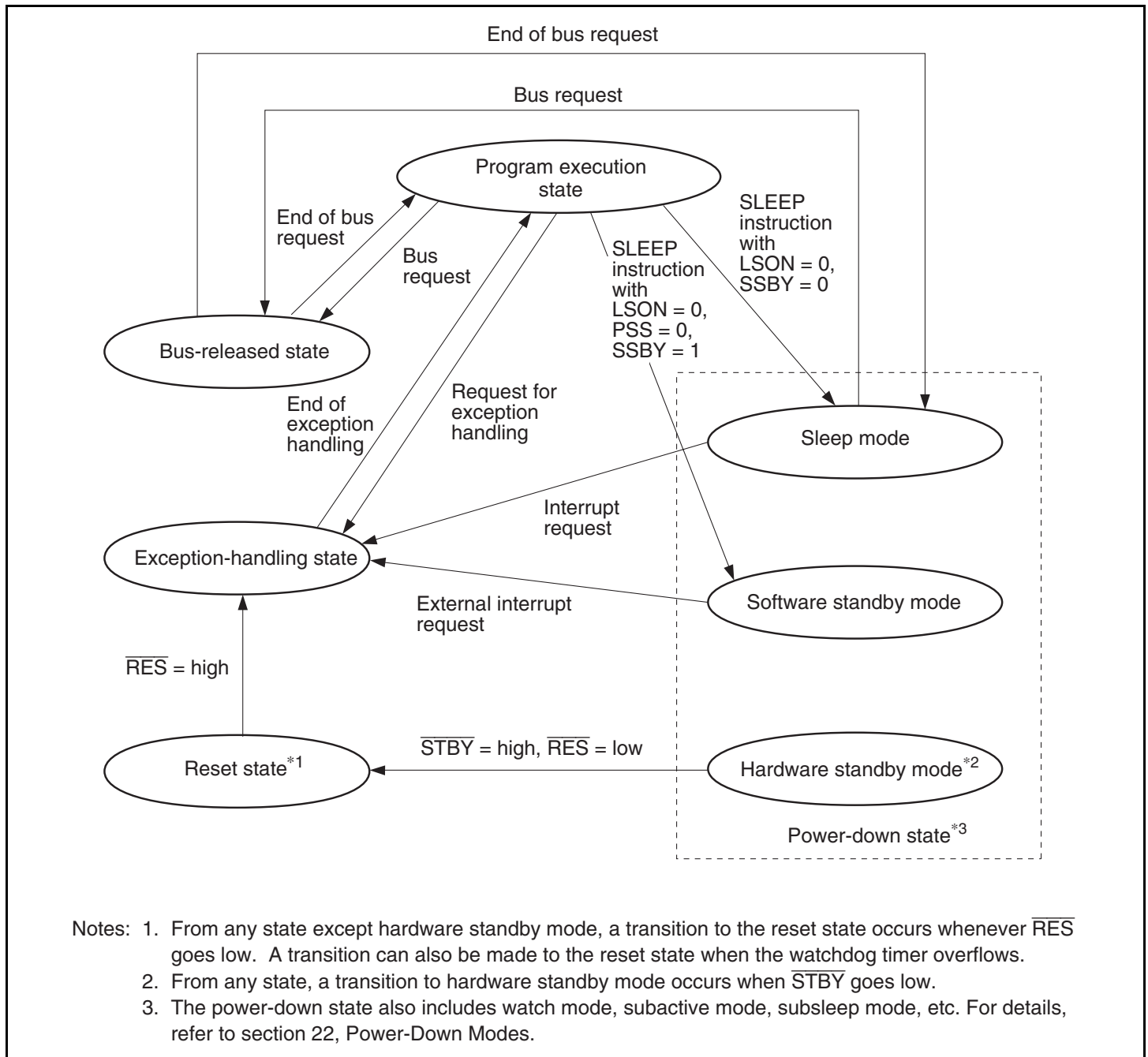
Figure 2.13 State Transitions
