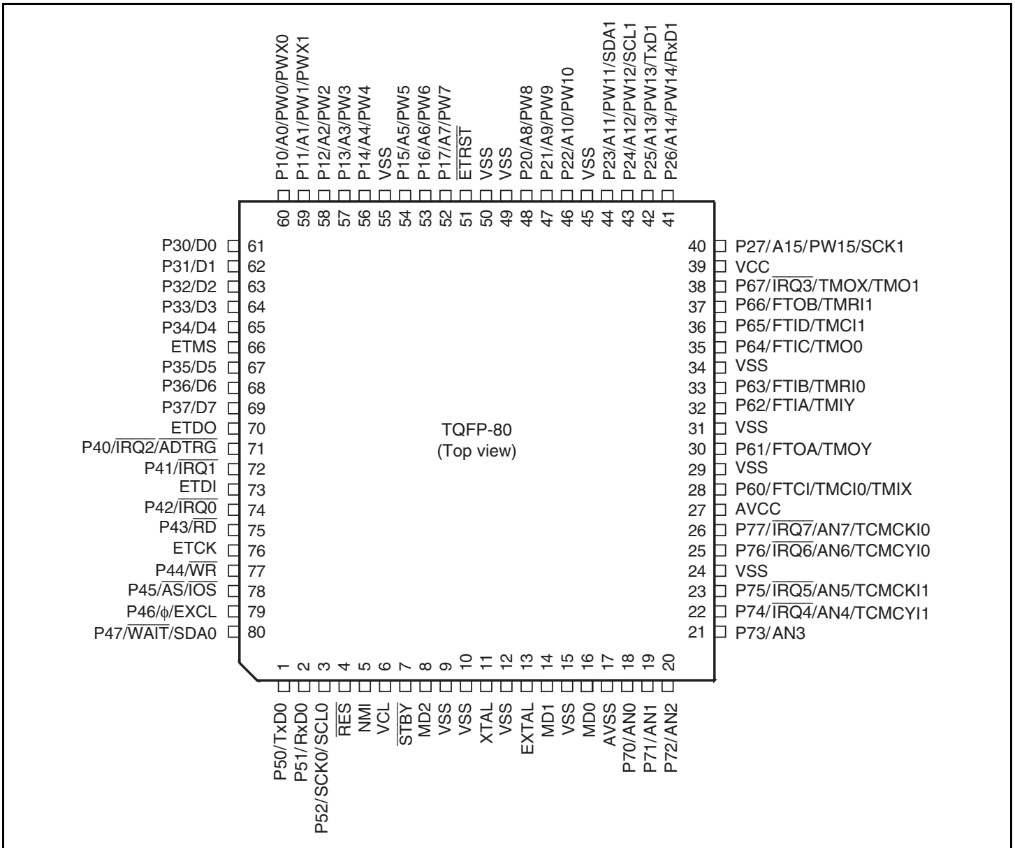
Figure 1.4 Pin Assignments (TQFP-80)
