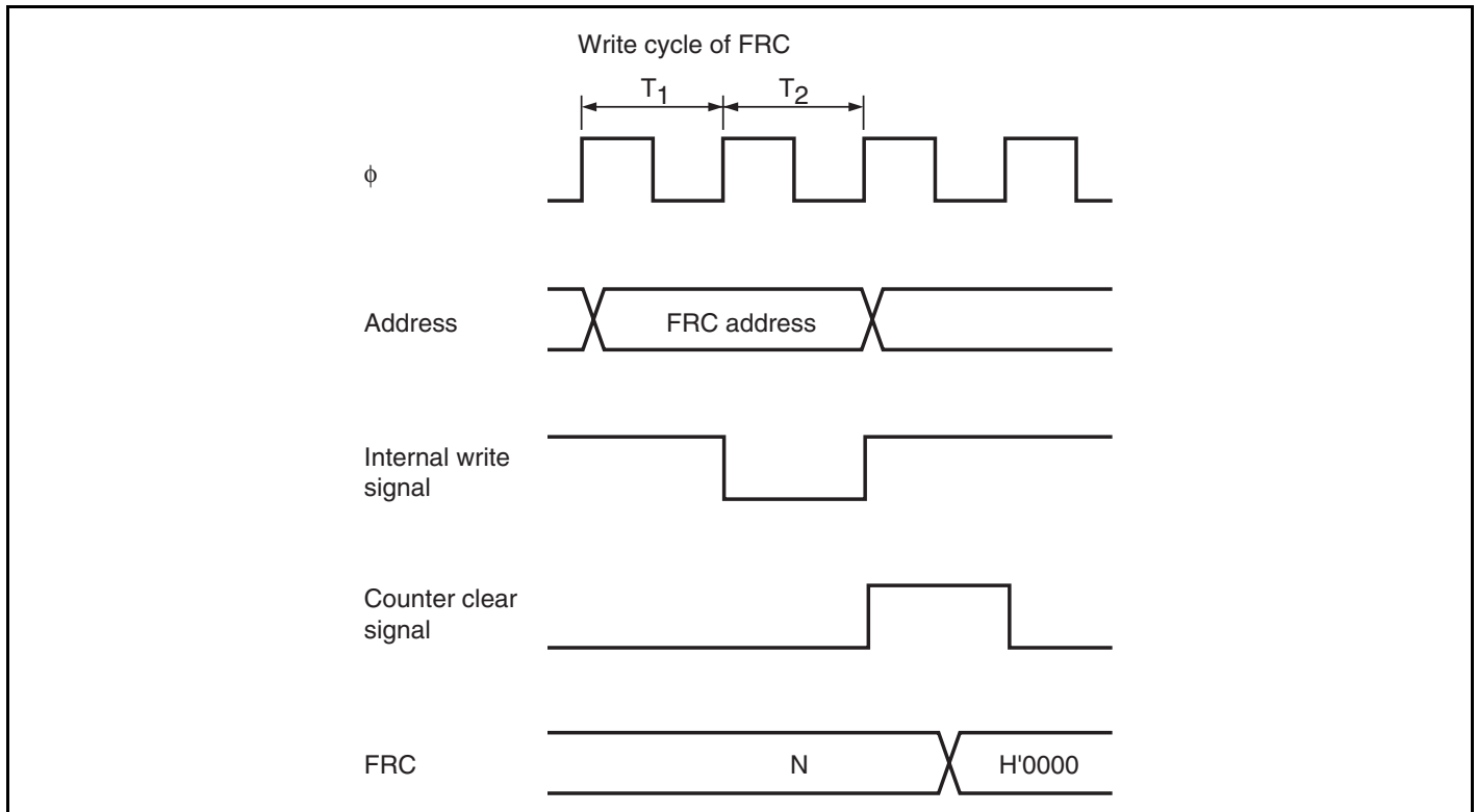
Figure 11.17 Conflict between FRC Write and Clear
