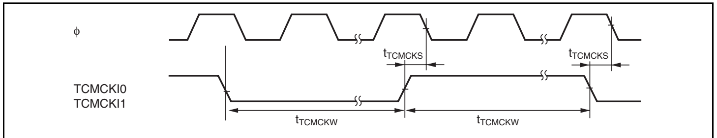
Figure 24.18 TCM Clock Input Timing
