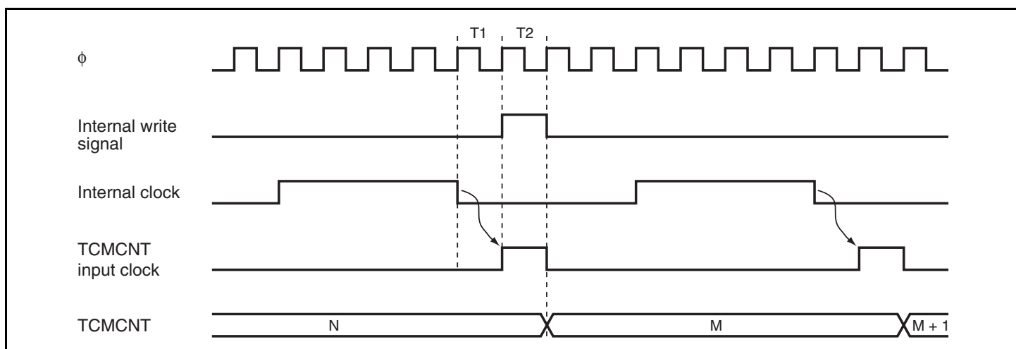
Figure 12.12 Conflict between TCMCNT Write and Count-Up Operation
