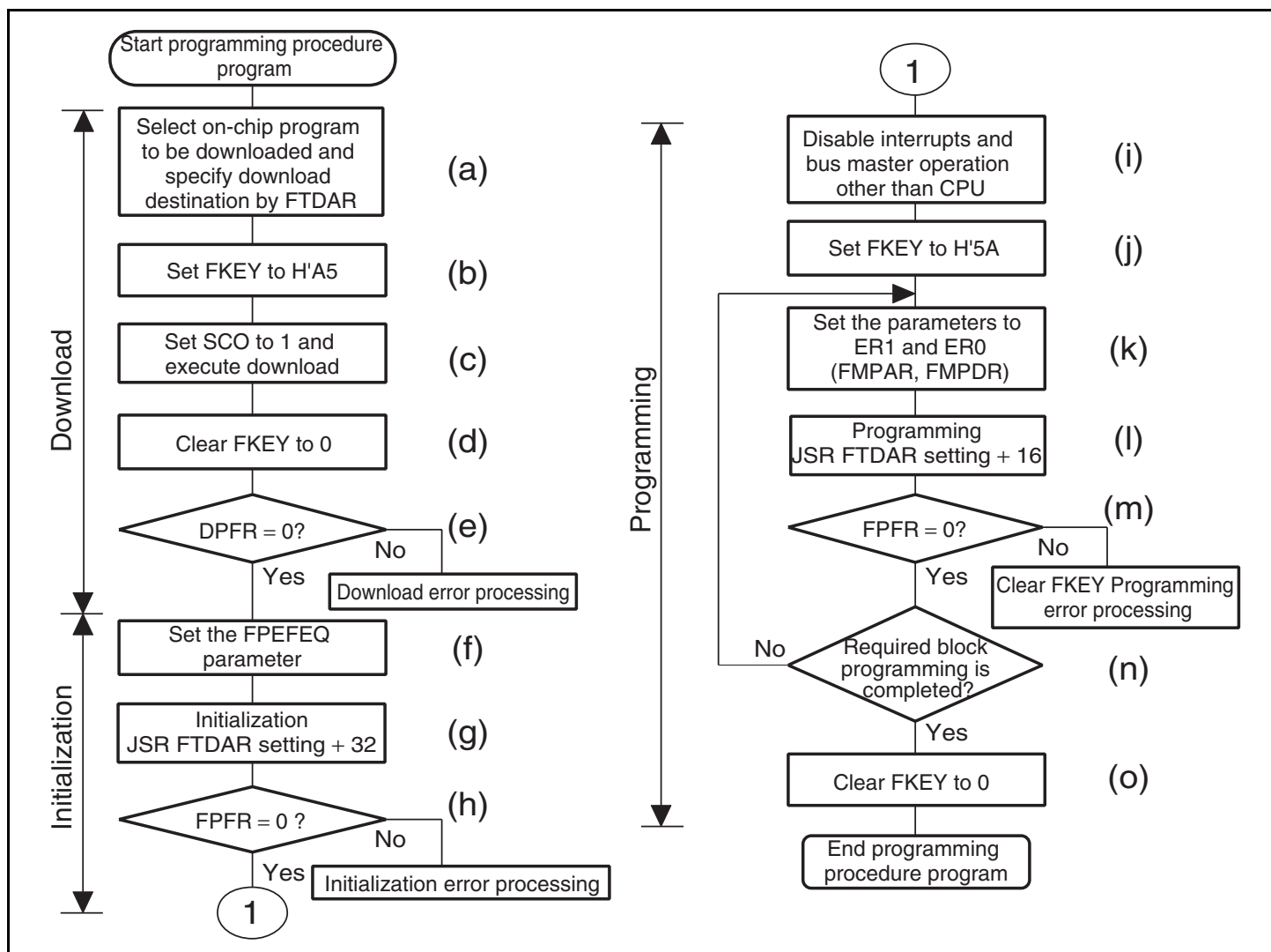
Figure 19.11 Programming Procedure
