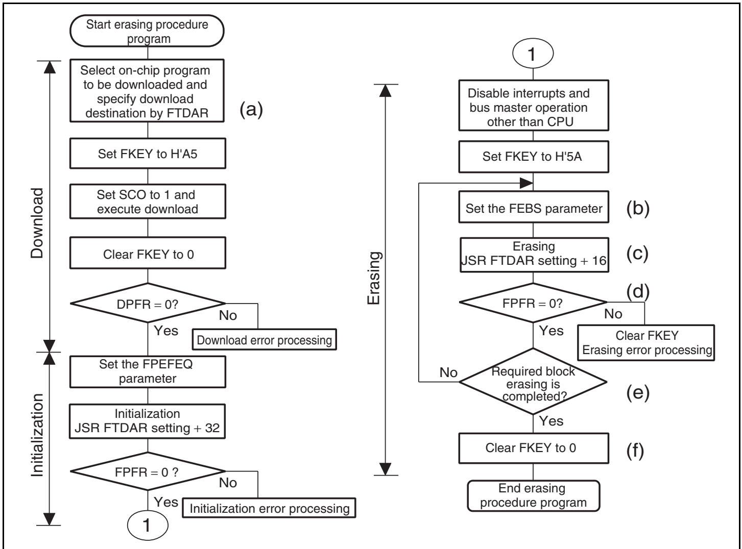
Figure 19.12 Erasing Procedure
