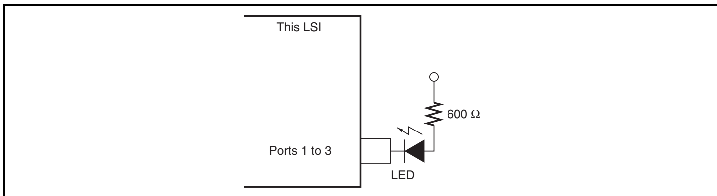
Figure 24.2 LED Drive Circuit (Example)
