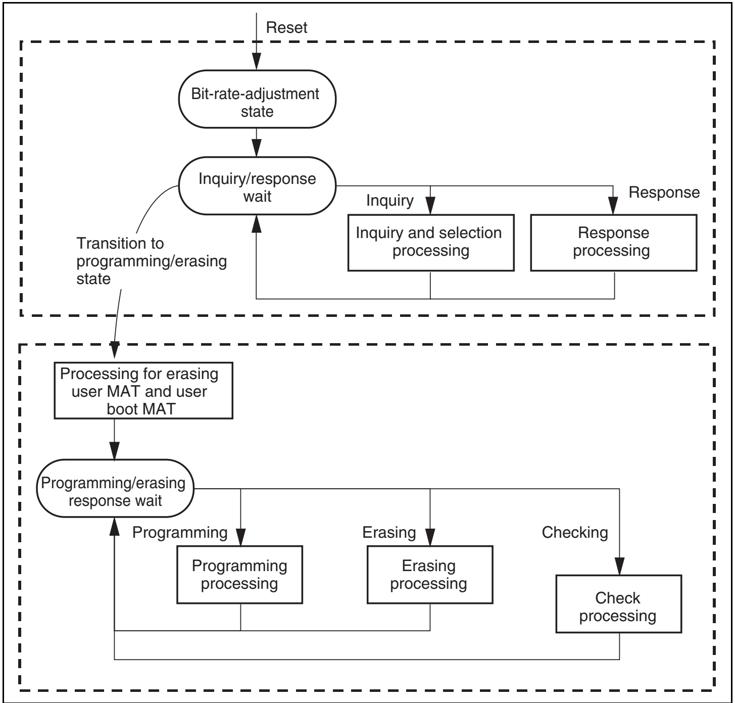
Figure 19.19 Boot Program States
