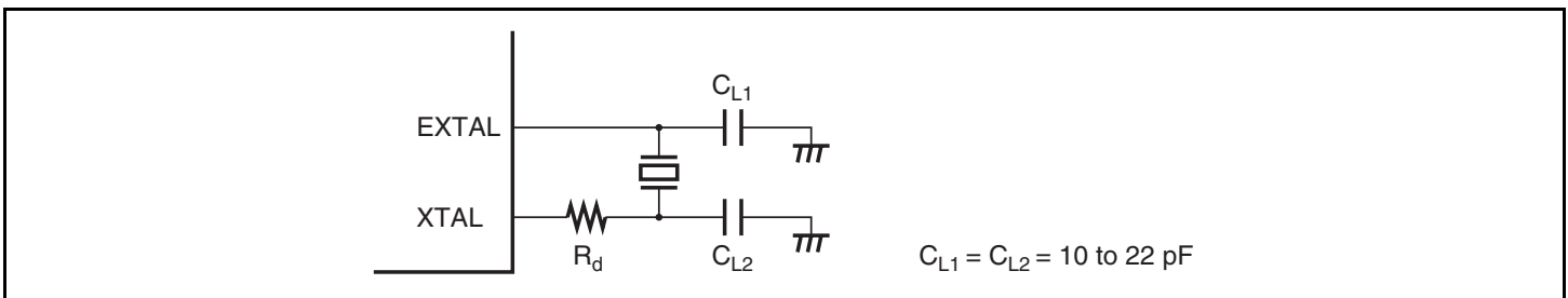
Figure 21.2 Typical Connection to Crystal Resonator
