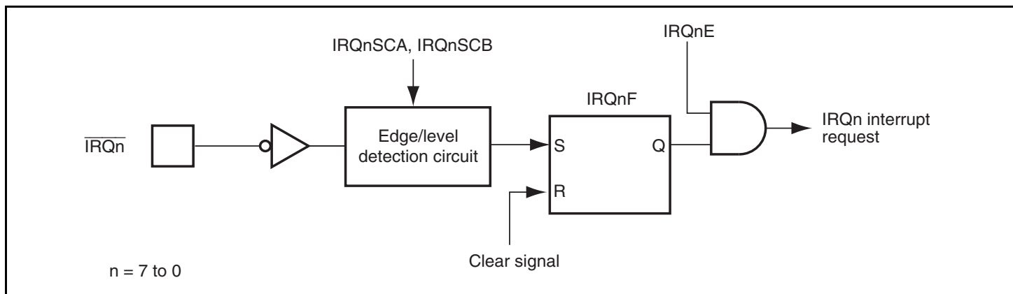
Figure 5.2 Block Diagram of Interrupts IRQ7 to IRQ0
