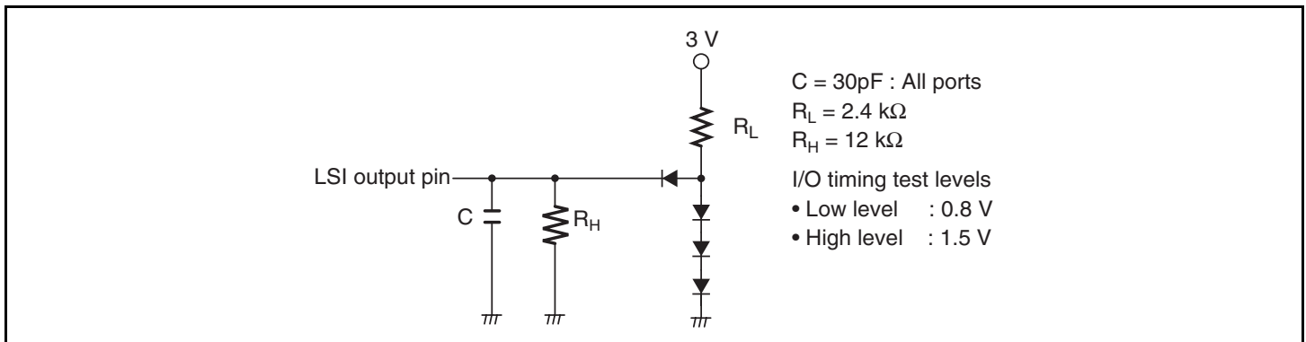
Figure 24.3 Output Load Circuit
