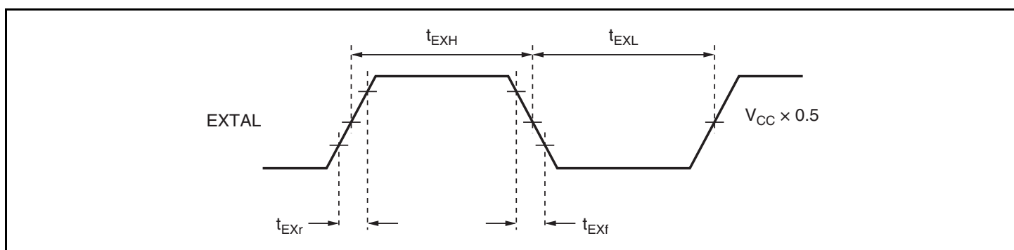
Figure 21.5 External Clock Input Timing
