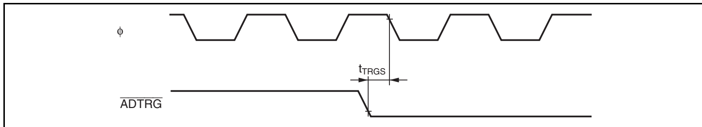
Figure 24.25 A/D Converter External Trigger Input Timing
