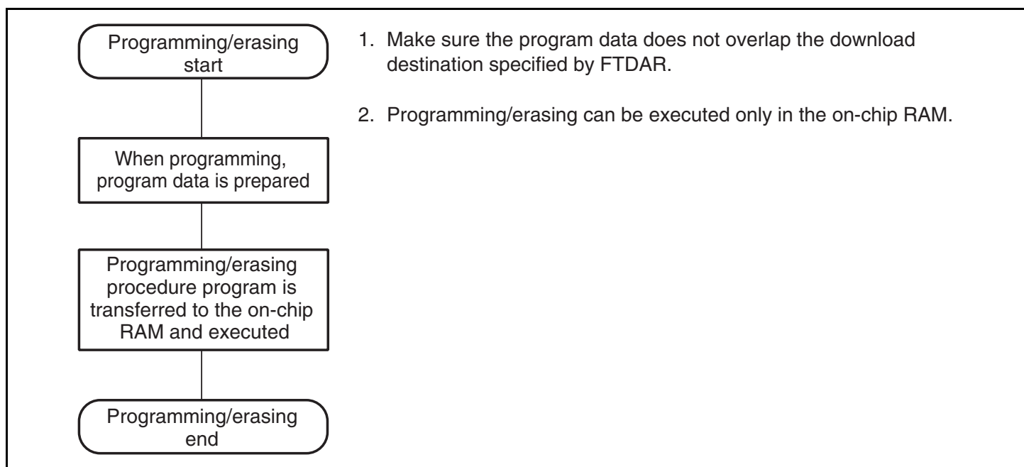
Figure 19.9 Programming/Erasing Overview Flow
