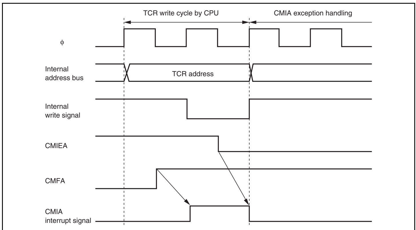
Figure 5.11 Conflict between Interrupt Generation and Disabling
