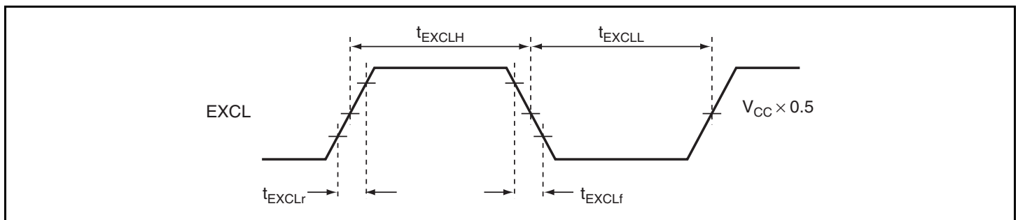
Figure 21.8 Subclock Input Timing
