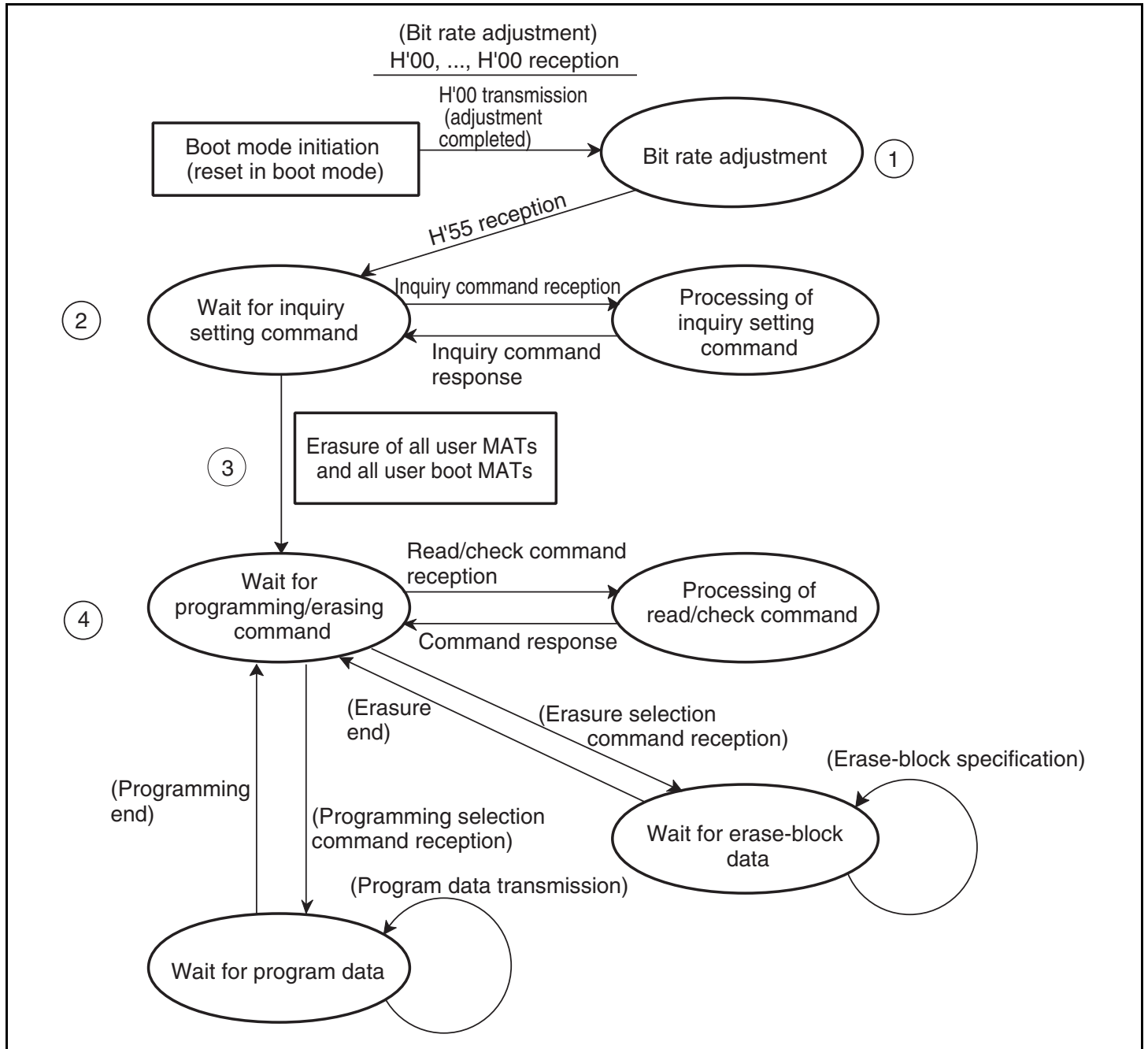
Figure 19.8 Overview of Boot Mode State Transition Diagram
