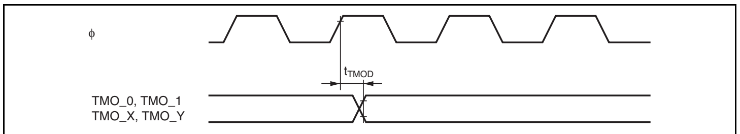
Figure 24.19 8-Bit Timer Output Timing
