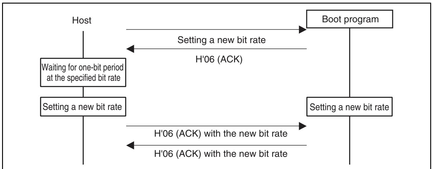
Figure 19.22 Sequence of New Bit Rate Selection
