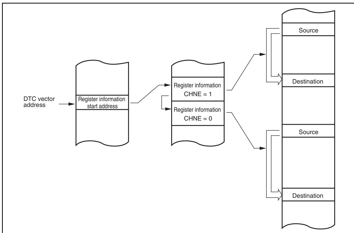
Figure 7.8 Chain Transfer Operation
