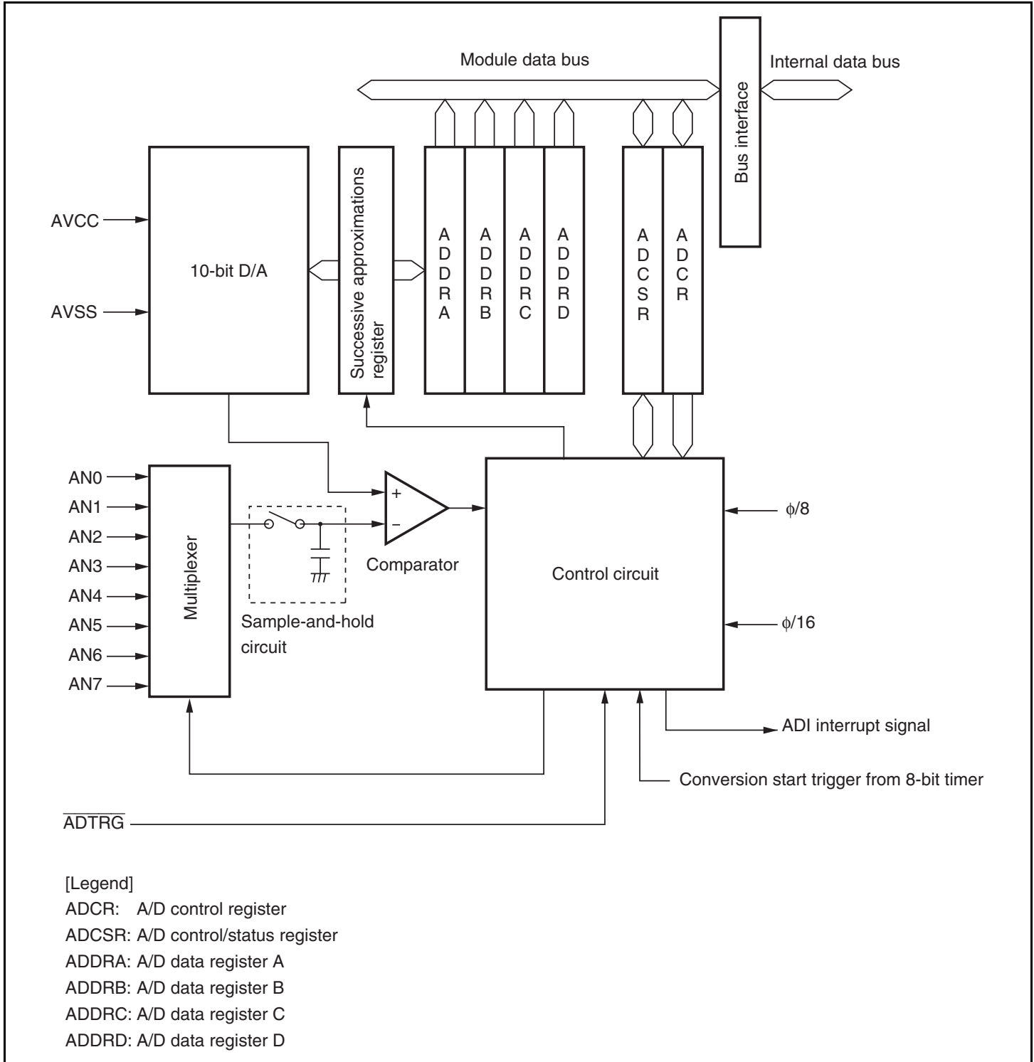
Figure 17.1 Block Diagram of A/D Converter
