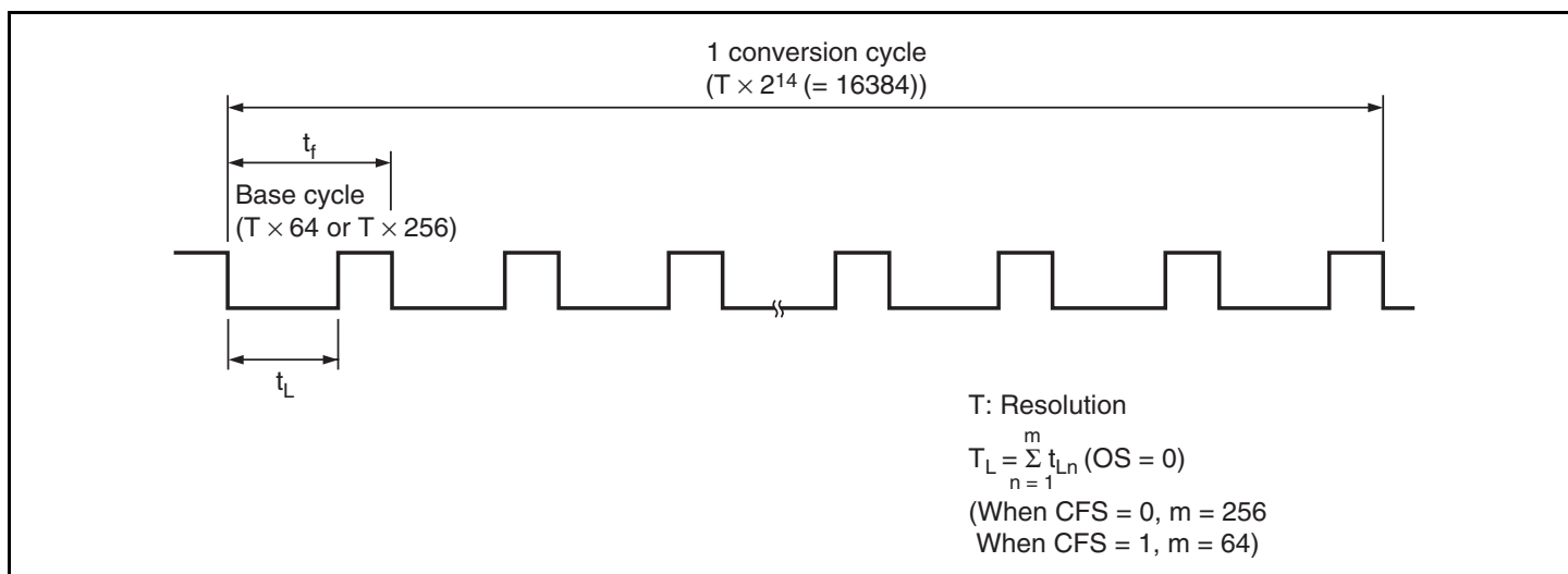
Figure 10.3 PWMX (D/A) Operation
