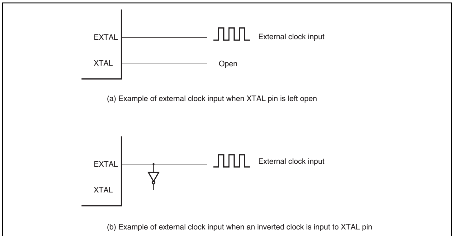
Figure 21.4 Example of External Clock Input
