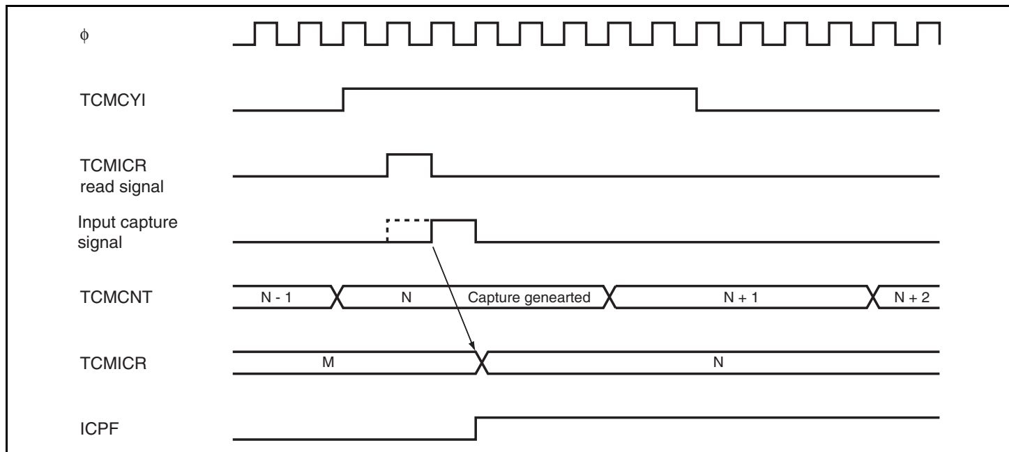
Figure 12.14 Conflict between TCMICR Read and Input Capture
