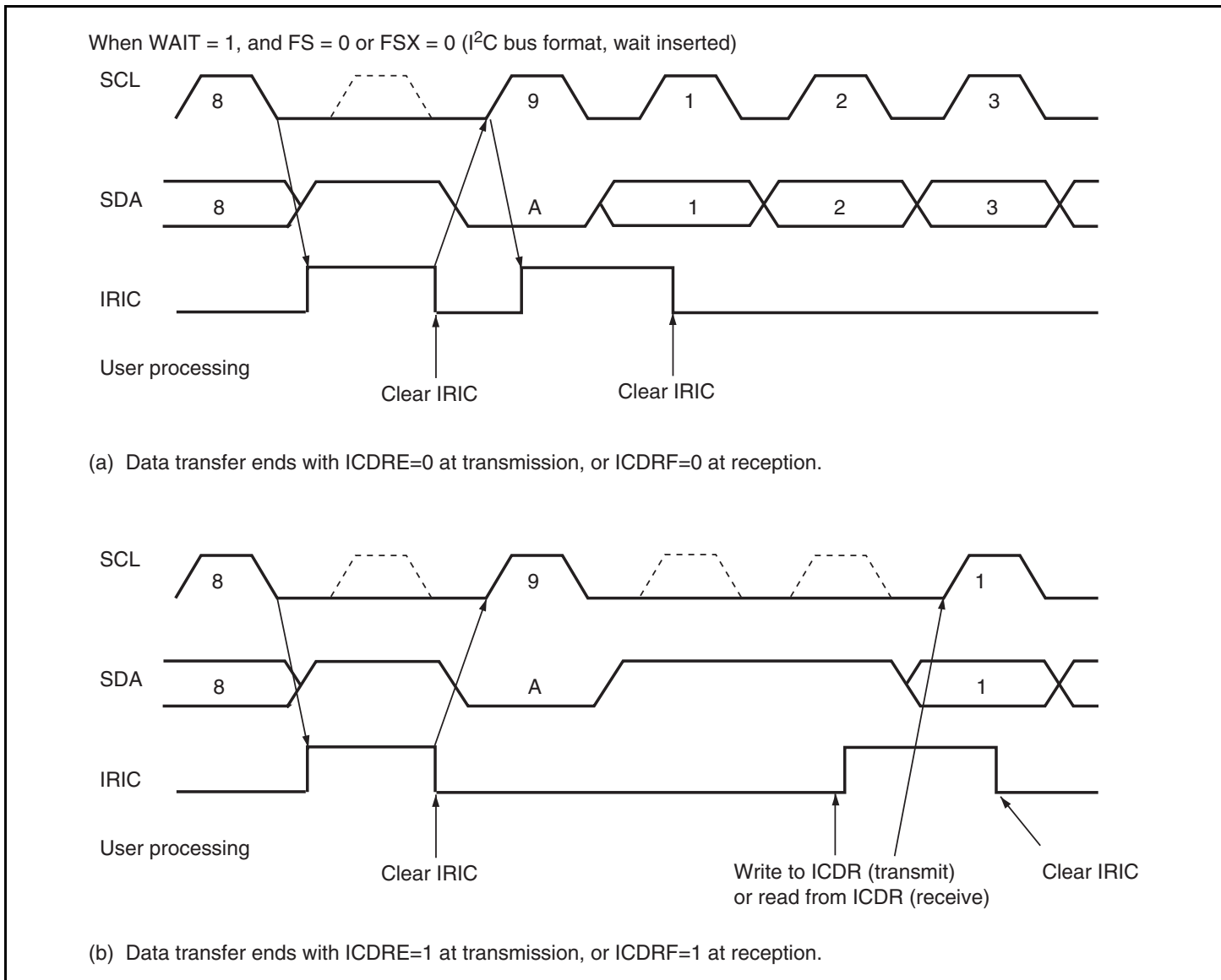
Figure 16.26 IRIC Setting Timing and SCL Control (2)
