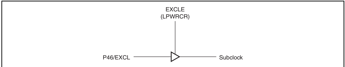
Figure 21.7 Subclock Input from EXCL Pin
