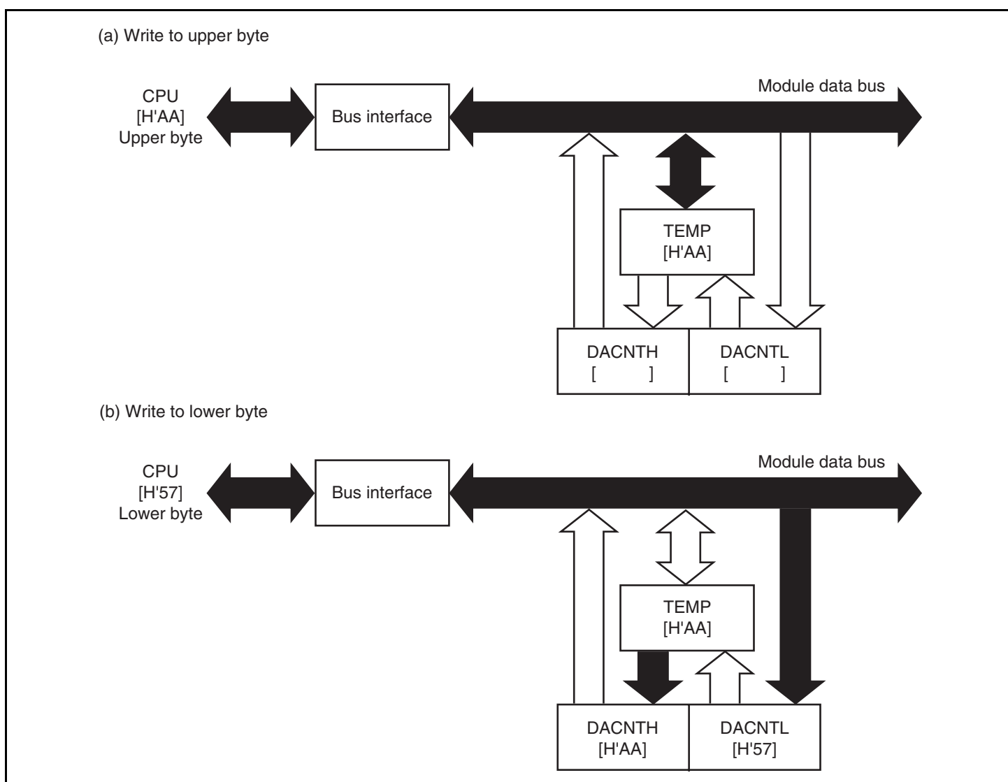
Figure 10.2 (1) DACNT Access Operation (1) [CPU → DACNT(H'AA57) Writing]
