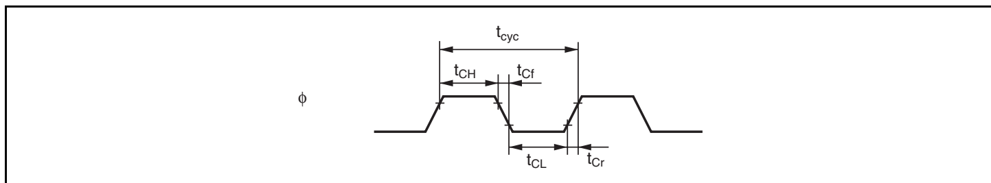
Figure 24.4 System Clock Timing
