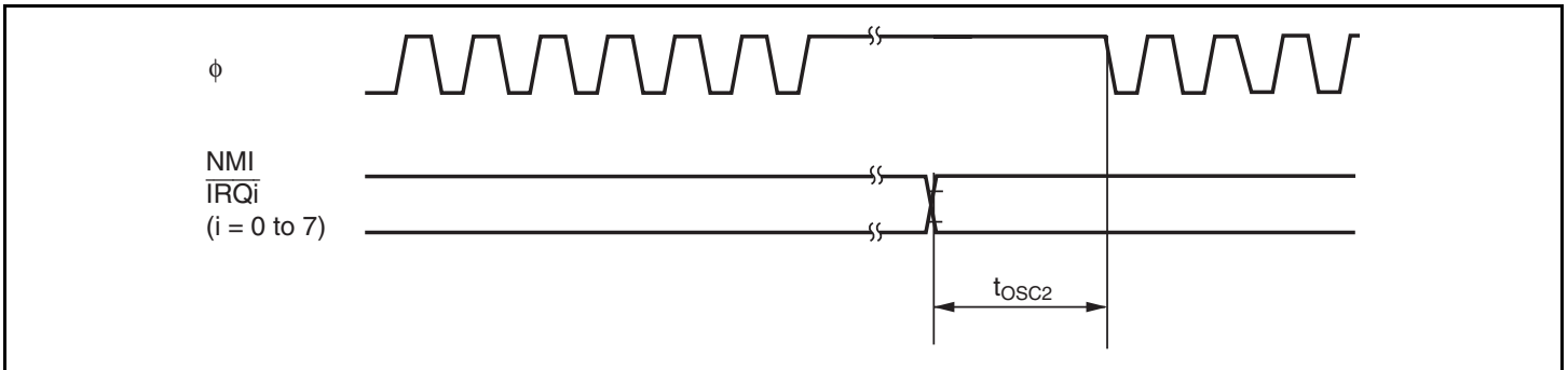
Figure 24.6 Oscillation Stabilization Timing (Exiting Software Standby Mode)
