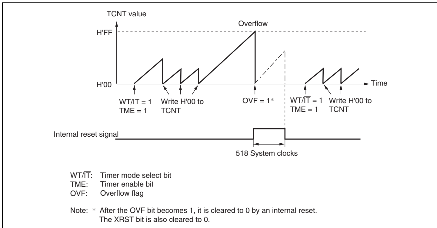
Figure 14.2 Watchdog Timer Mode (RST/NMI = 1) Operation
