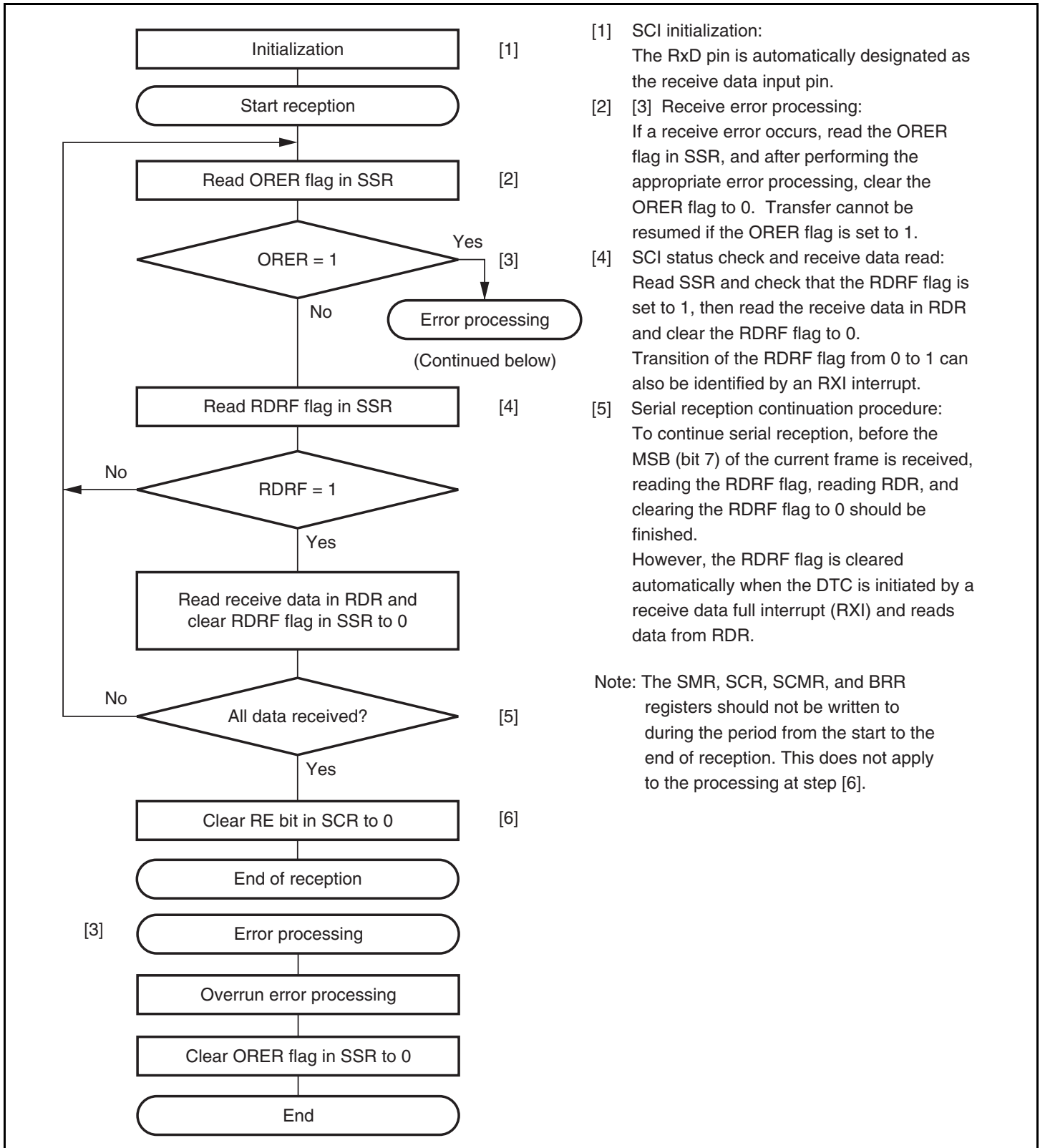
Figure 15.19 Sample Serial Reception Flowchart
