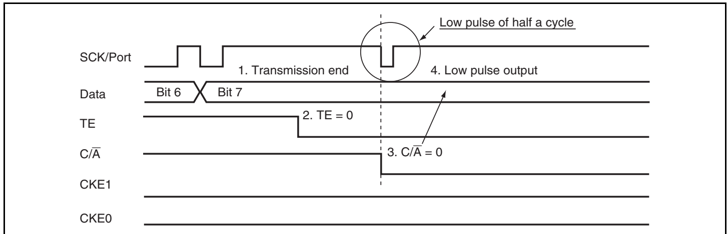
Figure 15.26 Switching from SCK Pins to Port Pins
