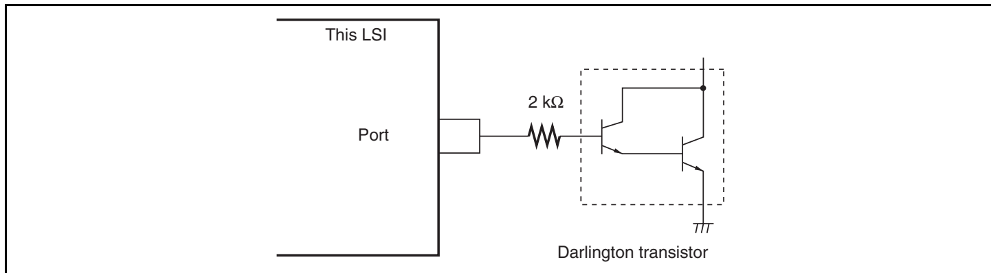
Figure 24.1 Darlington Transistor Drive Circuit (Example)
