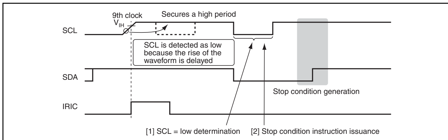
Figure 16.31 Stop Condition Issuance Timing
