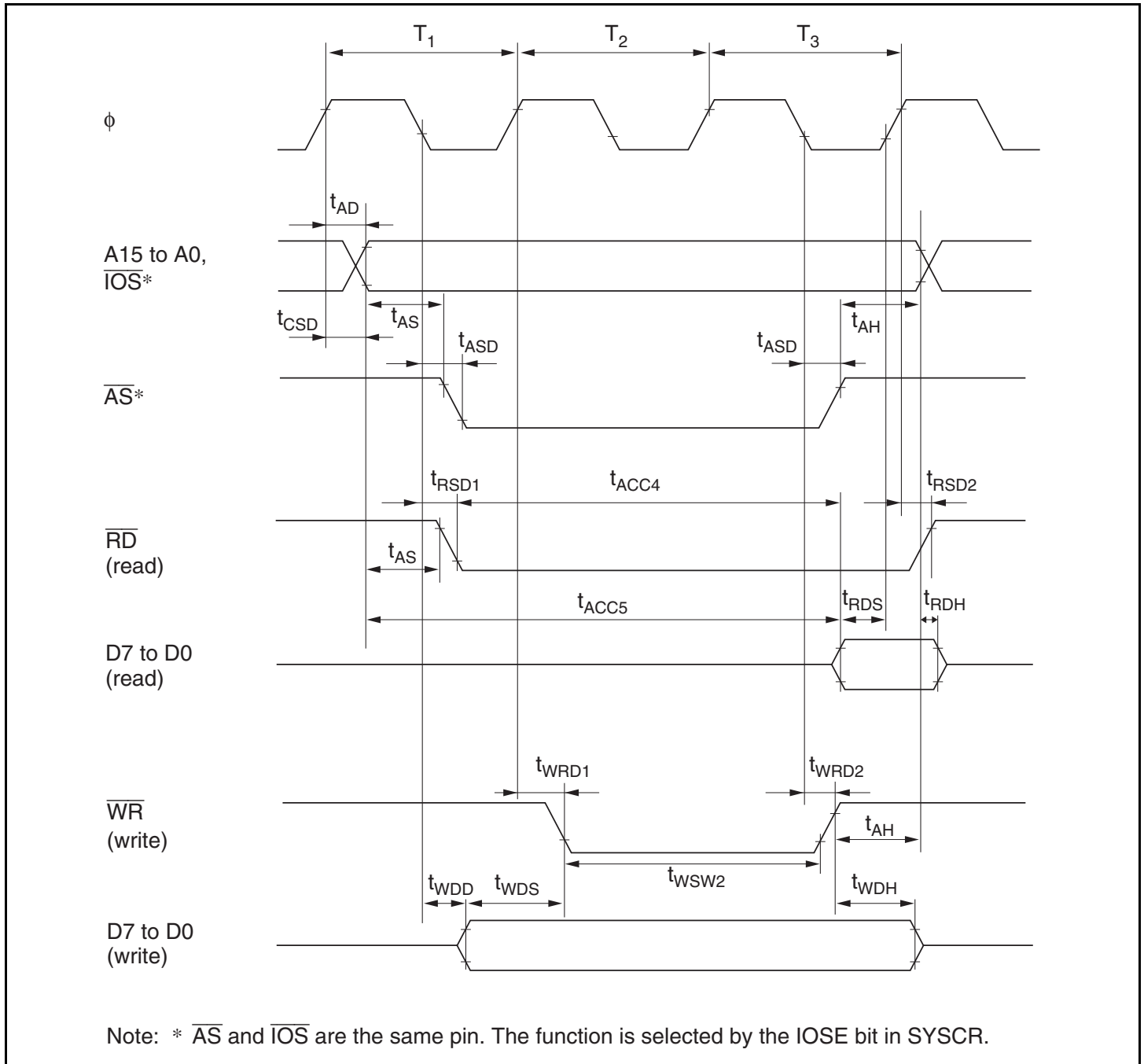
Figure 24.10 Basic Bus Timing (Three-State Access)
