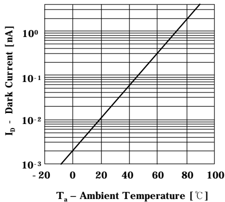
Fig.3 Dark current vs. Ambient temperature
