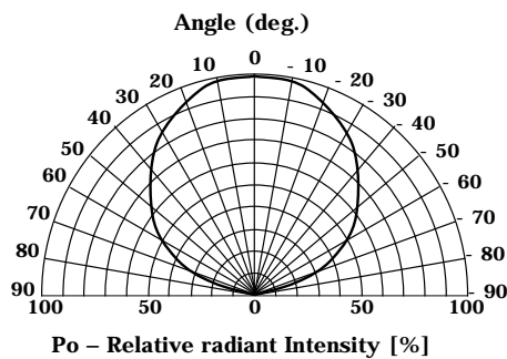
Fig.5 Radiant Pattern
